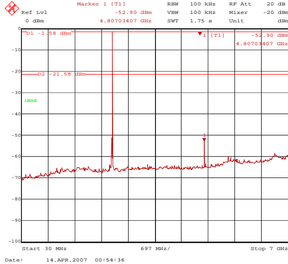
Figure 8: Spurious RF conducted emissions
