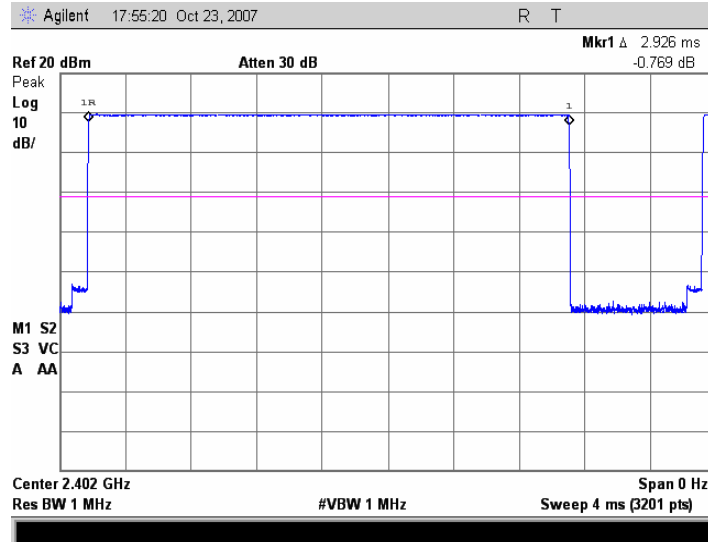
Figure 5. Plot of the Time of Occupancy (Conducted)
