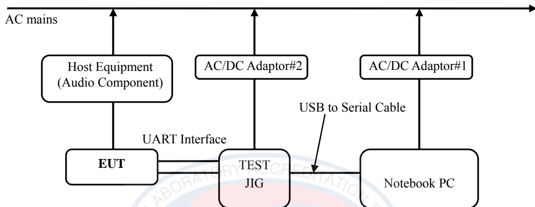
[ System Block Diagram of Test Configuration ]
