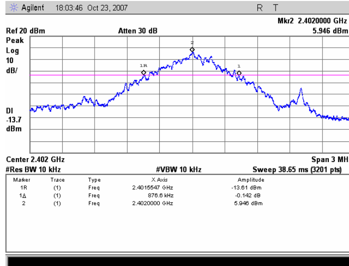
Figure 3. Plot of the 20dB Channel Bandwidth (Conducted)
