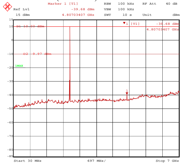
Figure 9: Spurious RF conducted emissions
