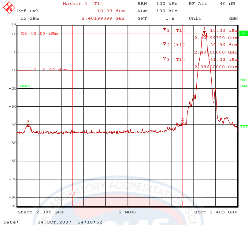
Figure 6. Plot of the Band Edge (Conducted)
