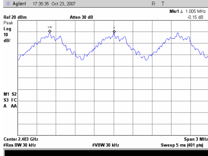
Figure 2. Plot of the Carrier Frequency Separation (Conducted)
