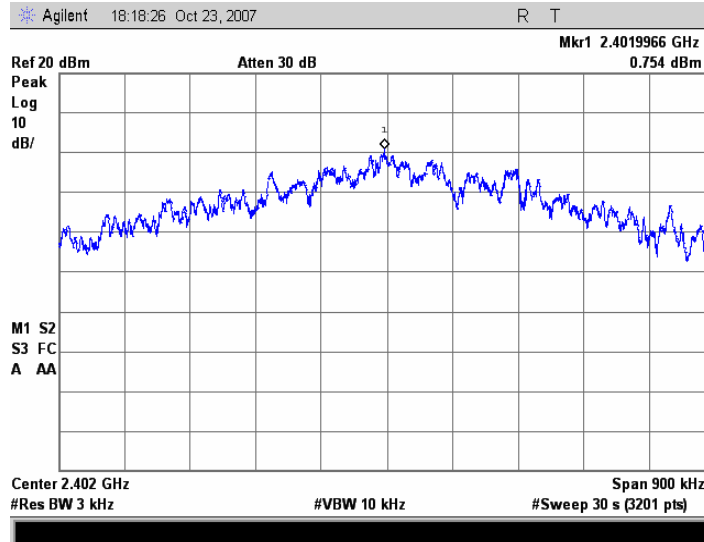
Figure 10. Plot of the Peak Power Spectral Density (Conducted)
