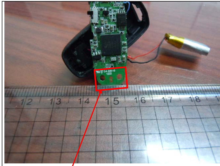
PCB Antenna
