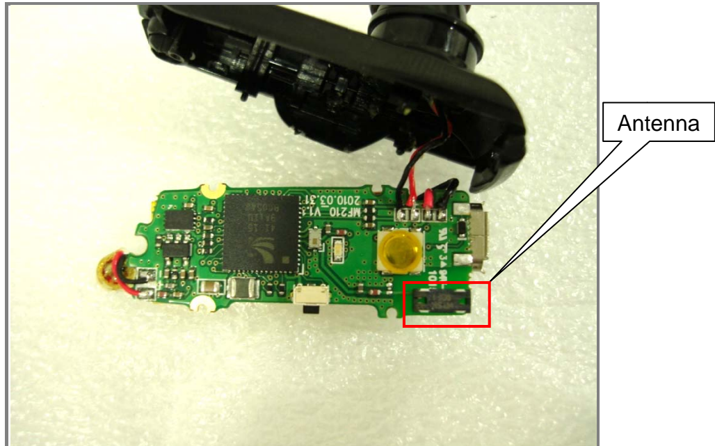
Bottom view of PCB
