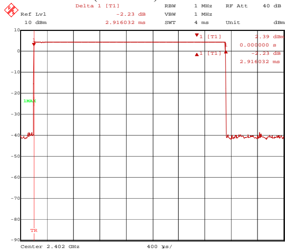
Figure 5. Plot of the Time of Occupancy Basic (GFSK) Lowest Channel (2402 MHz)
