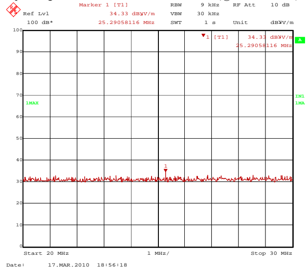
Figure 9. Emission plot for the preliminary radiated measurements
