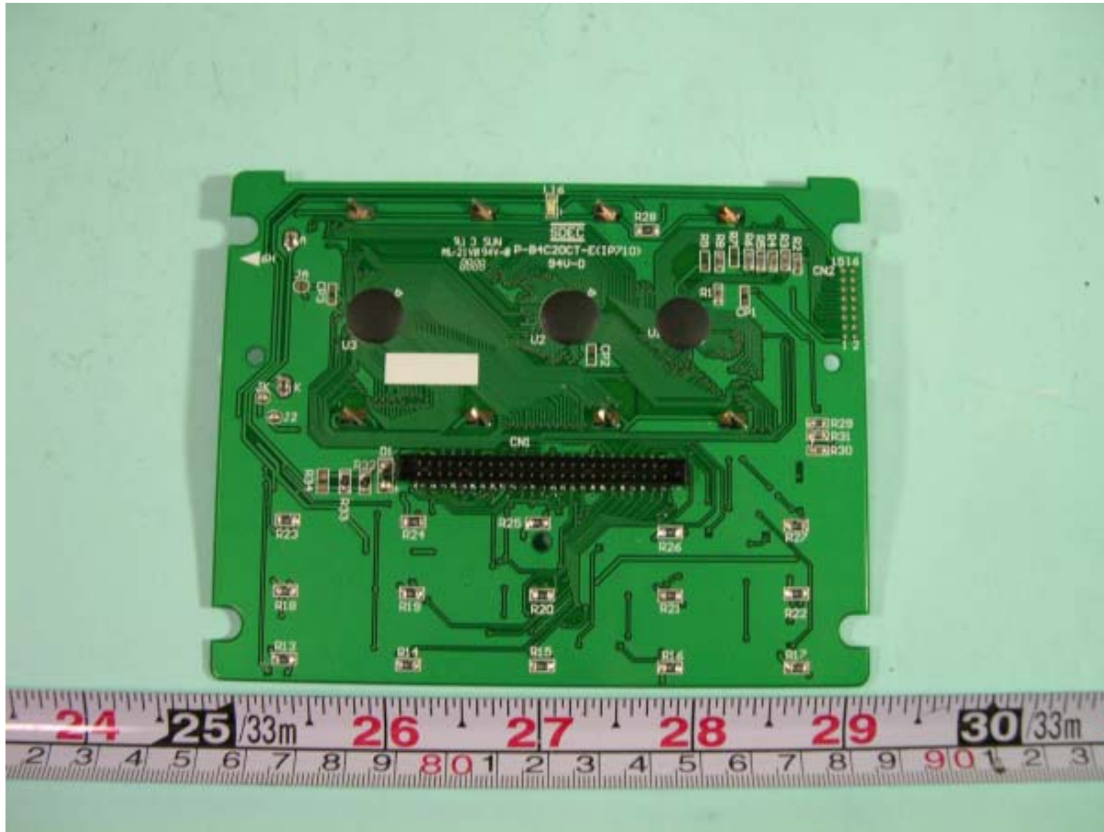
REAR SIDE OF LCD BOARD
