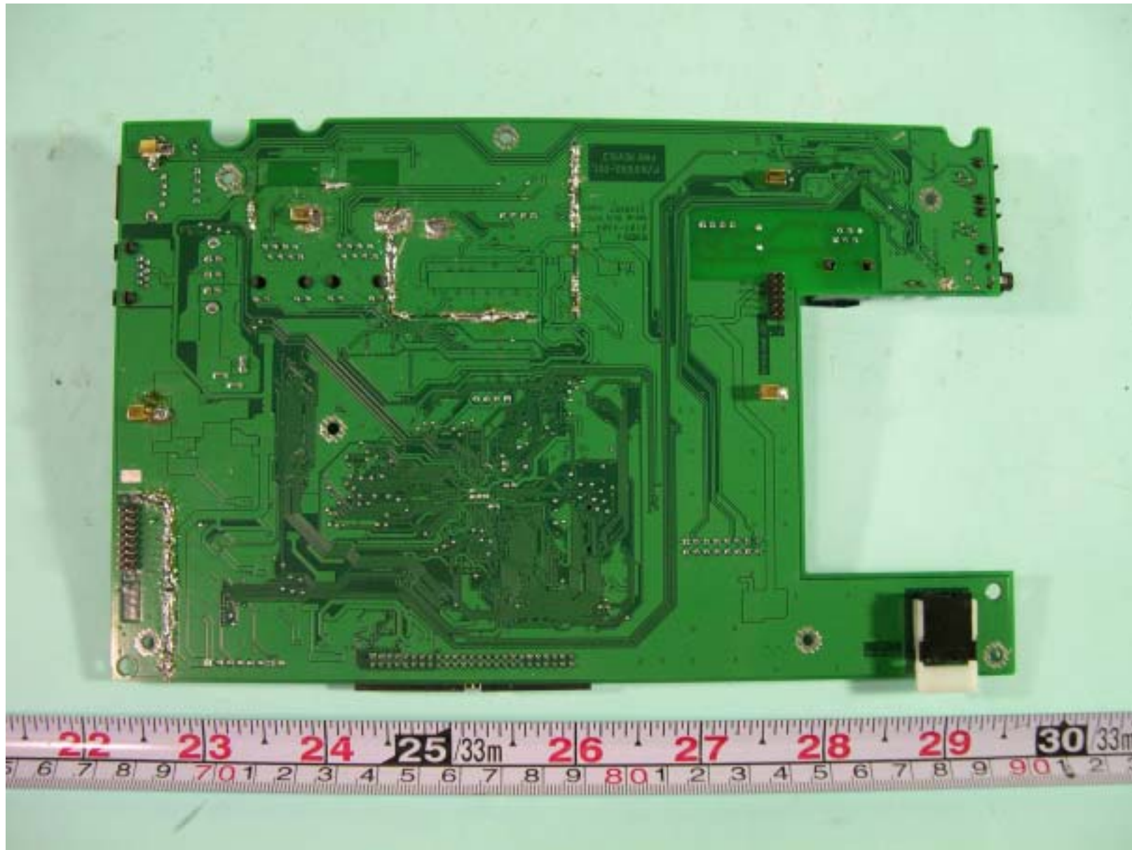
REAR SIDE OF MAIN BOARD
