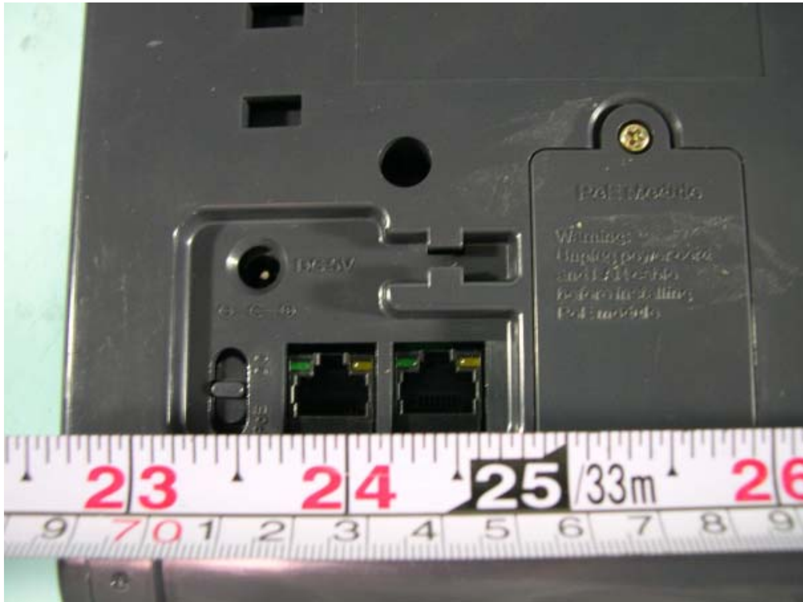
CLOSER LOOK OF REAR INTERFACE PORT
