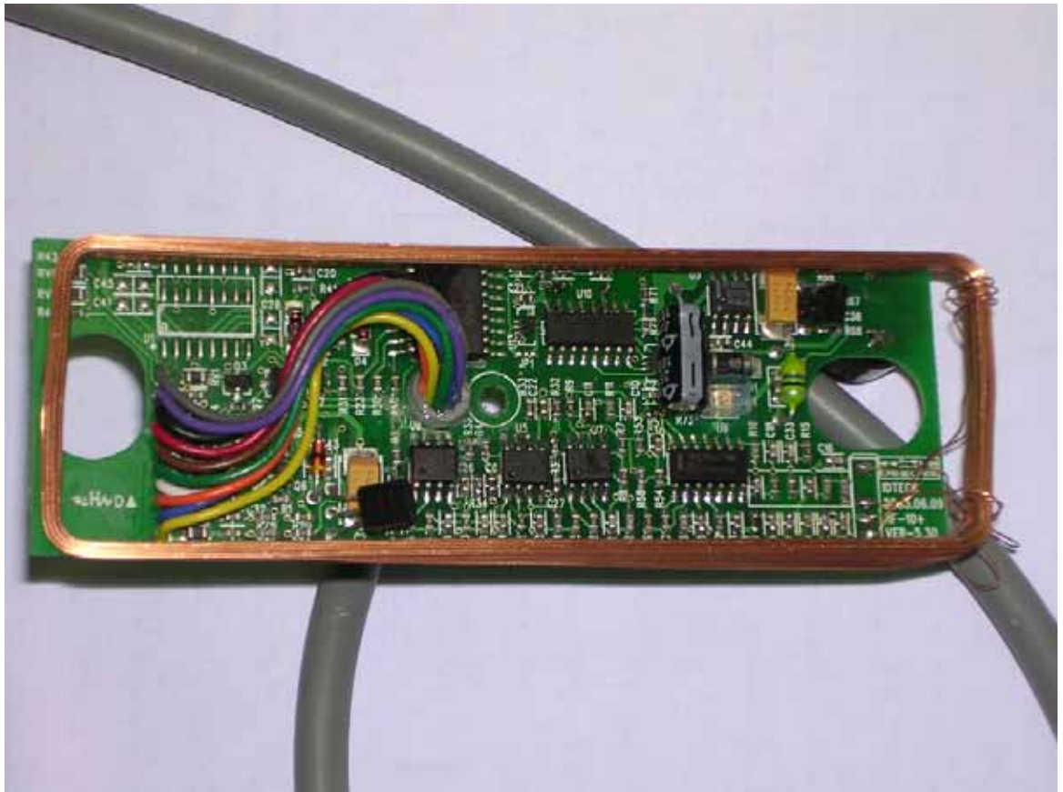
PCB ASS'Y_Top
