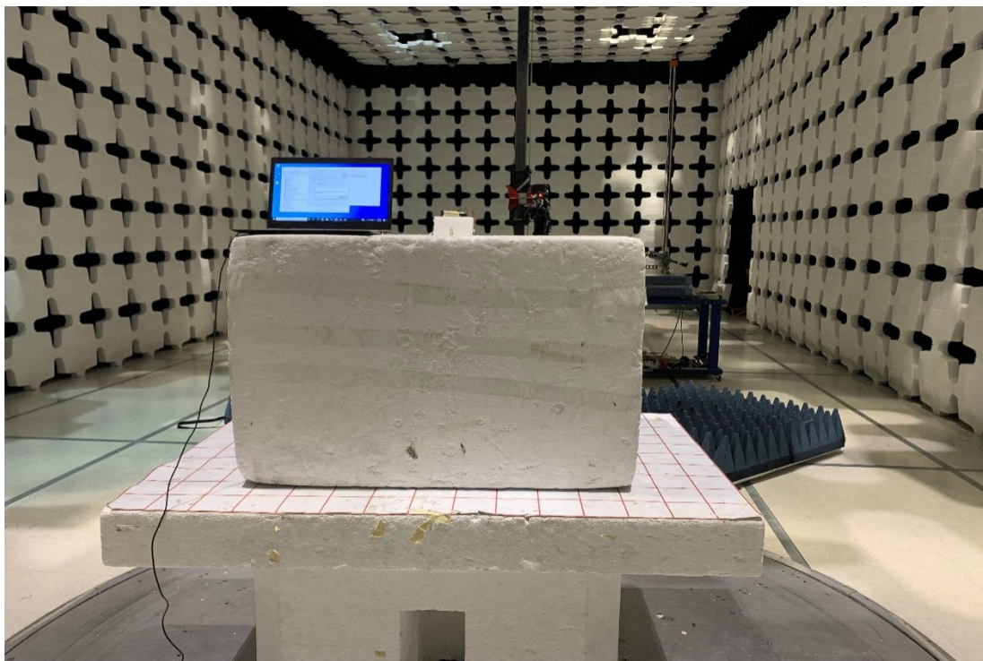
Radiated Emission 1 – 18GHz (Rear View)
