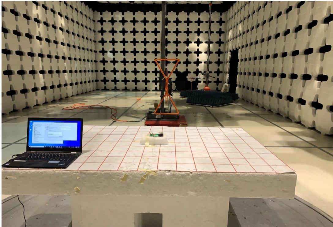
Radiated Emission 30 – 1000MHz (Rear View)
