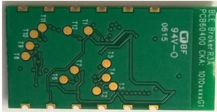
Circuit Board Bottom View
