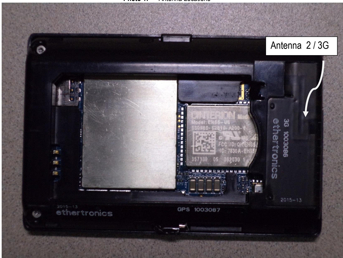
Photo 1: Antenna Locations
