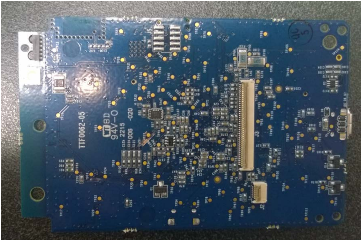
Circuit Board Top Inside View
