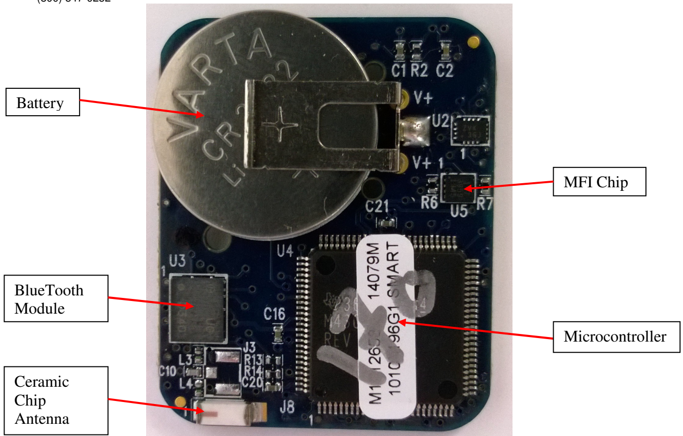
Circuit Board Top View
