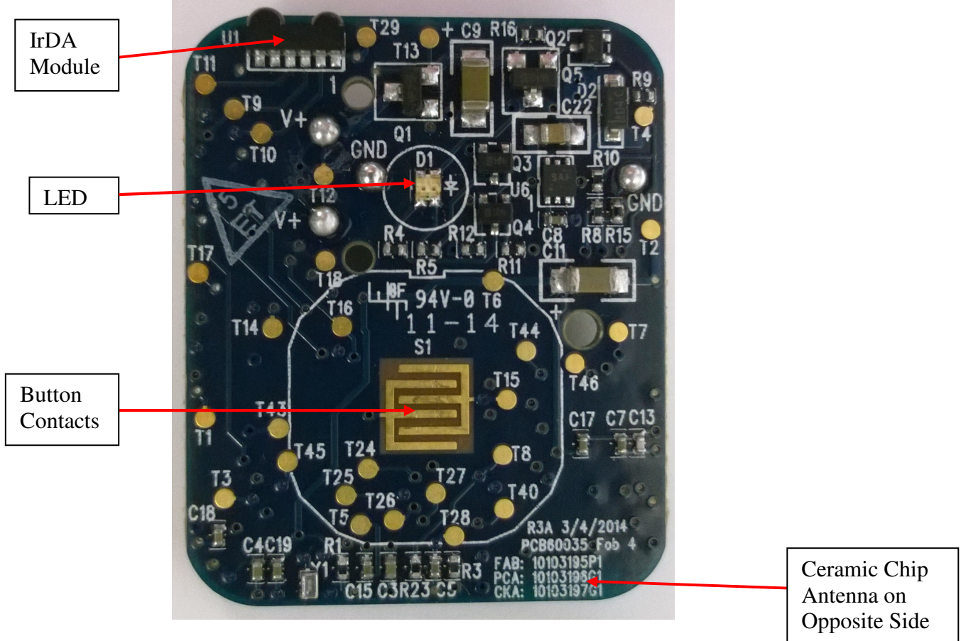
Circuit Board Bottom View
