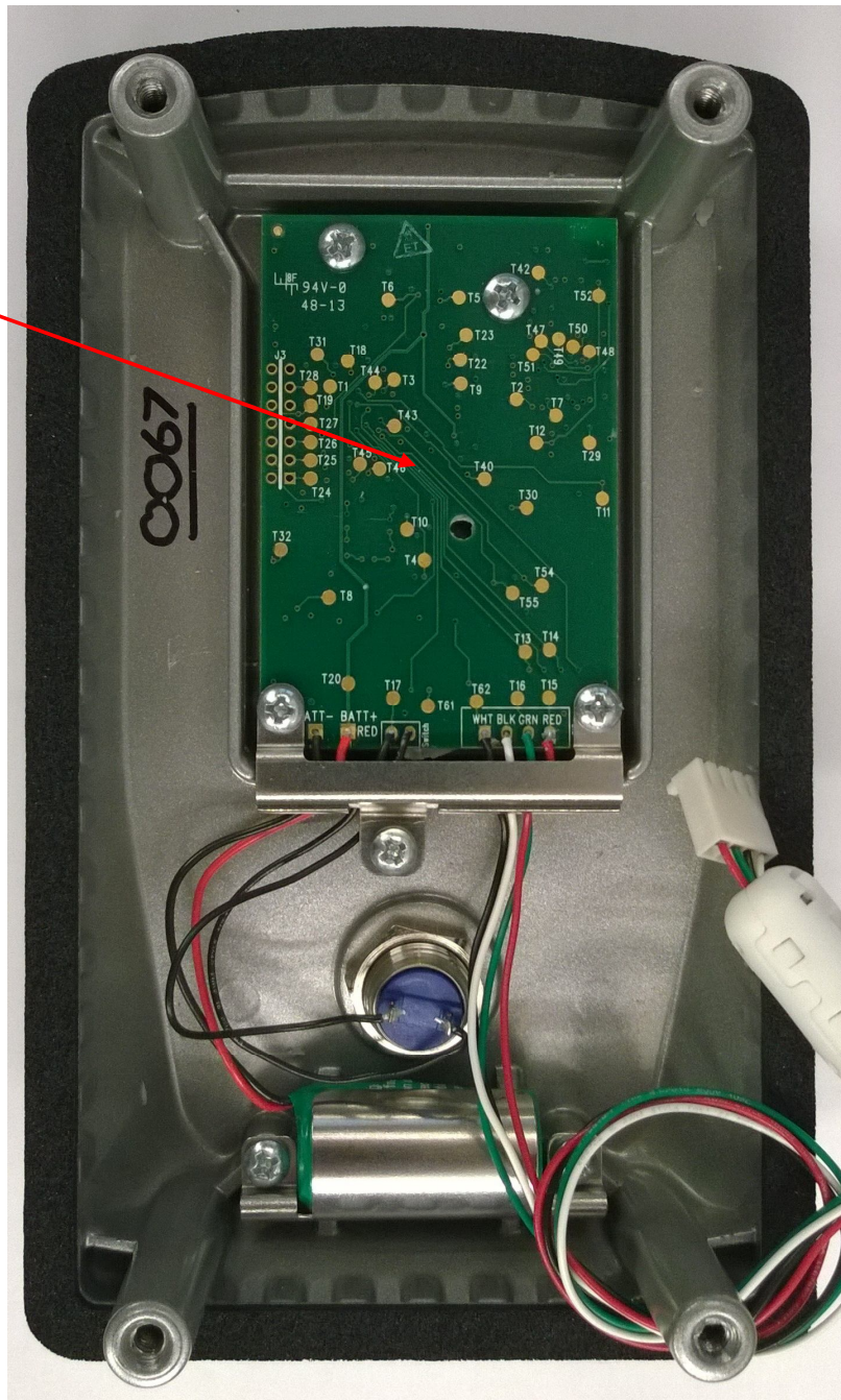
Rear View (Potting Compound Removed)
