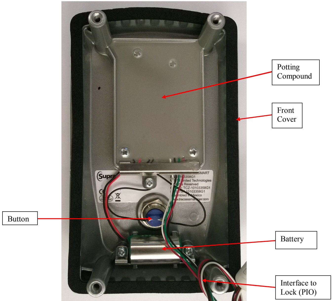
Rear View (with Potting Compound)
