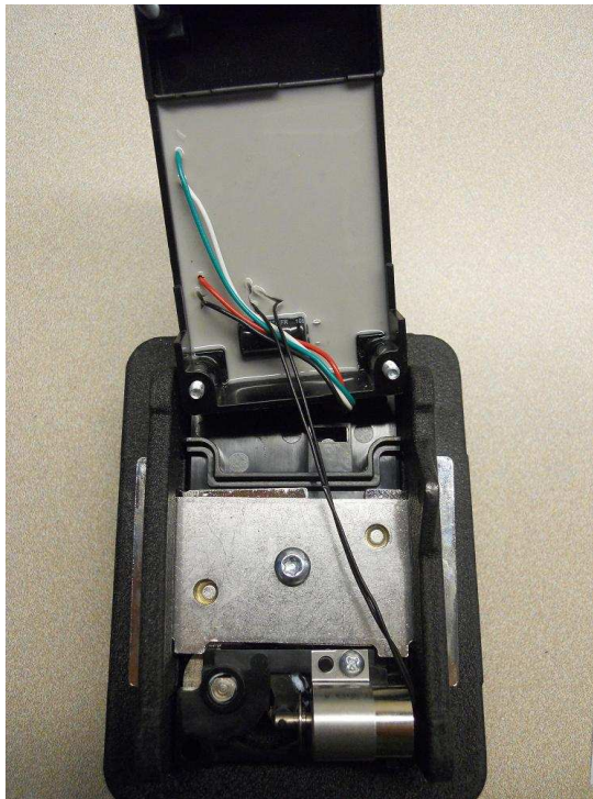
Inside Back Cover – picture shows completed assembly with potting material
