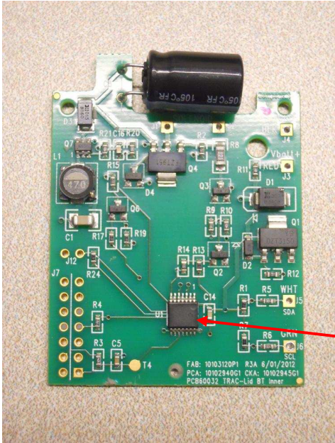
Inner Circuit Board Top View
