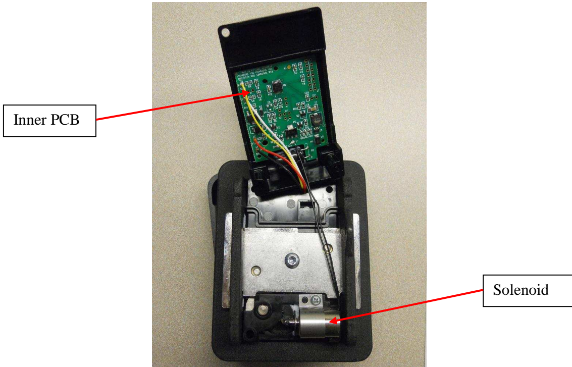
Inside Back Cover – picture shows circuit board without potting material
