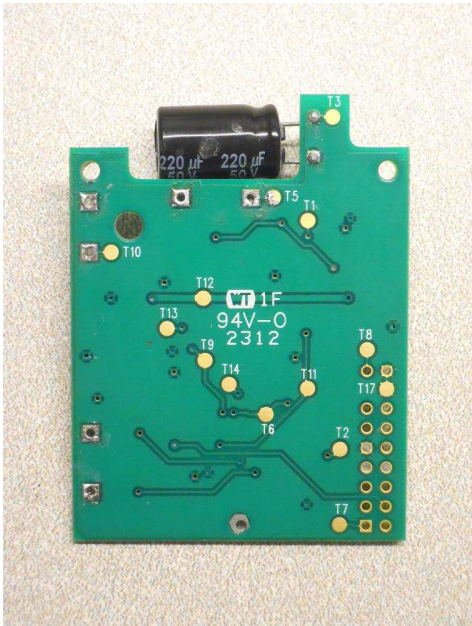
Inner Circuit Board Bottom View
