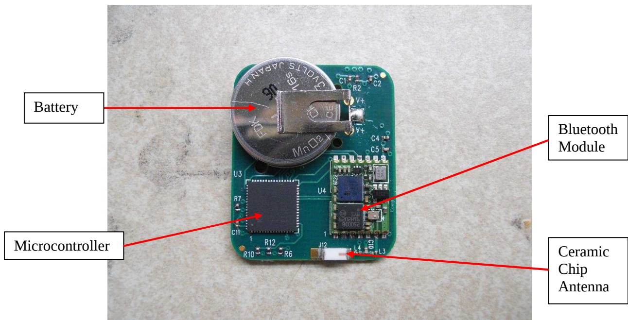
Circuit Board Bottom View
