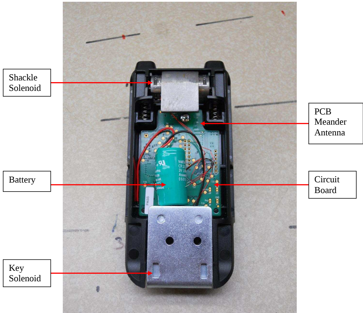
Inside chassis Back View
