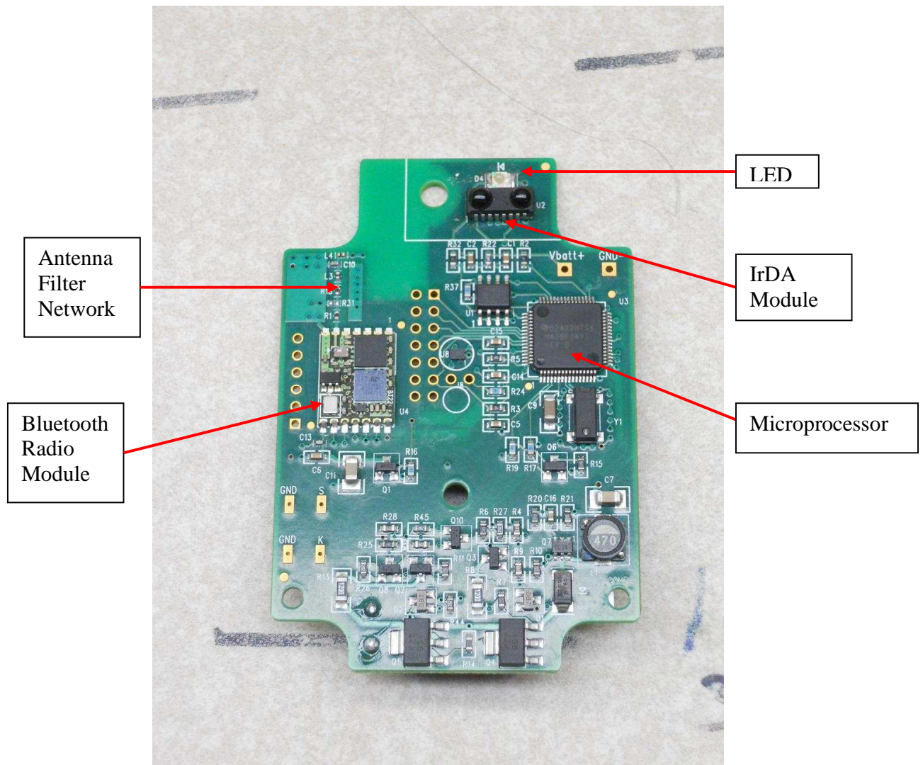
Circuit Board Front View
