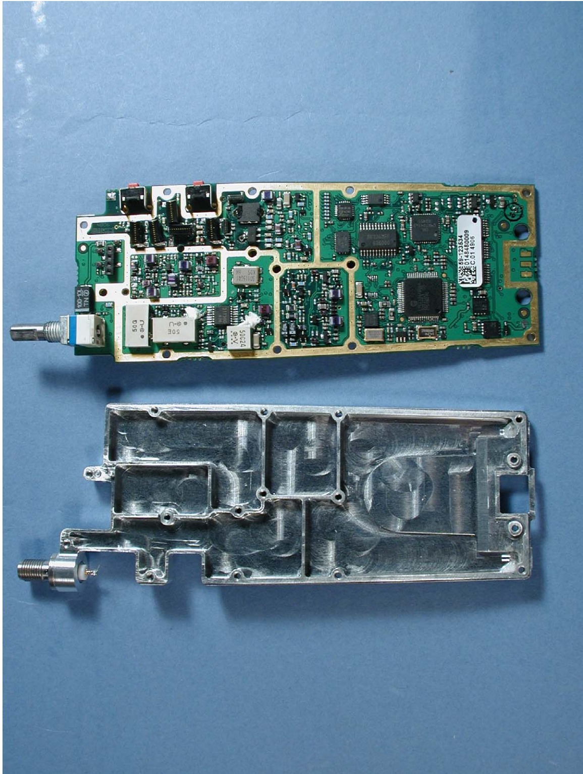
Photograph 3: PCB bottom view (uncovered)
