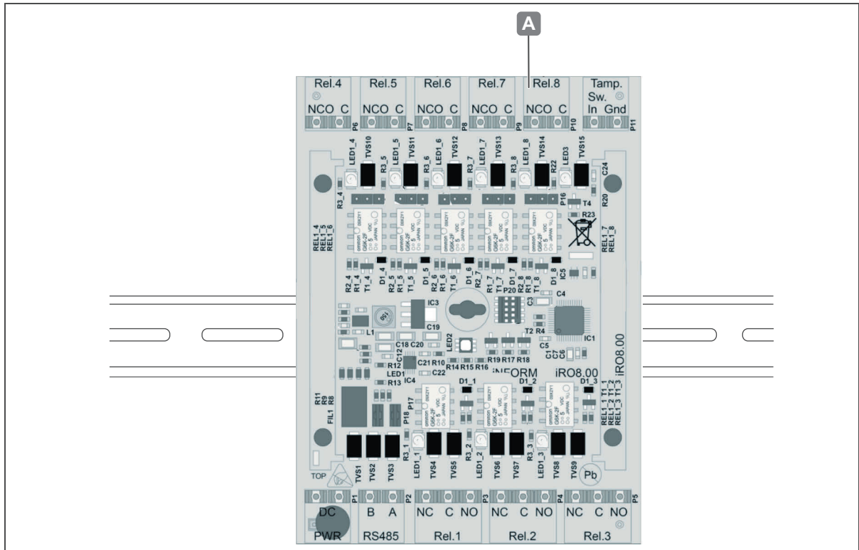
Fig. 11: WTX 201 installation on top hat rail
