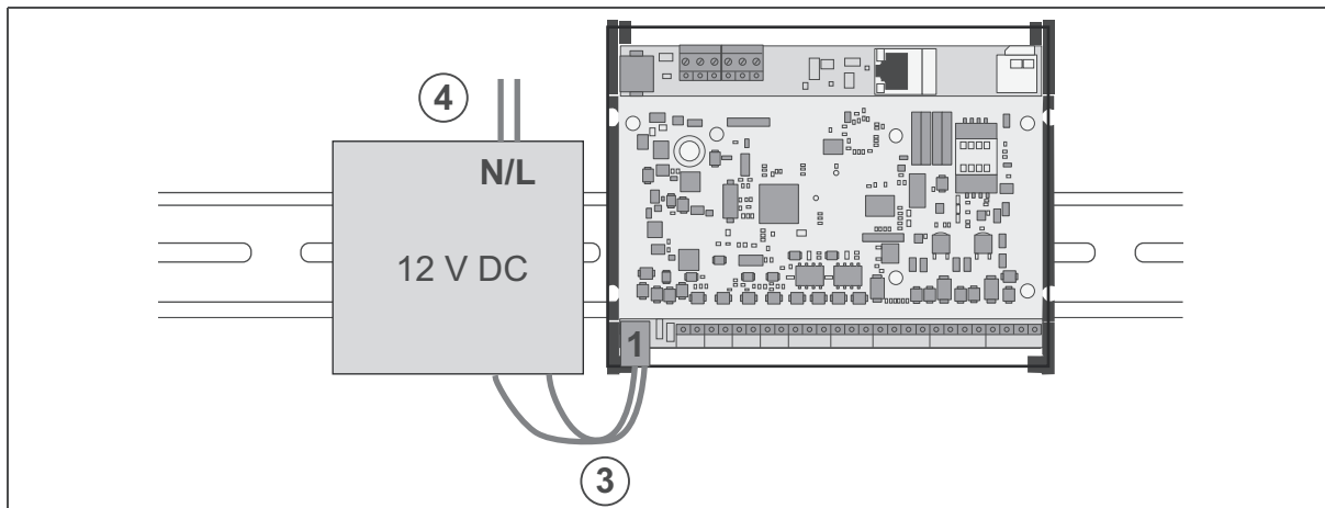
Fig. 6: Montage WTC 200
