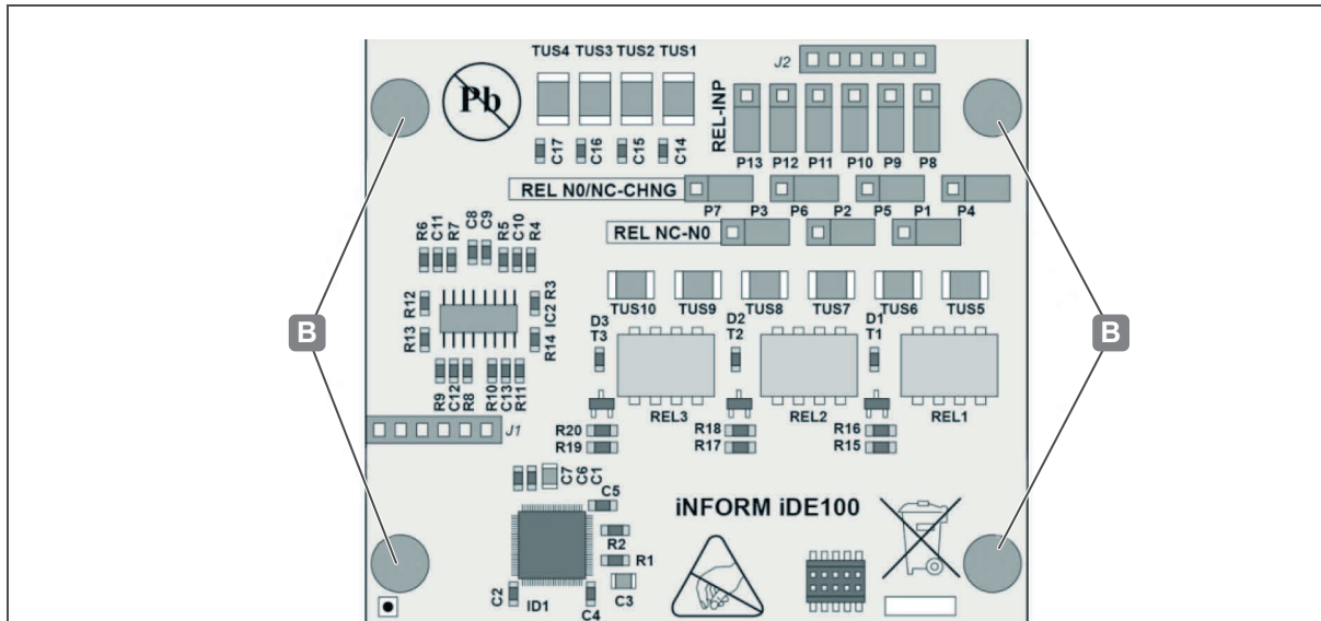
Fig. 8: I/O WTX 200 installation - installing spacers
