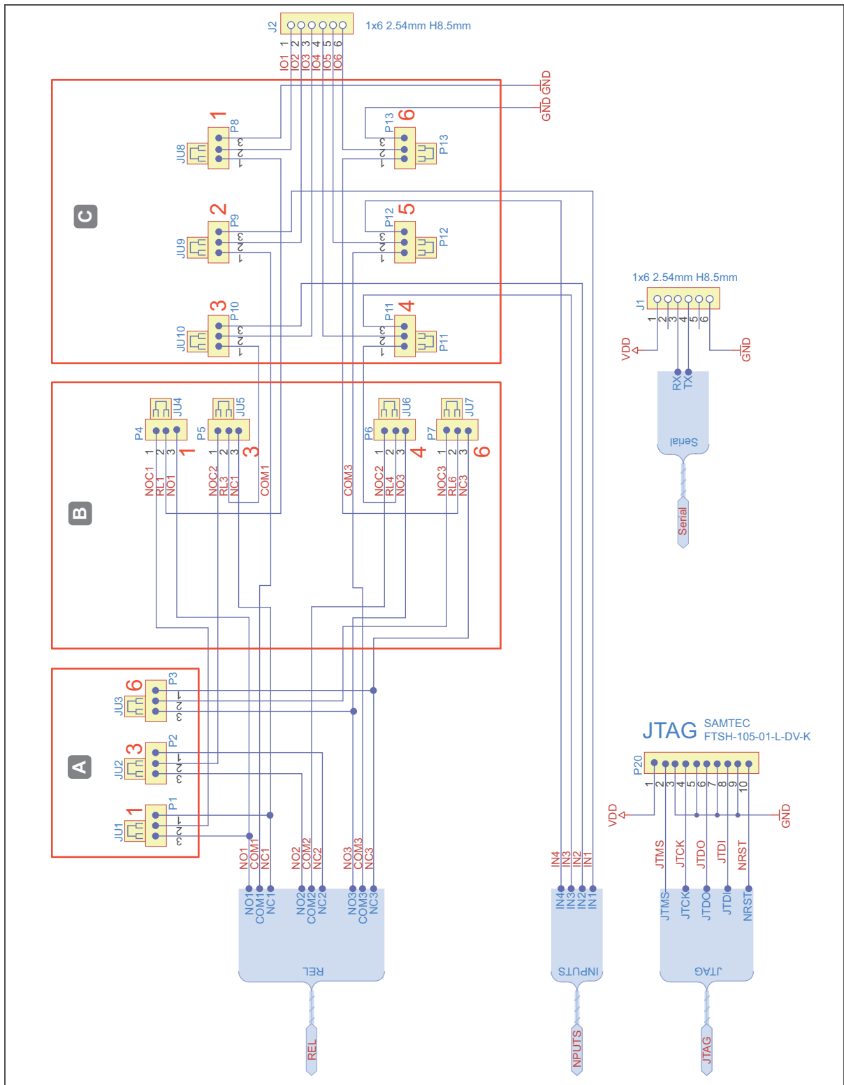
Fig. 16: Structure and pin assignment of the I/O WTX 200
