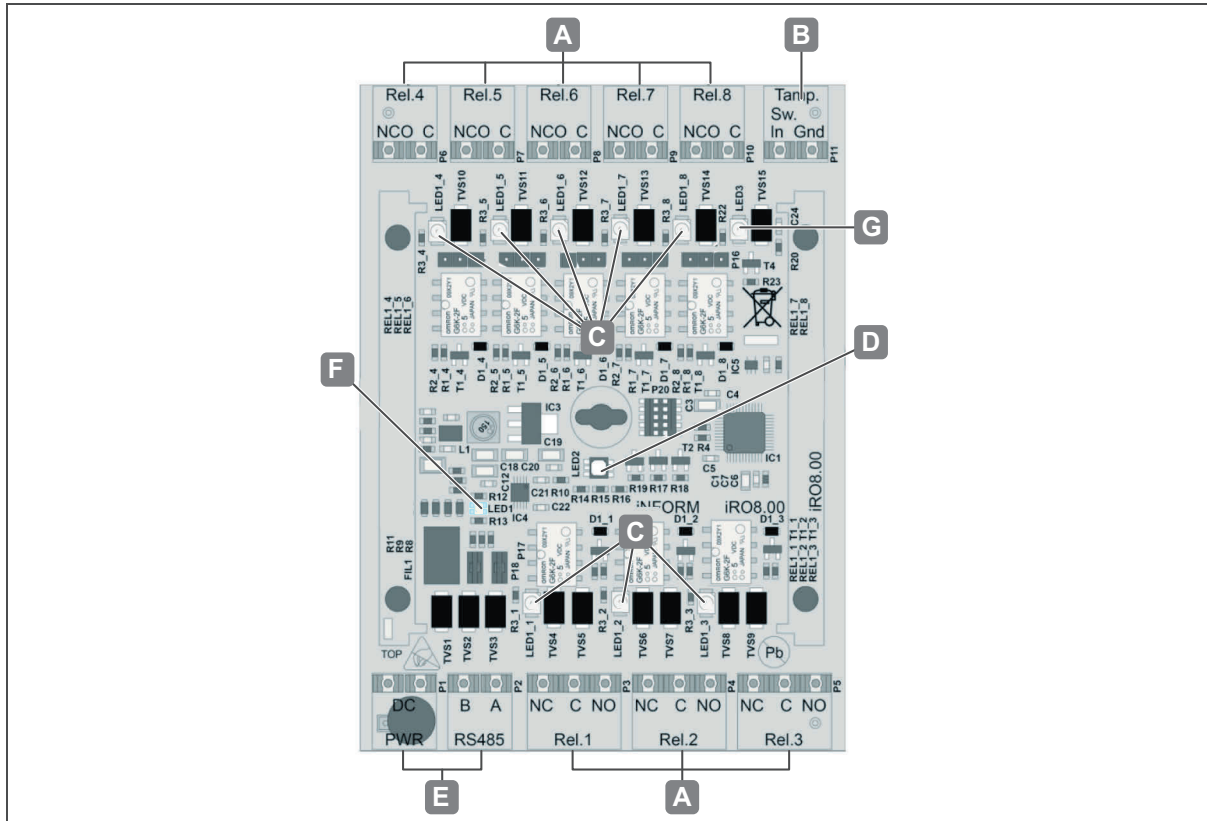
Fig. 20: WTX 201 connections
