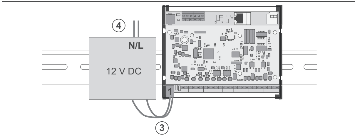
Abb. 6: Montage WTC 200
