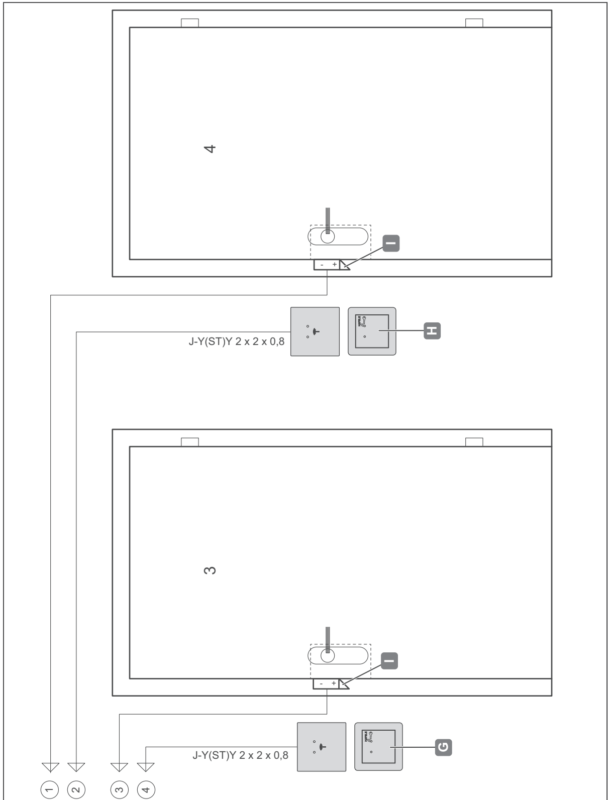
Fig. 32: Installation example 5 - part 2 - four doors with one reader / electric strike and one controller each (including add-on module)
