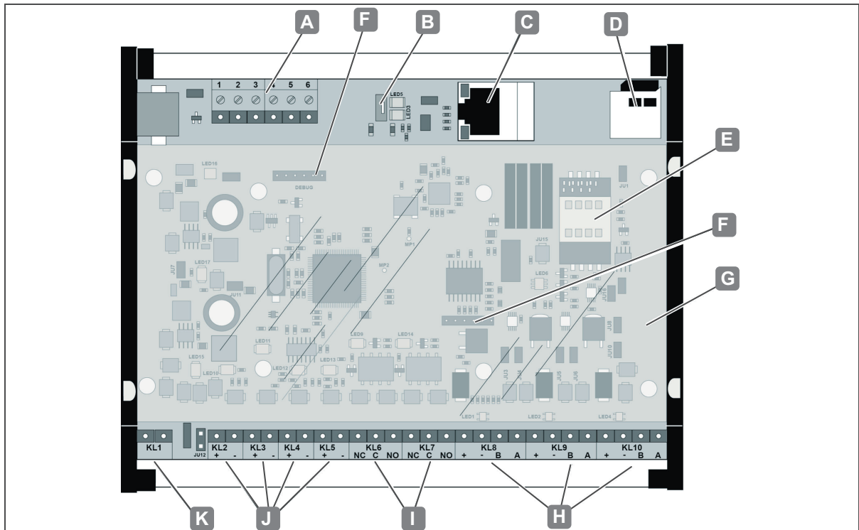
Fig. 14: WTC 200 connections
