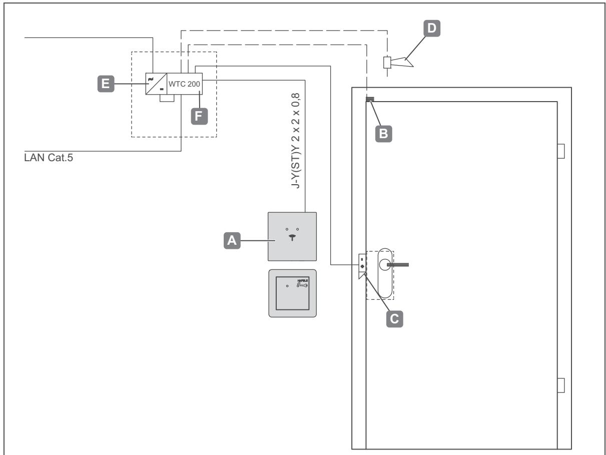
Fig. 23: Installation example 1 - a door with a reader, door signalling contact, electric strike, signal generator and controller
