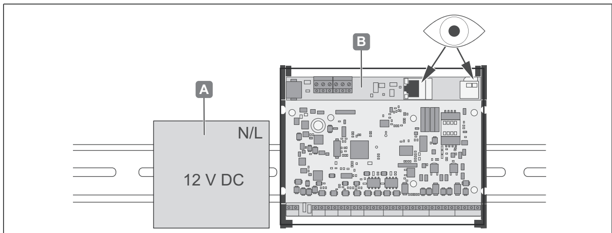
Abb. 5: Montage WTC 200
