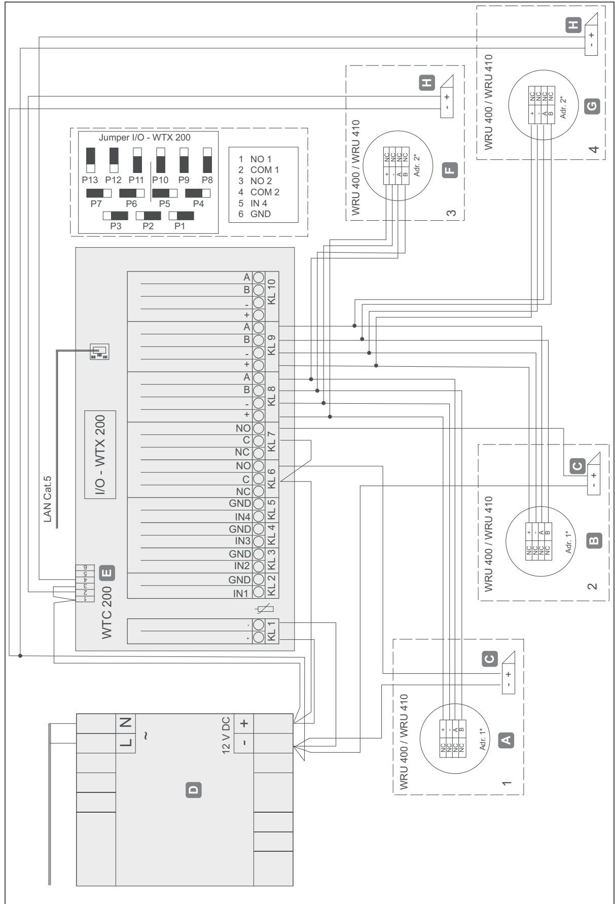
Fig. 33: Circuit diagram for installation example 5
