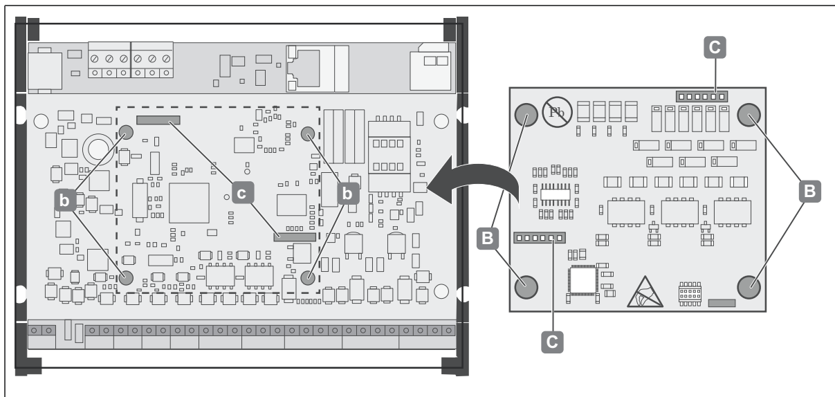
Fig. 9: I/O WTX 200 Installation - clipping I/O WTX 200 onto WTC 200 controller
