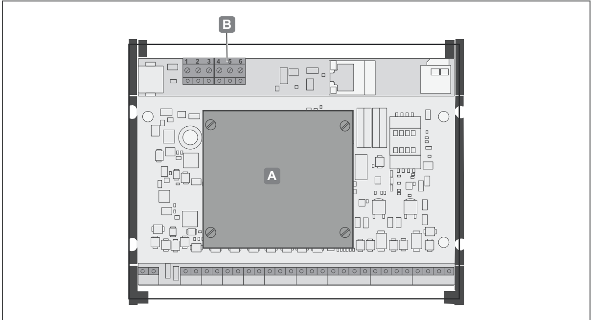
Fig. 15: I/O WTX 200 connections
