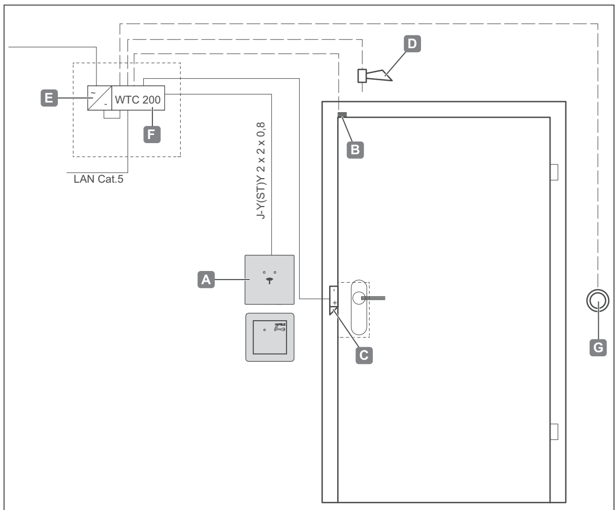
Fig. 25: Installation example 2 - a door with a reader, door signalling contact, electric strike, signal generator, door release button and controller
