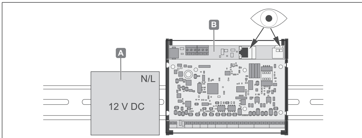
Fig. 5: Montage WTC 200
