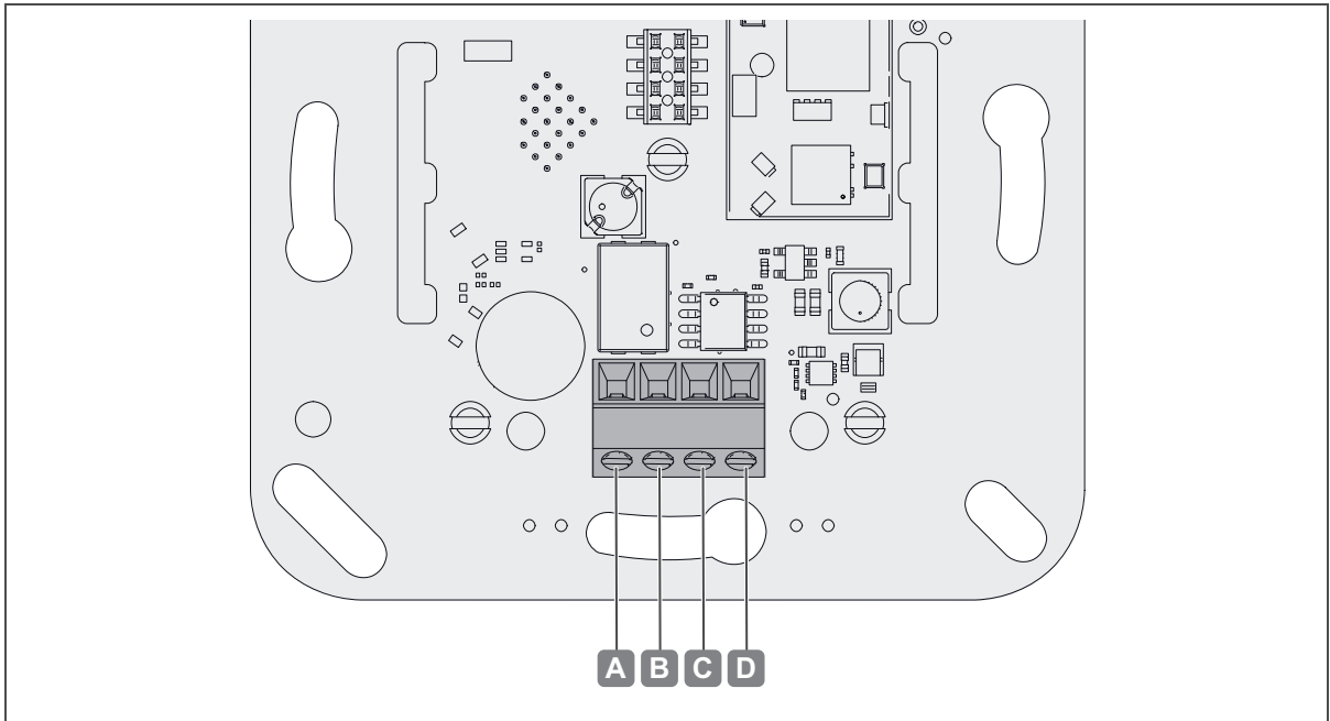
Fig. 13: WRU 400 / WRU 410 connections
