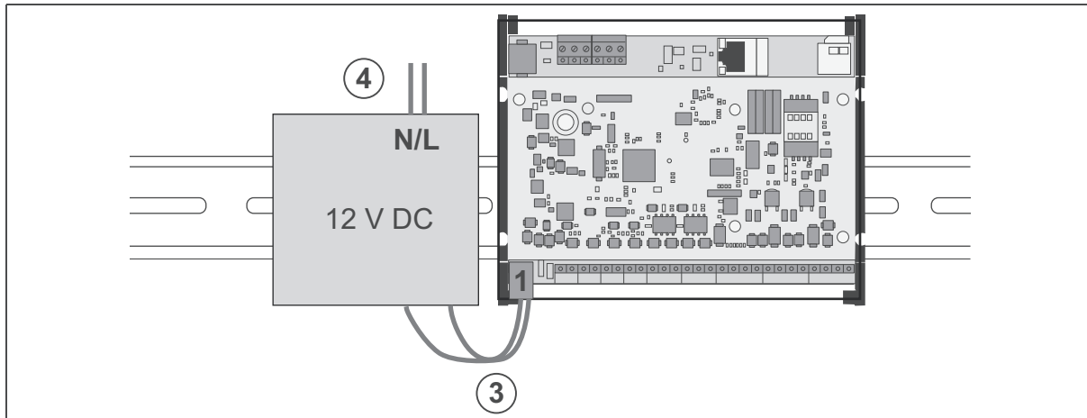
Fig. 6: WTC 200 installation
