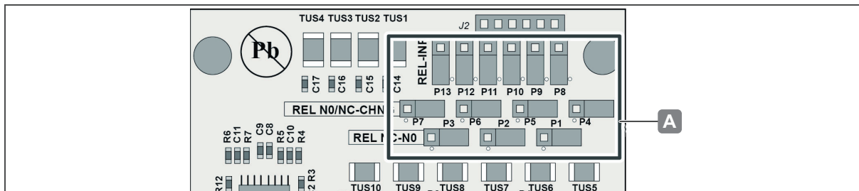
Fig. 7: I/O WTX 200 installation - setting jumper
