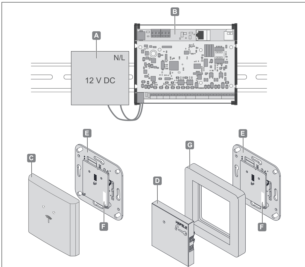
Fig. 1: System overview
