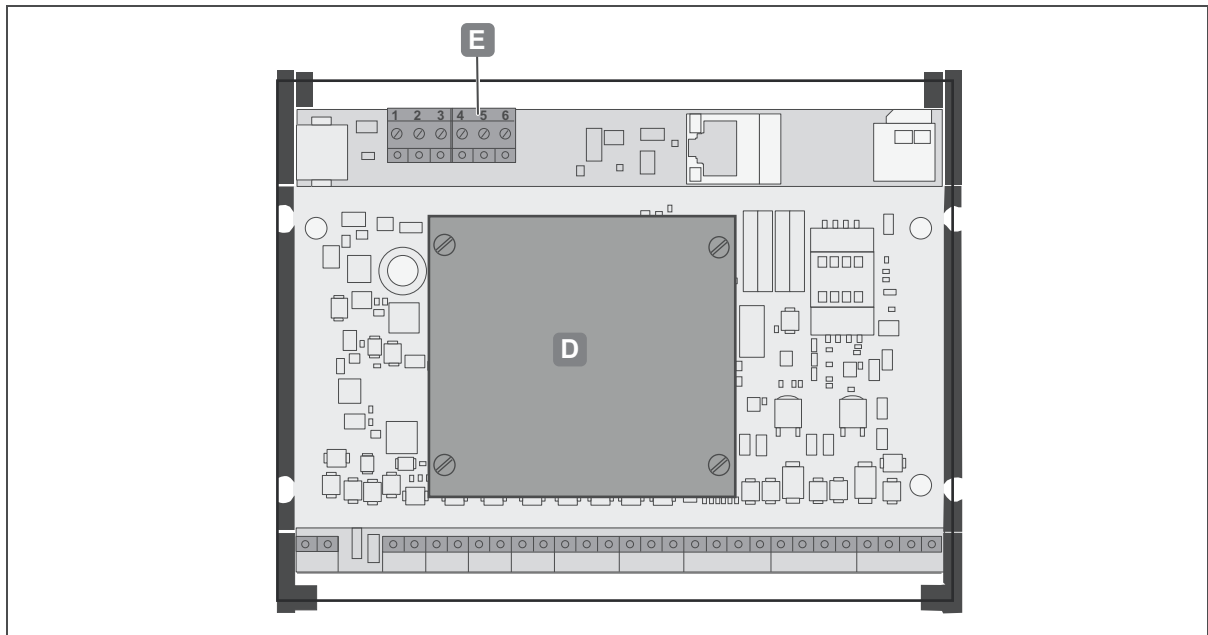
Fig. 10: I/O WTX 200 installation - connected to controller
