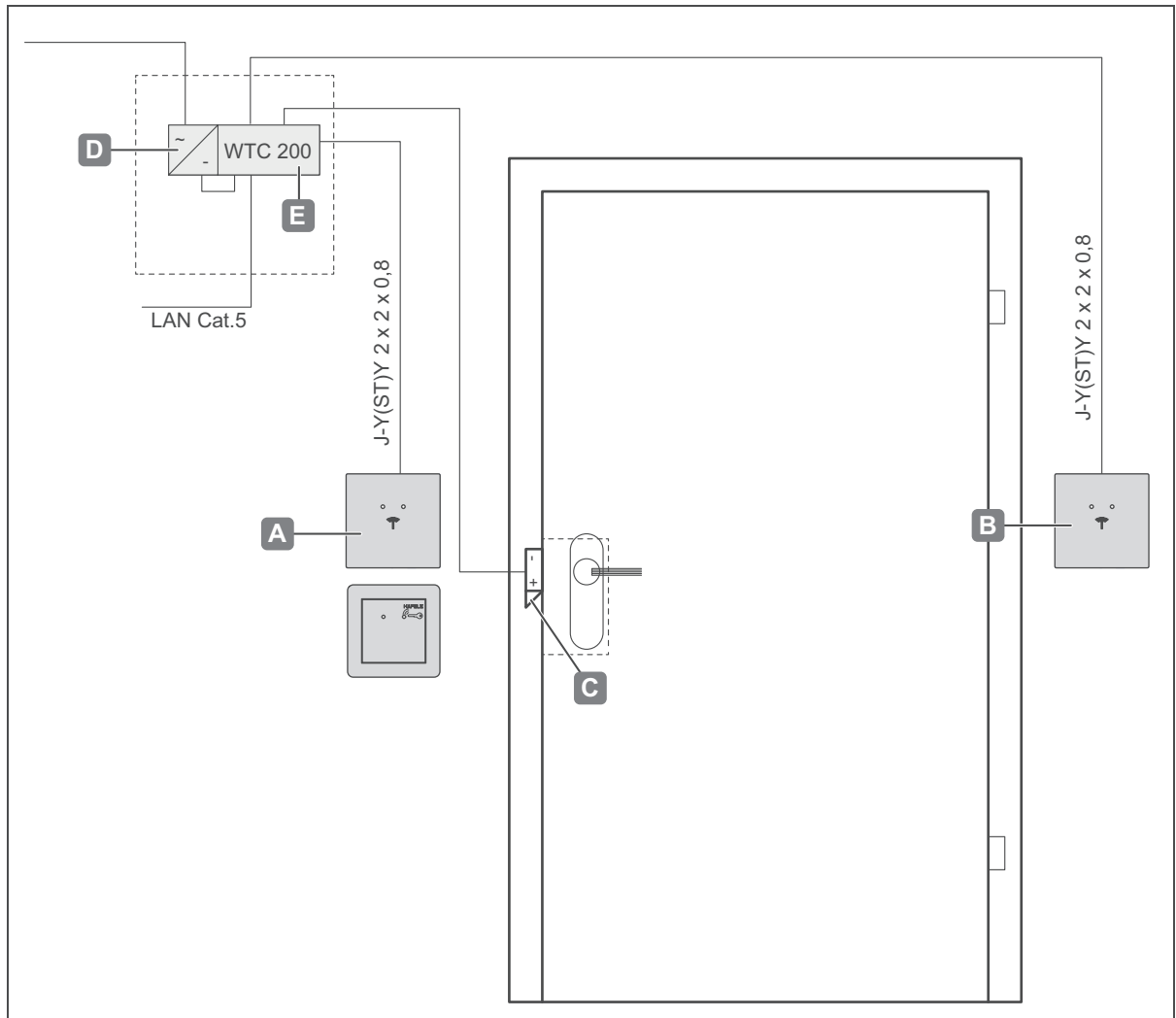
Fig. 27: Installation example 3 - a door with two readers (e.g. inside and outside), electric strike and controller
