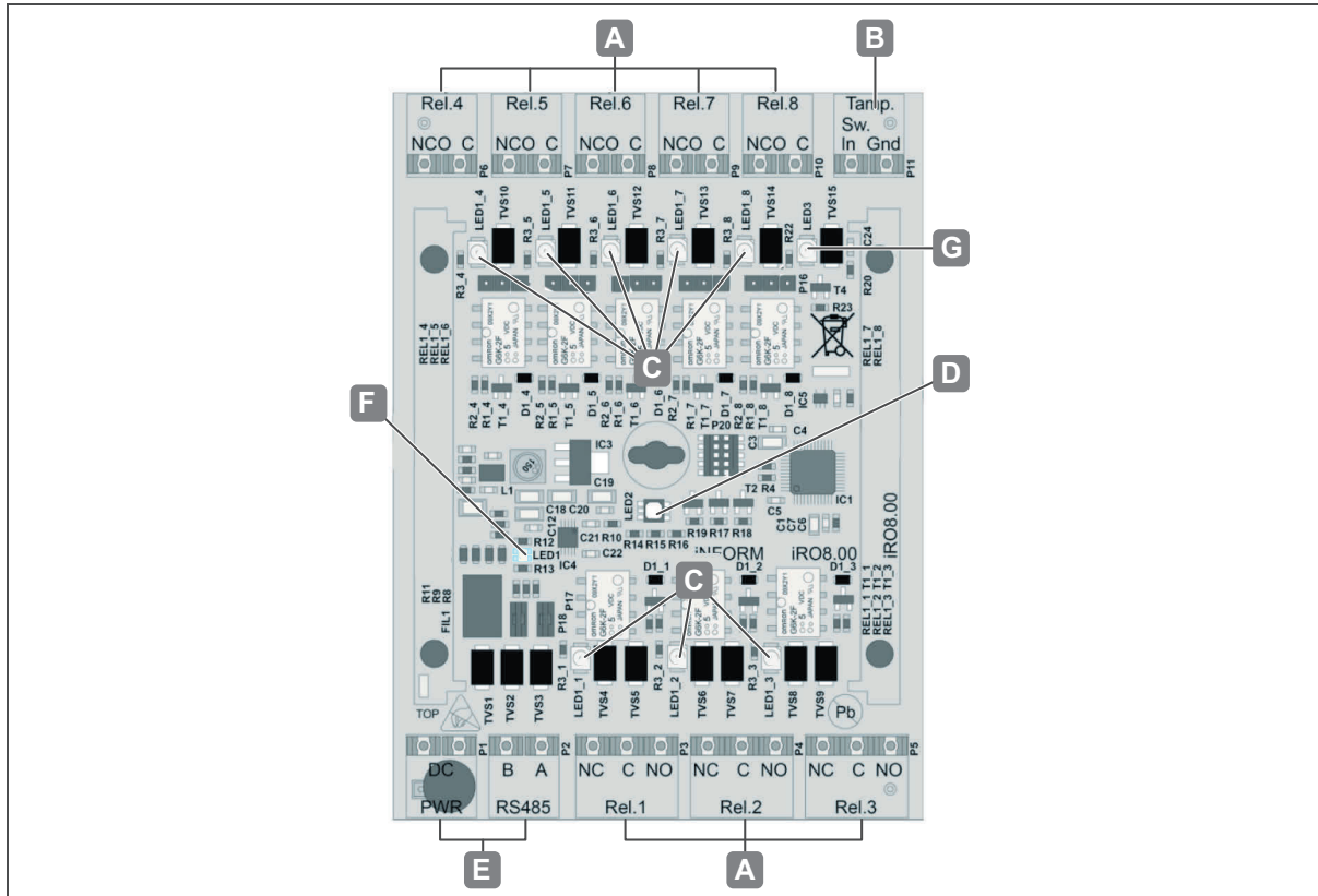
Abb. 20: Anschlüsse WTX 201
