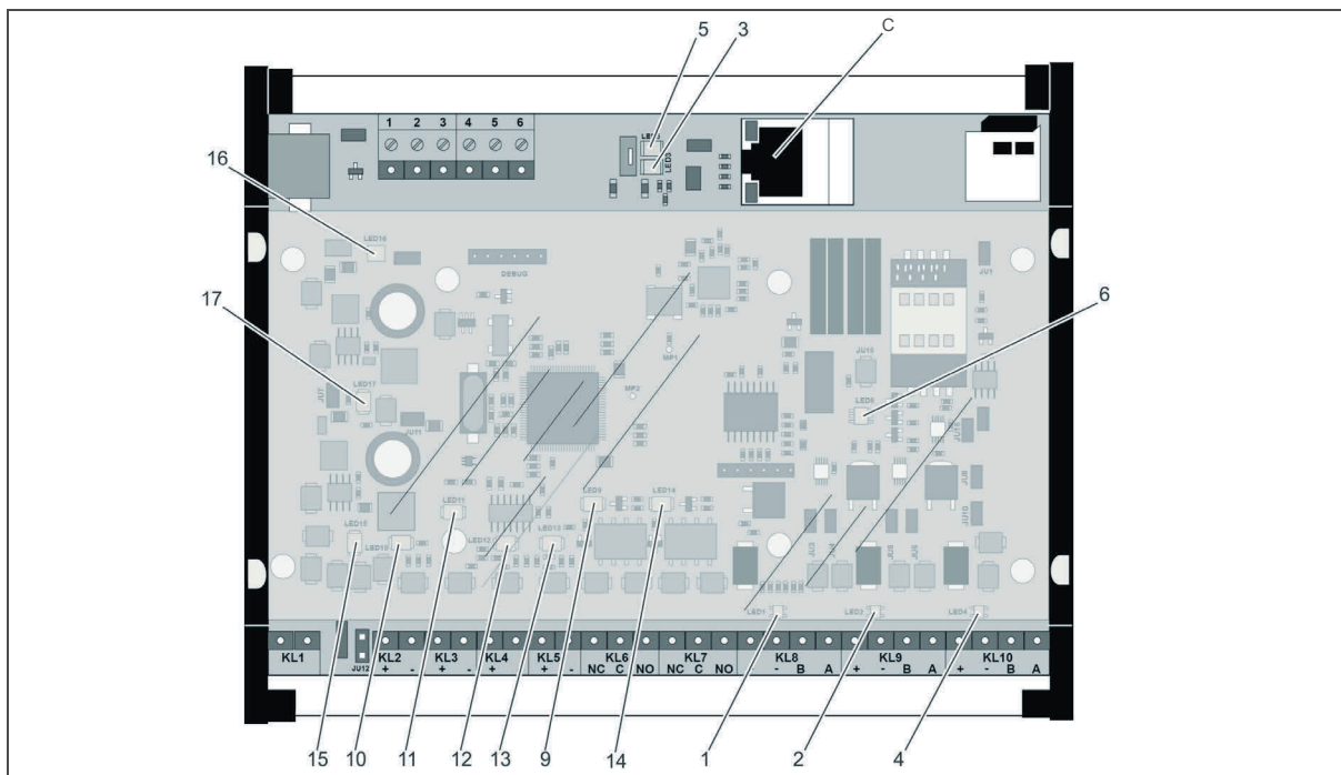
Fig. 12: Overview of LEDs on the WTC 200 controller
