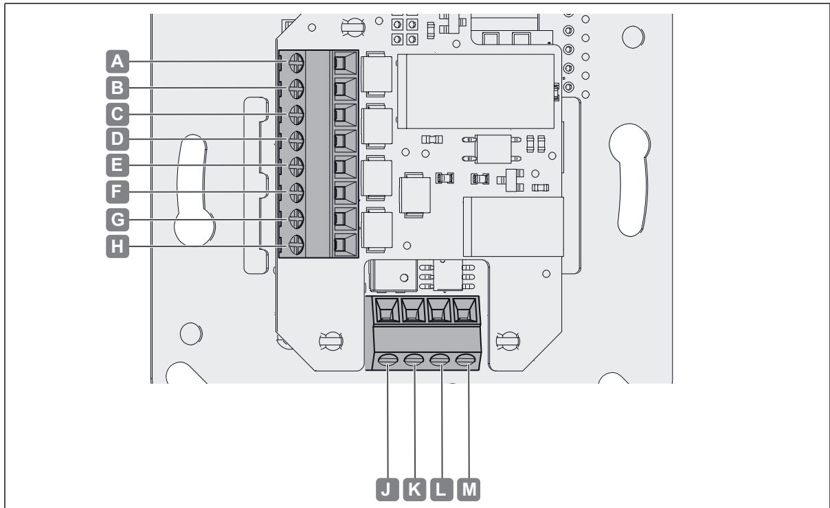
Abb. 2: Anschlüsse
