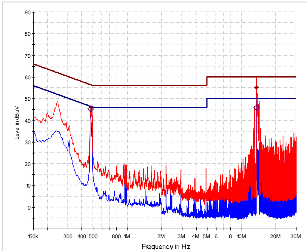
— Preview Result 2-AVG — Preview Result 1-PK+ — FCC 15.107 Class B QP — FCC 15.107 Class B AV * Final Result QP K ◊ Final Result AVG
