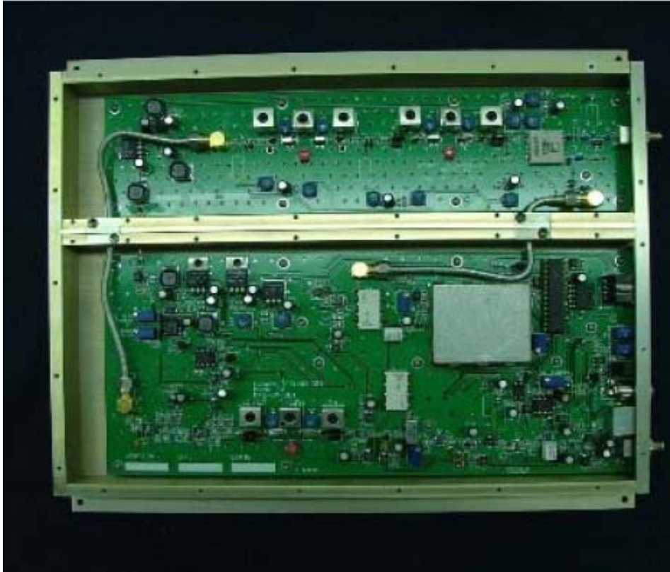
EUT - Cover Off View Without Shields
