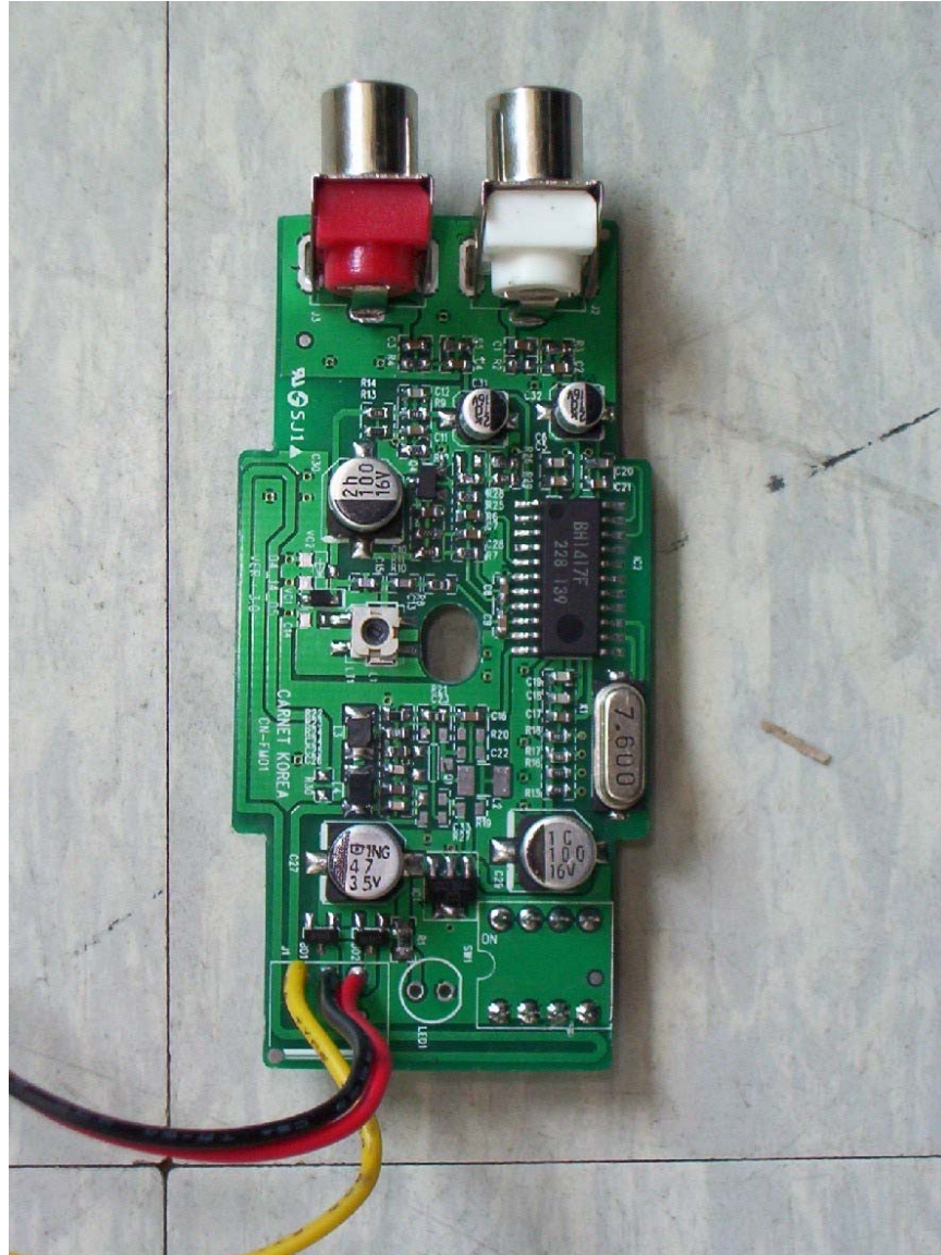
Mainboard ( Components side)
