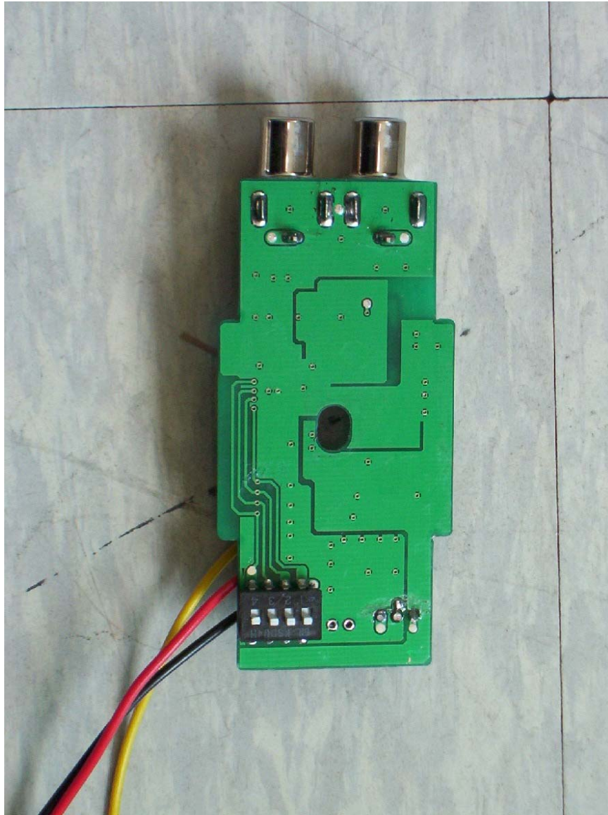
Mainboard ( Copper side)
