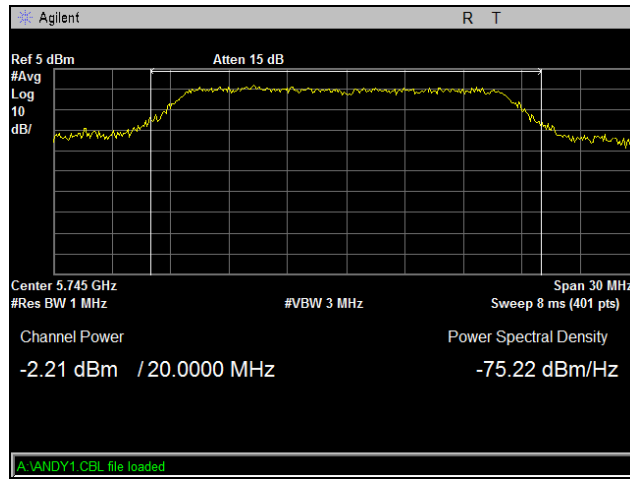
Plot 4. Maximum Conducted Output Power, 802.11a, Low Channel
