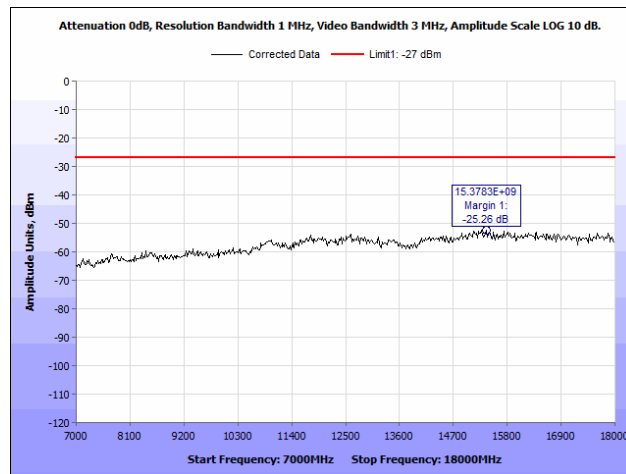
Plot 12. Radiated Spurious Emissions, 802.11a, Low Channel, 7 GHz – 18 GHz, Peak
