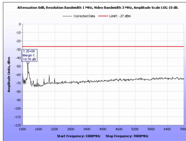
Plot 17. Radiated Spurious Emissions, 802.11a, High Channel, 1 GHz – 7 GHz, Peak
