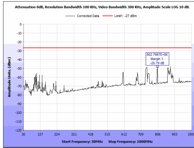
Plot 10. Radiated Spurious Emissions, 802.11a, Low Channel, 30 MHz – 1 GHz
