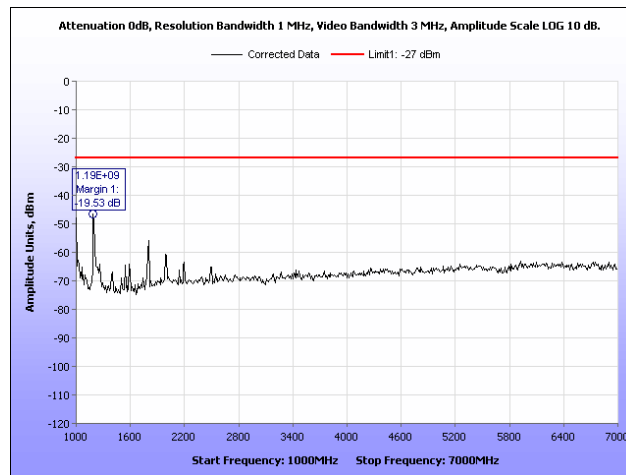
Plot 14. Radiated Spurious Emissions, 802.11a, Mid Channel, 1 GHz – 7 GHz, Peak
