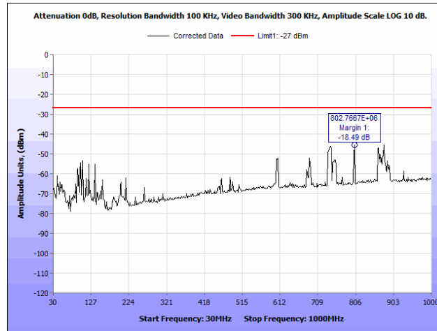
Plot 13. Radiated Spurious Emissions, 802.11a, Mid Channel, 30 MHz – 1 GHz
