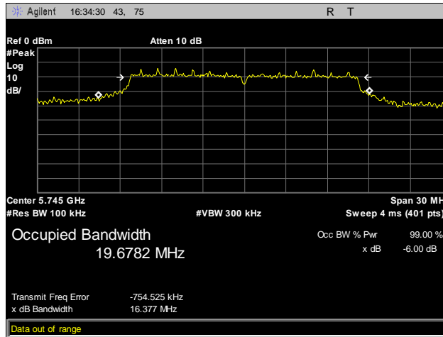
Plot 23. 6 dB Bandwidth, 802.11a, Low Channel
