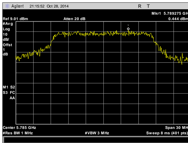
Plot 8. Maximum Power Spectral Density, 802.11a, Mid Channel
