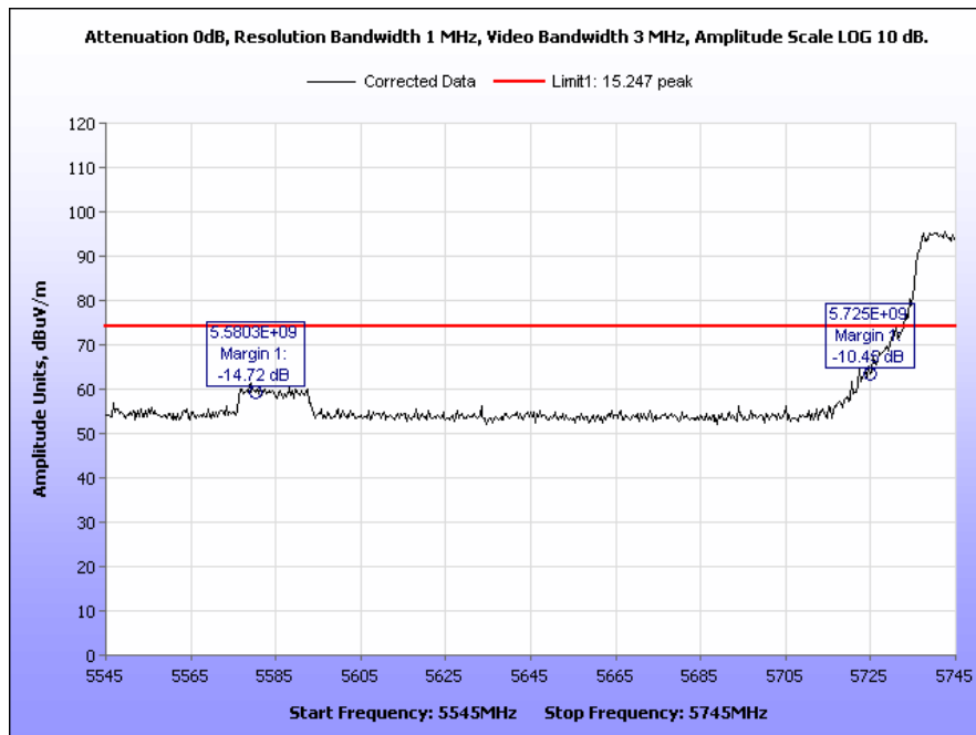
Plot 20. Radiated Band Edge, 802.11a, Low Channel, Peak
