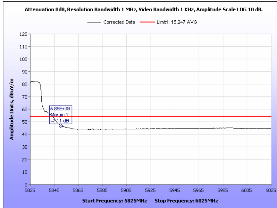
Plot 21. Radiated Band Edge, 802.11a, High Channel, Average
