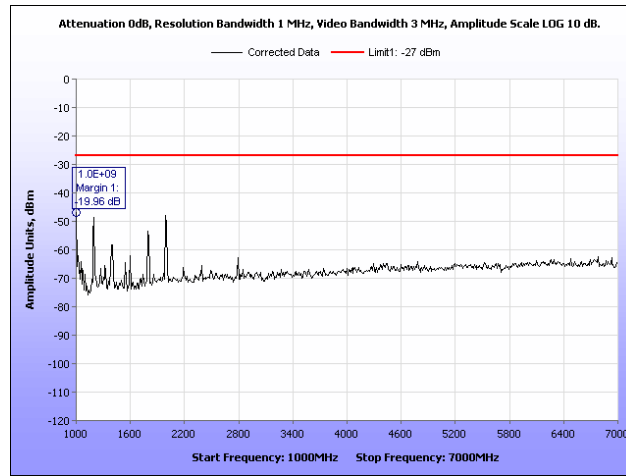
Plot 11. Radiated Spurious Emissions, 802.11a, Low Channel, 1 GHz – 7 GHz, Peak
