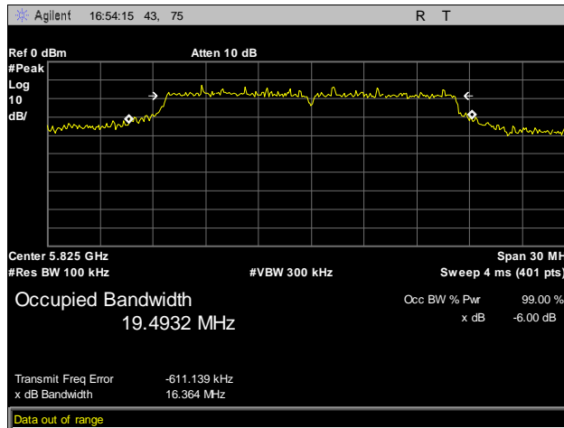
Plot 25. 6 dB Bandwidth, 802.11a, High Channel
