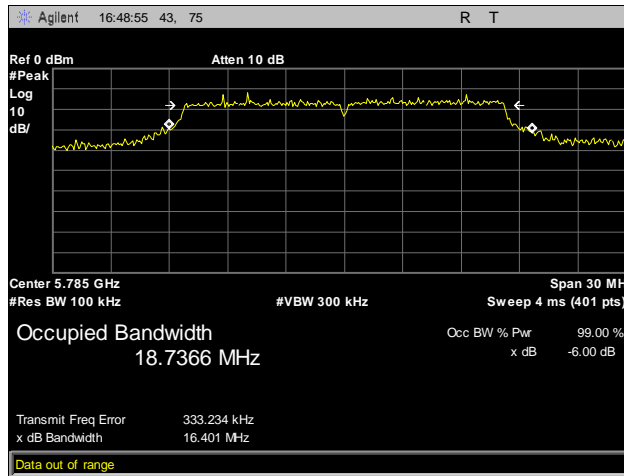
Plot 24. 6 dB Bandwidth, 802.11a, Mid Channel
