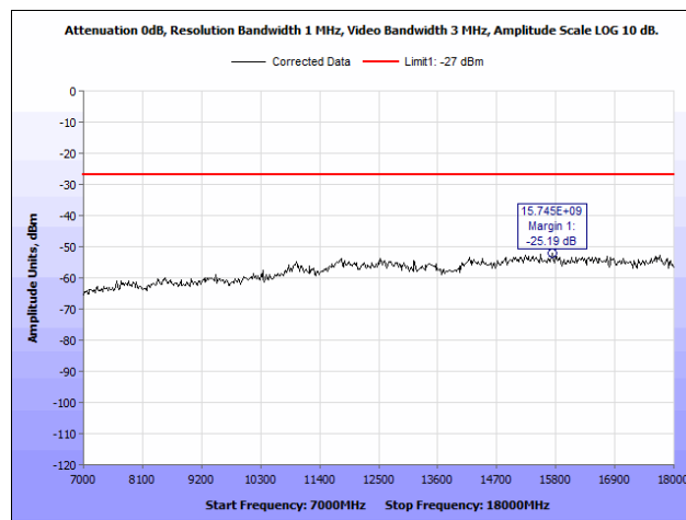
Plot 15. Radiated Spurious Emissions, 802.11a, Mid Channel, 7 GHz – 18 GHz, Peak
