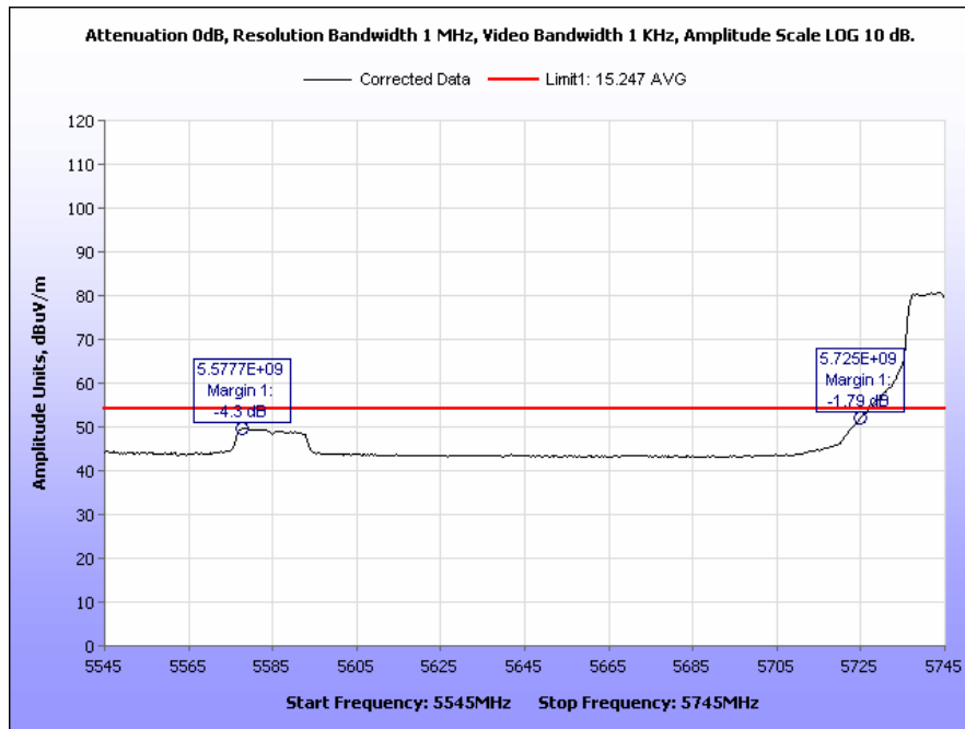
Plot 19. Radiated Band Edge, 802.11a, Low Channel, Average
