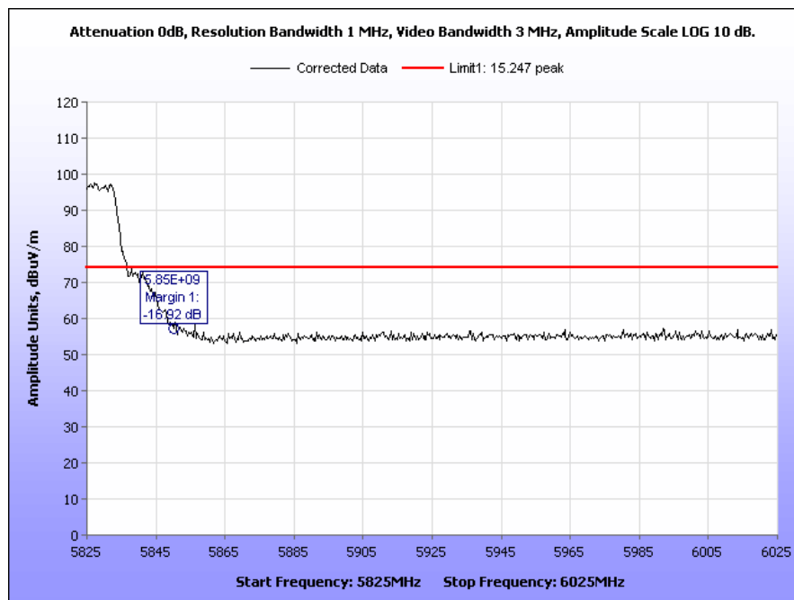
Plot 22. Radiated Band Edge, 802.11a, High Channel, Peak
