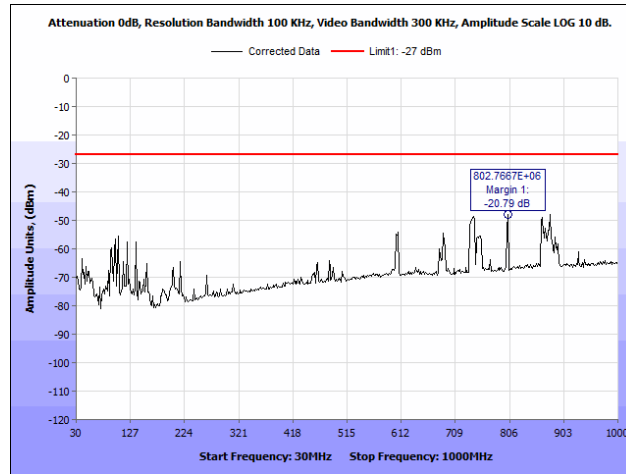
Plot 16. Radiated Spurious Emissions, 802.11a, High Channel, 30 MHz – 1 GHz
