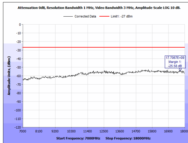
Plot 18. Radiated Spurious Emissions, 802.11a, High Channel, 7 GHz – 18 GHz, Peak
