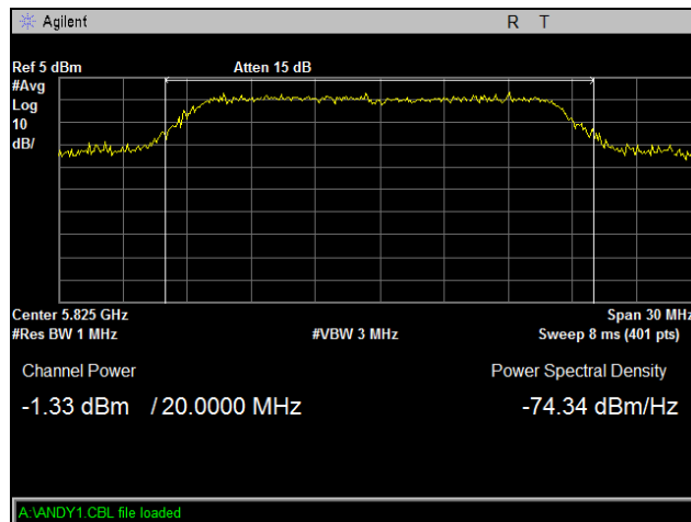
Plot 6. Maximum Conducted Output Power, 802.11a, High Channel
