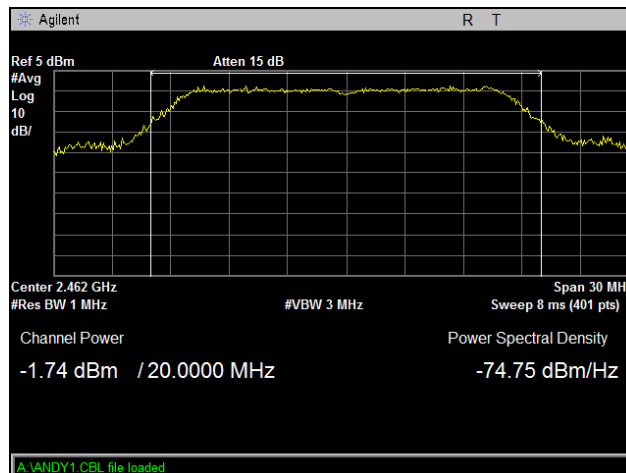
Plot 6. Peak Power Output, High Channel, 802.11g
