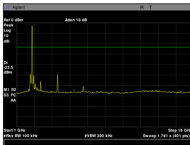
Plot 25. Conducted Spurious Emissions, High Channel, 802.11g, 1 GHz – 18 GHz
