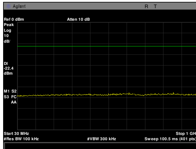
Plot 20. Conducted Spurious Emissions, Low Channel, 802.11g, 30 MHz – 1 GHz
