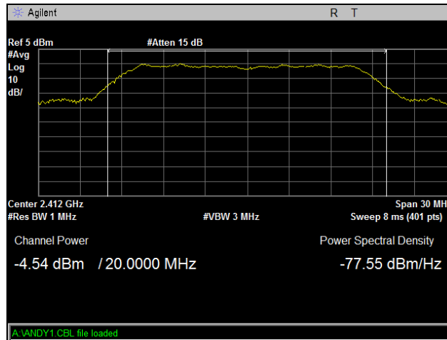
Plot 4. Peak Power Output, Low Channel, 802.11g
