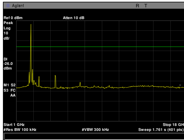
Plot 23. Conducted Spurious Emissions, Mid Channel, 802.11g, 1 GHz – 18 GHz
