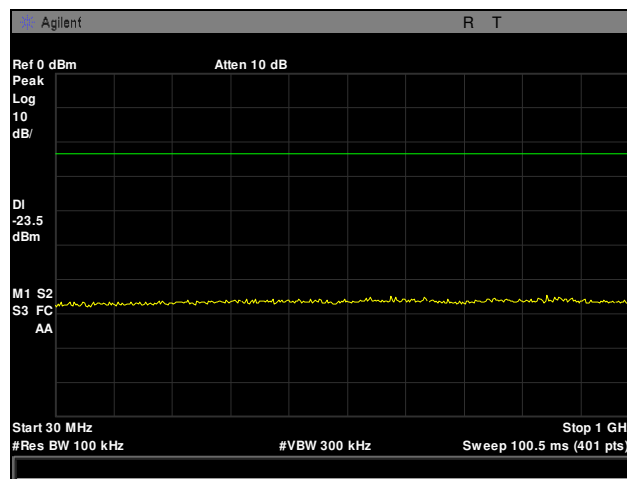
Plot 24. Conducted Spurious Emissions, High Channel, 802.11g, 30 MHz – 1 GHz
