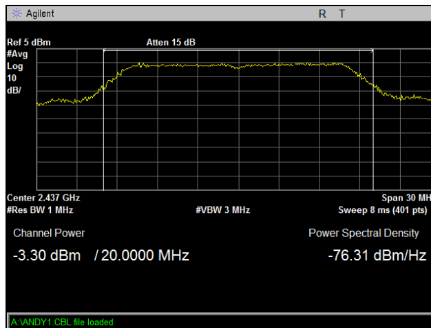
Plot 5. Peak Power Output, Mid Channel, 802.11g
