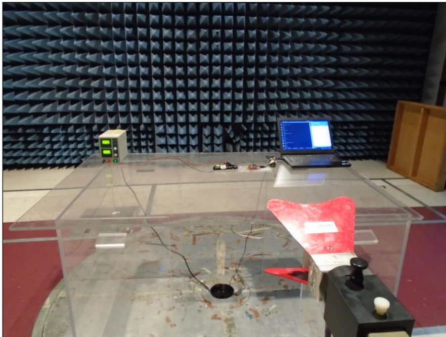
Photograph 2. Radiated Spurious Emissions, Test Setup, 1 GHz – 18 GHz
