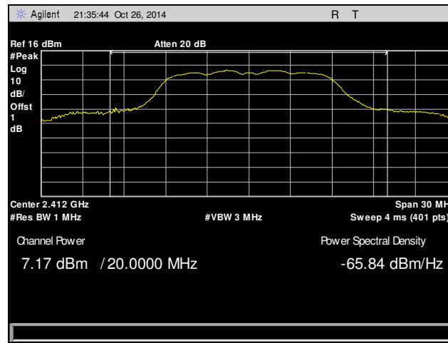
Plot 7. Peak Power Output, Low Channel, 2412 MHz, 802.11g
