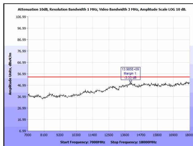
Plot 36. Radiated Spurious Emissions, High Channel, 2462 MHz, 802.11n, 7 GHz – 18 GHz, Average
