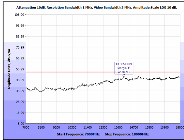
Plot 16. Radiated Spurious Emissions, Low Channel, 2412 MHz, 802.11g, 7 GHz – 18 GHz, Average
