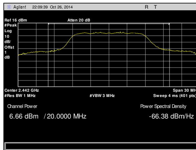
Plot 8. Peak Power Output, Mid Channel, 2442 MHz, 802.11g
