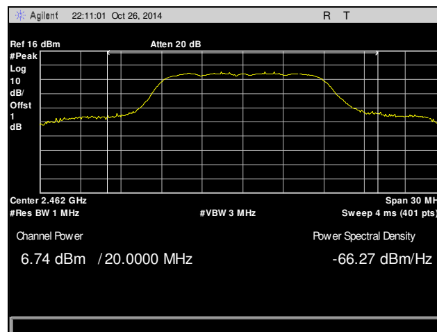
Plot 9. Peak Power Output, High Channel, 2462 MHz, 802.11g
