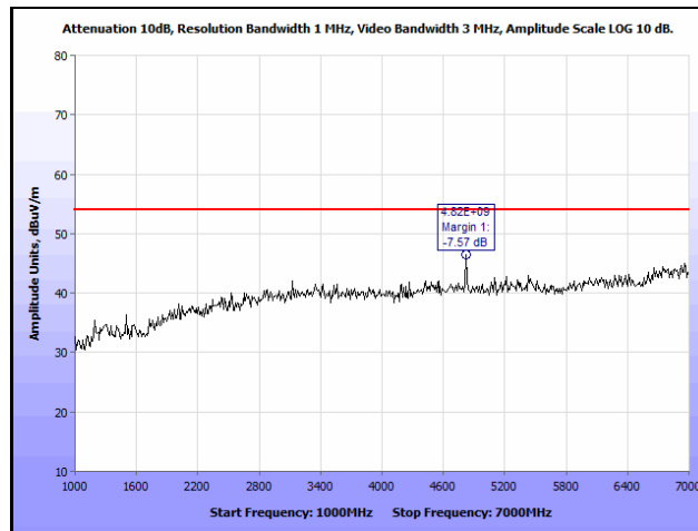
Plot 23. Radiated Spurious Emissions, High Channel, 2462 MHz, 802.11g, 1 GHz – 7 GHz, Average
