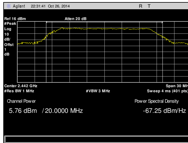
Plot 11. Peak Power Output, Mid Channel, 2442 MHz, 802.11n
