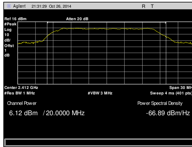
Plot 10. Peak Power Output, Low Channel, 2412 MHz, 802.11n
