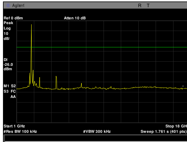
Plot 54. Conducted Spurious Emissions, Mid Channel, 2442 MHz, 802.11n, 1 GHz – 18 GHz
