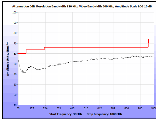
Plot 22. Radiated Spurious Emissions, High Channel, 2462 MHz, 802.11g, 30 MHz – 1 GHz, Peak
