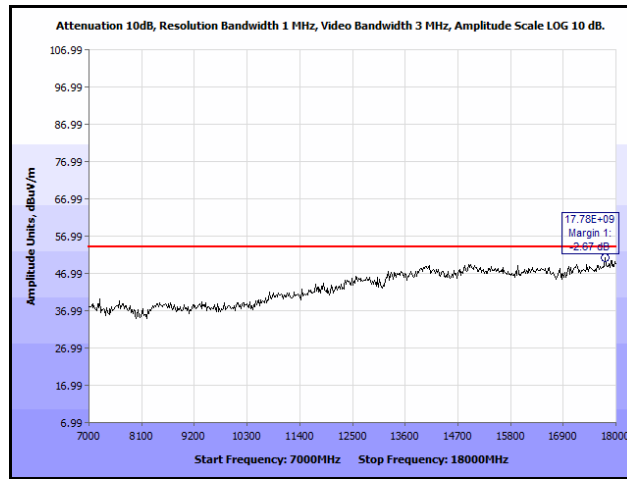
Plot 28. Radiated Spurious Emissions, Low Channel, 2412 MHz, 802.11n, 7 GHz – 18 GHz, Average
