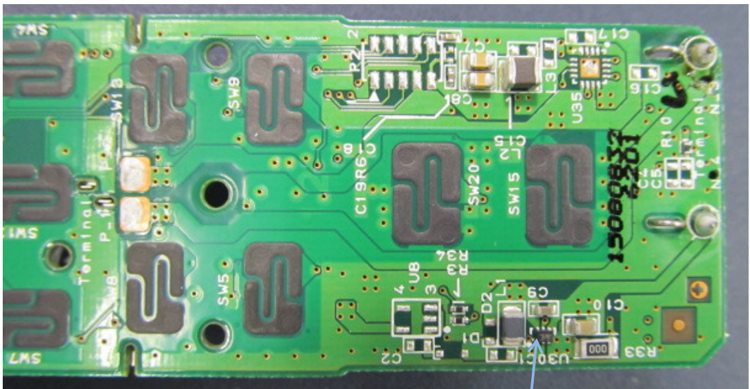
Voltage Regulator 1.8V Output(U30)
