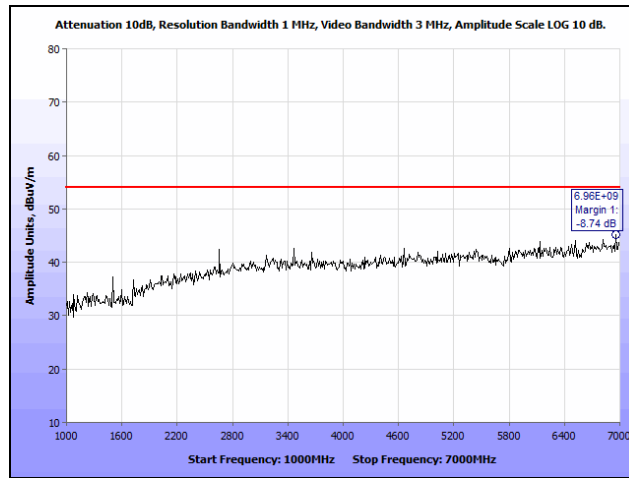
Plot 11. Radiated Spurious Emissions, Low Channel, 5745 MHz, 802.11a, 1 GHz – 7 GHz, Peak under Avg. Limit
