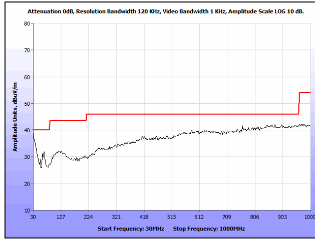
Plot 10. Radiated Spurious Emissions, Low Channel, 5745 MHz, 802.11a, 30 MHz – 1 GHz, Average
