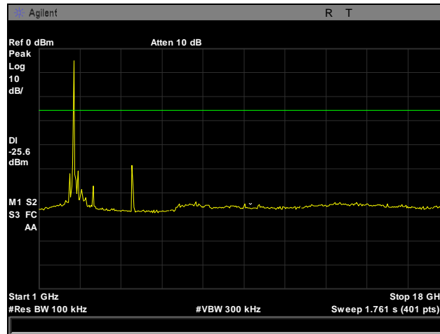
Plot 48. Conducted Spurious Emissions, Mid Channel, 2442 MHz, 802.11b, 1 GHz – 18 GHz
