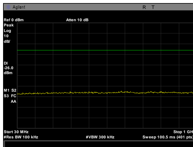
Plot 53. Conducted Spurious Emissions, Mid Channel, 2442 MHz, 802.11g, 30 MHz – 1 GHz
