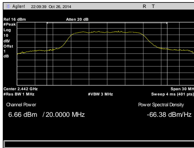
Plot 8. Peak Power Output, Mid Channel, 2442 MHz, 802.11b
