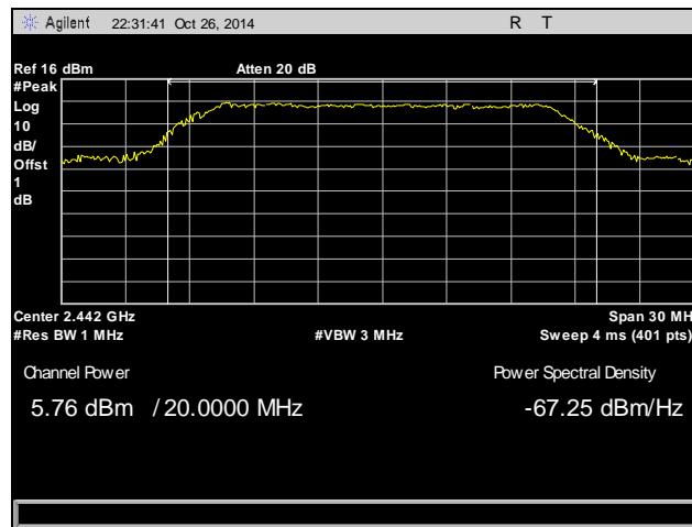
Plot 11. Peak Power Output, Mid Channel, 2442 MHz, 802.11g
