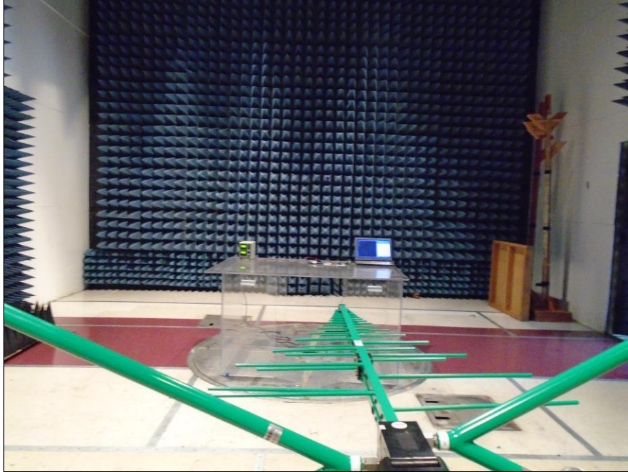
Photograph 2. Radiated Spurious Emissions, 30MHz – 1GHz
