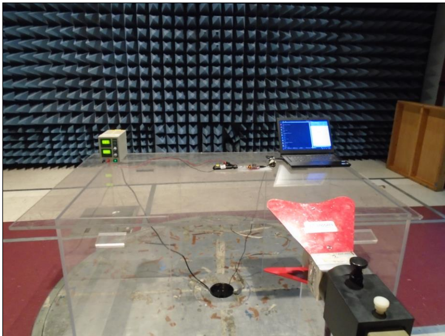
Photograph 3. Radiated Spurious Emissions, 1GHz – 18GHz
