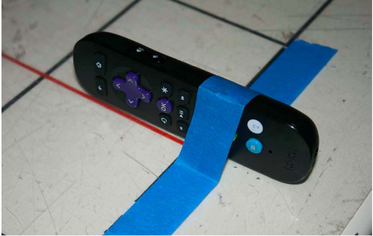
RADIATED EMISSIONS TEST SETUP
