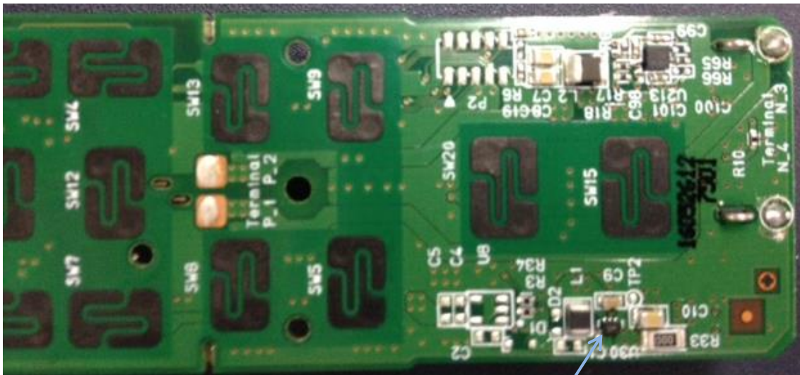
Voltage Regulator 1.85V Output(U30)
