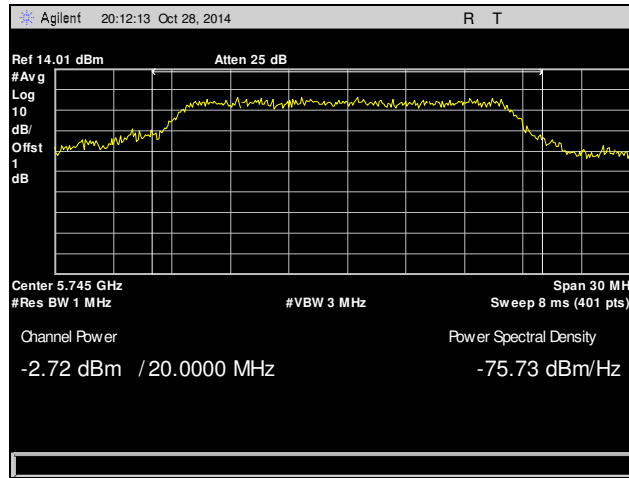
Plot 4. Peak Power Output, Low Channel, 5745 MHz, 802.11a
