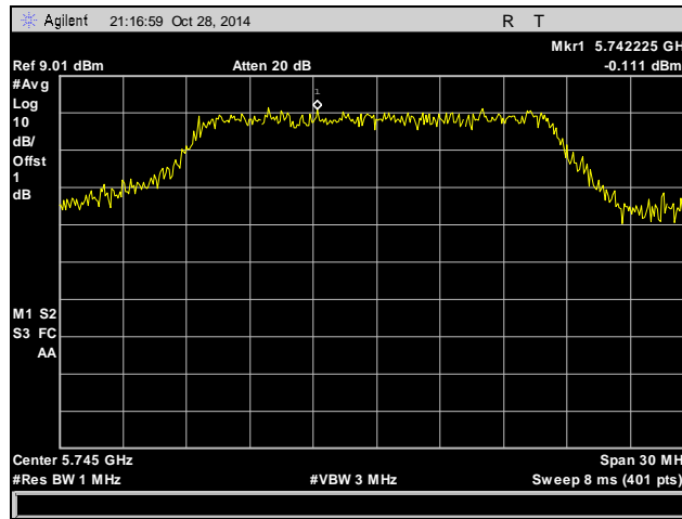
Plot 7. Peak Power Spectral Density, Low Channel, 5745 MHz, 802.11a
