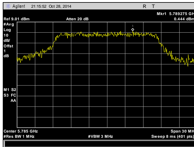
Plot 8. Peak Power Spectral Density, Mid Channel, 5785 MHz, 802.11a
