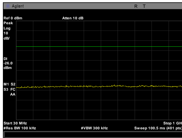
Plot 25. Conducted Spurious Emissions, Mid Channel, 2442 MHz, 802.11g, 30 MHz – 1 GHz
