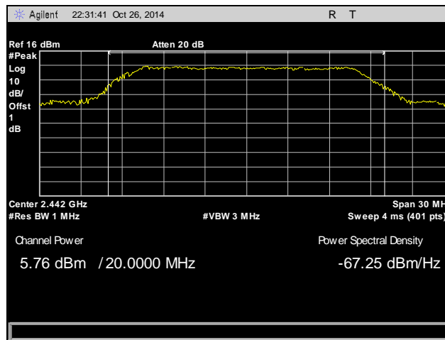
Plot 5. Peak Power Output, Mid Channel, 2442 MHz, 802.11g
