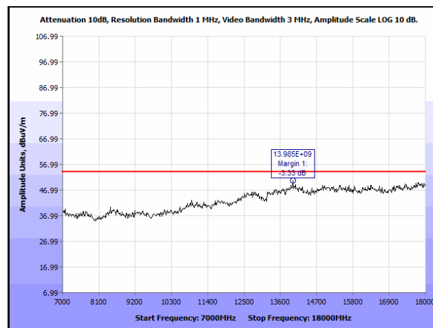
Plot 18. Radiated Spurious Emissions, High Channel, 2462 MHz, 802.11g, 7 GHz – 18 GHz, Average
