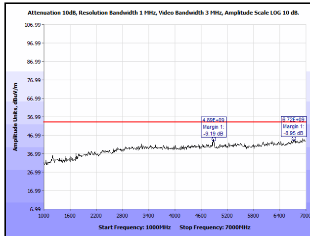
Plot 13. Radiated Spurious Emissions, Mid Channel, 2442 MHz, 802.11g, 1 GHz – 7 GHz, Average
