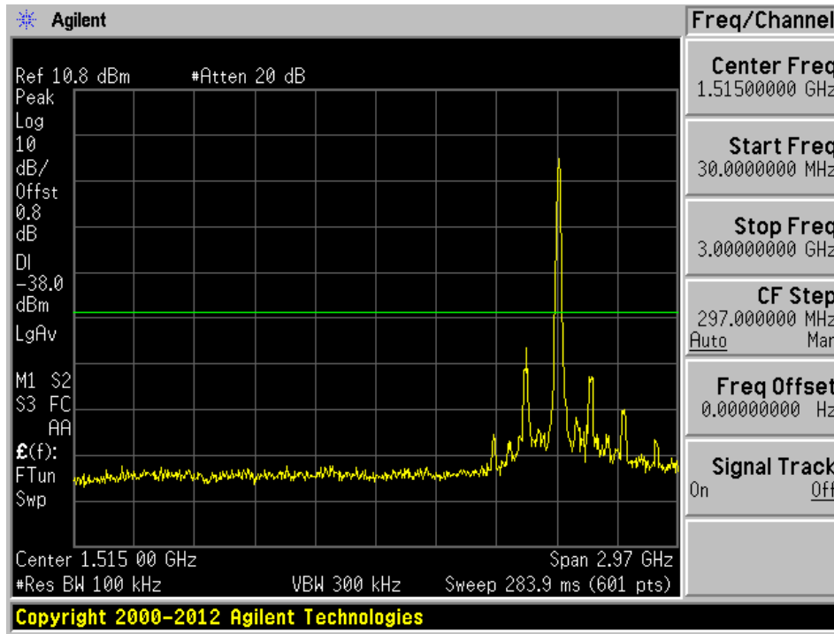
ANT 1 G Mode 2412 MHz Low Channel Spurious Emission_2
