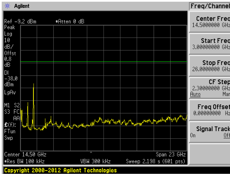
ANT 1 G Mode 2412 MHz Low Channel Spurious Emission_2
