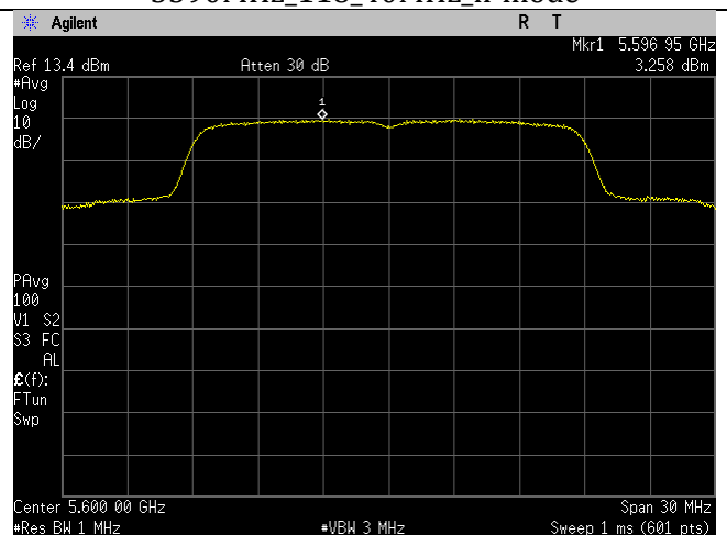
5600MHz_120_20MHz_n-mode
