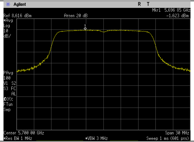
5700MHz_140_20MHz_a-mode
