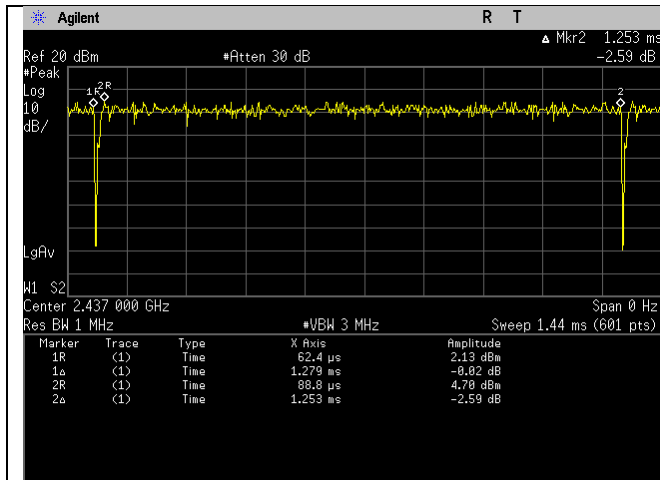
2.4band_n20_mode_Duty_Cycle
