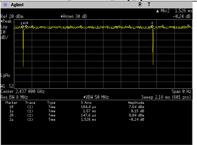
2.4band_ax40mode_Duty_Cycle
