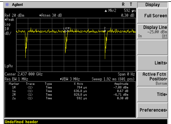
2.4band_n40_mode_Duty_Cycle
