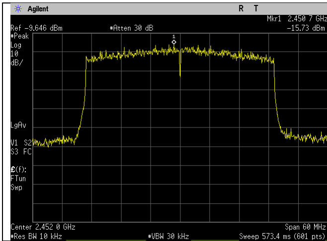
High Ch_2452MHz_40MHz BW_ax-mode_Spectral Density_Port 1
