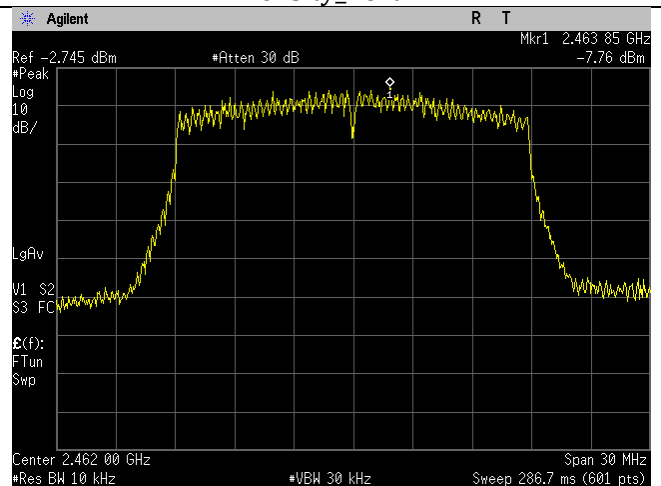
High Ch_2462MHz_20MHz BW_n-mode_Spectral Density_Port 2
