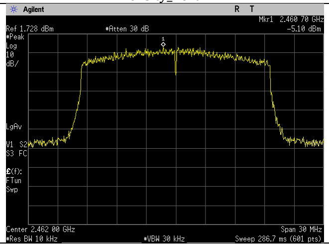
High Ch_2462MHz_20MHz BW_ax-mode_Spectral Density_Port 2
