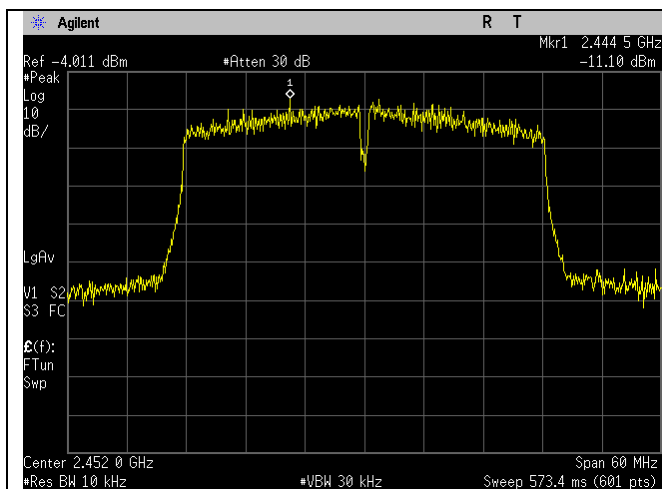
High Ch_2452MHz_40MHz BW_n-mode_Spectral Density_Port 1
