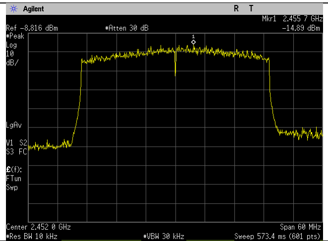
High Ch_2452MHz_40MHz BW_ax-mode_Spectral Density_Port 2
