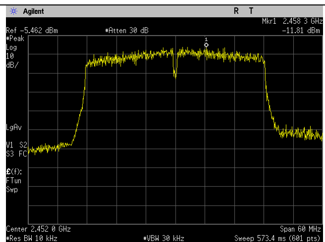
High Ch_2452MHz_40MHz BW_n-mode_Spectral Density_Port 2
