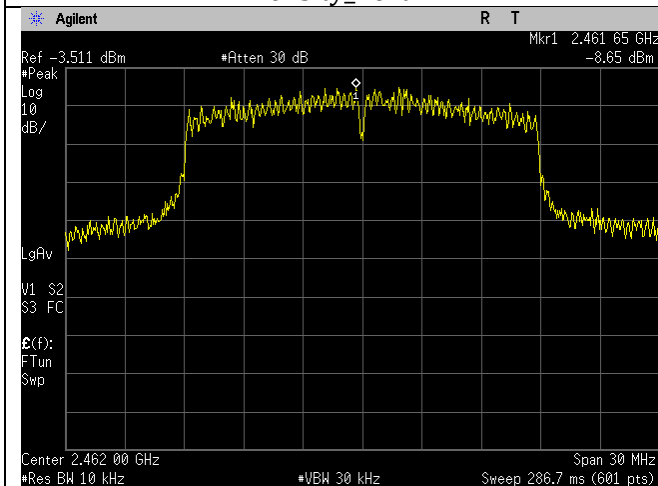
High Ch_2462MHz_20MHz BW_n-mode_Spectral Density_Port 1
