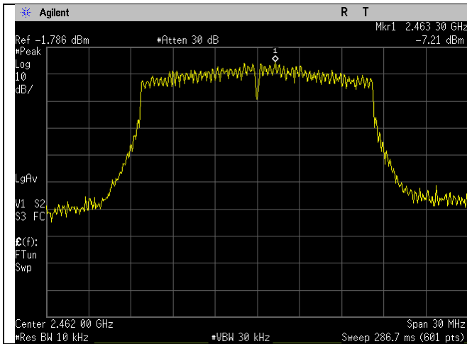
High Ch_2462MHz_20MHz BW_g-mode_Spectral Density_Port 1
