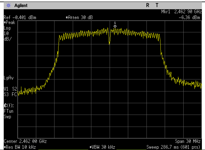
High Ch_2462MHz_20MHz BW_g-mode_Spectral Density_Port 2
