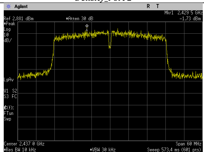
Mid Ch_2437MHz_40MHz BW_n-mode_Spectral Density_Port 2
