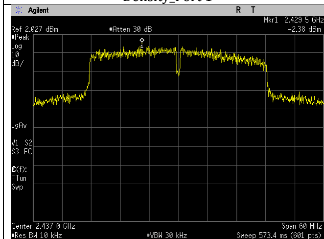
Mid Ch_2437MHz_40MHz BW_n-mode_Spectral Density_Port 1
