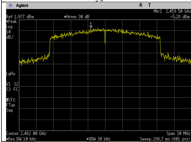
High Ch_2462MHz_20MHz BW_ax-mode_Spectral Density_Port 1
