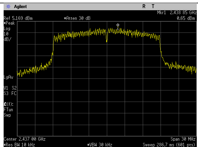
Mid Ch_2437MHz_20MHz BW_n-mode_Spectral Density_Port 2
