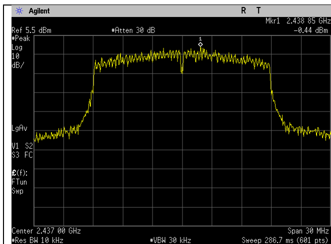
Mid Ch_2437MHz_20MHz BW_n-mode_Spectral Density_Port 1
