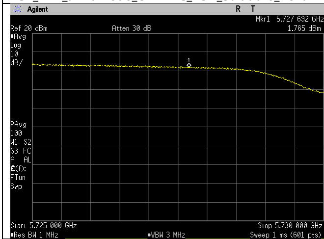
Ch_144_ax40mode_UNII-3_PSD_Straddle_Port 1
