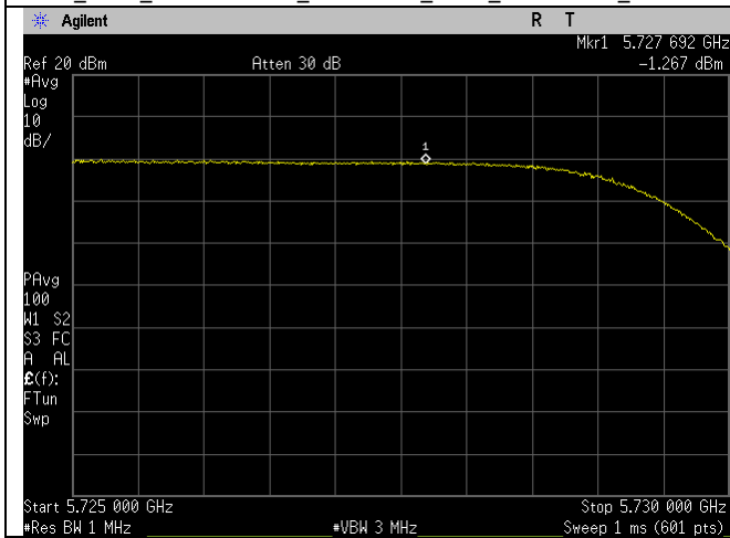
Ch_144_ax80mode_UNII-3_PSD_Straddle_Port 1
