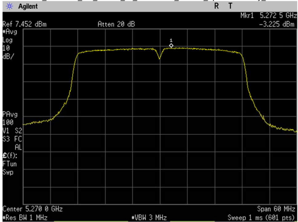
U-NII-2A_5270MHz_low_Mid Ch_54_40MHz BW_n-mode_Spectral Density_Port 2
