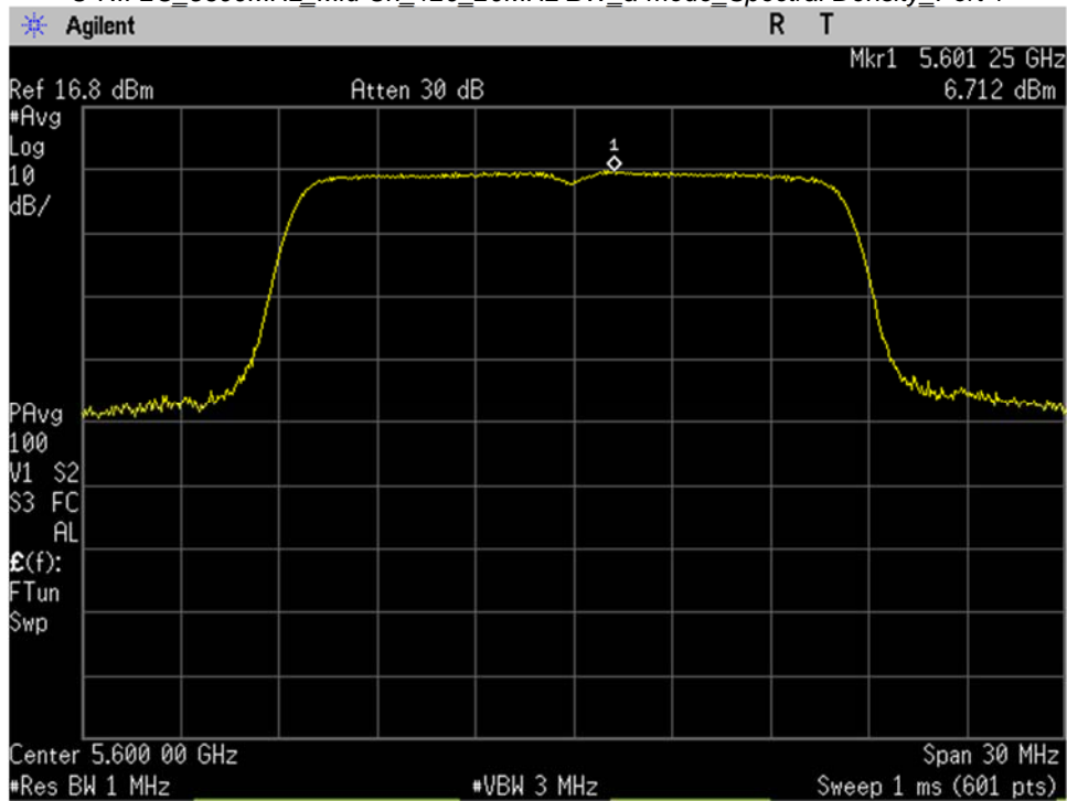
U-NII-2C_5600MHz_Mid Ch_120_20MHz BW_a-mode_Spectral Density_Port 1
