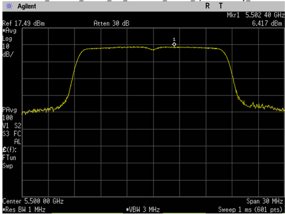
U-NII-2C_5500MHz_Low Ch_100_20MHz BW_a-mode_Spectral Density_Port 1
