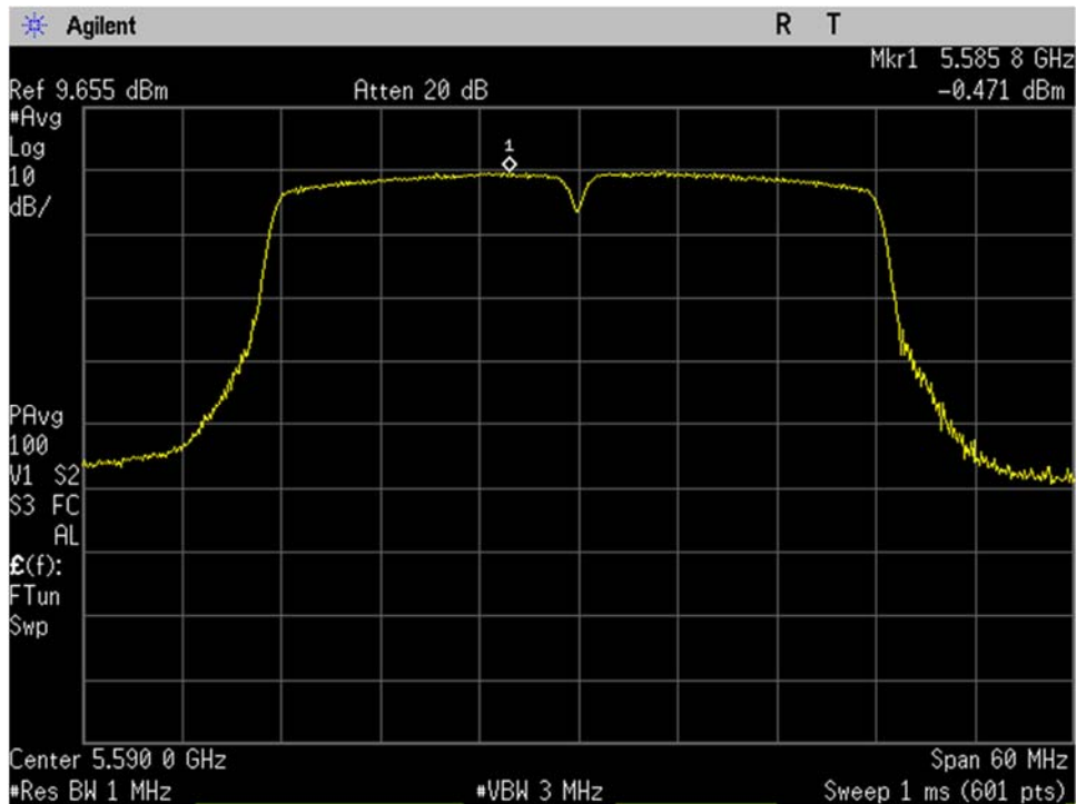
U-NII-2C_5590MHz_Mid Ch_118_40MHz BW_n-mode_Spectral Density_Port 2
