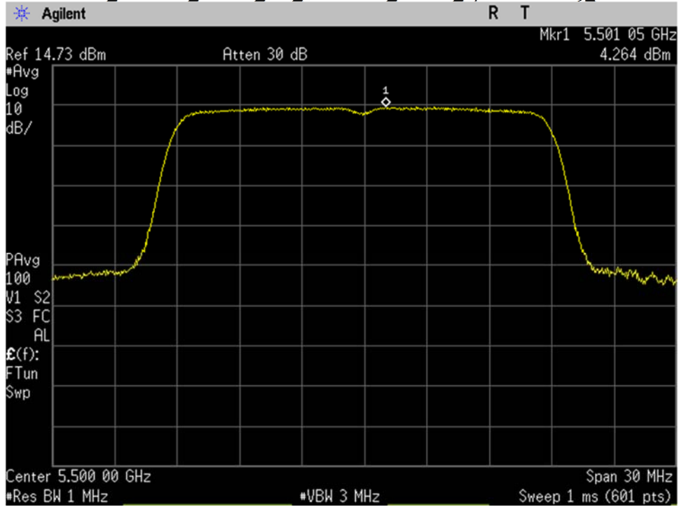
U-NII-2C_5500MHz_Low Ch_100_20MHz BW_n-mode_Spectral Density_Port 1
