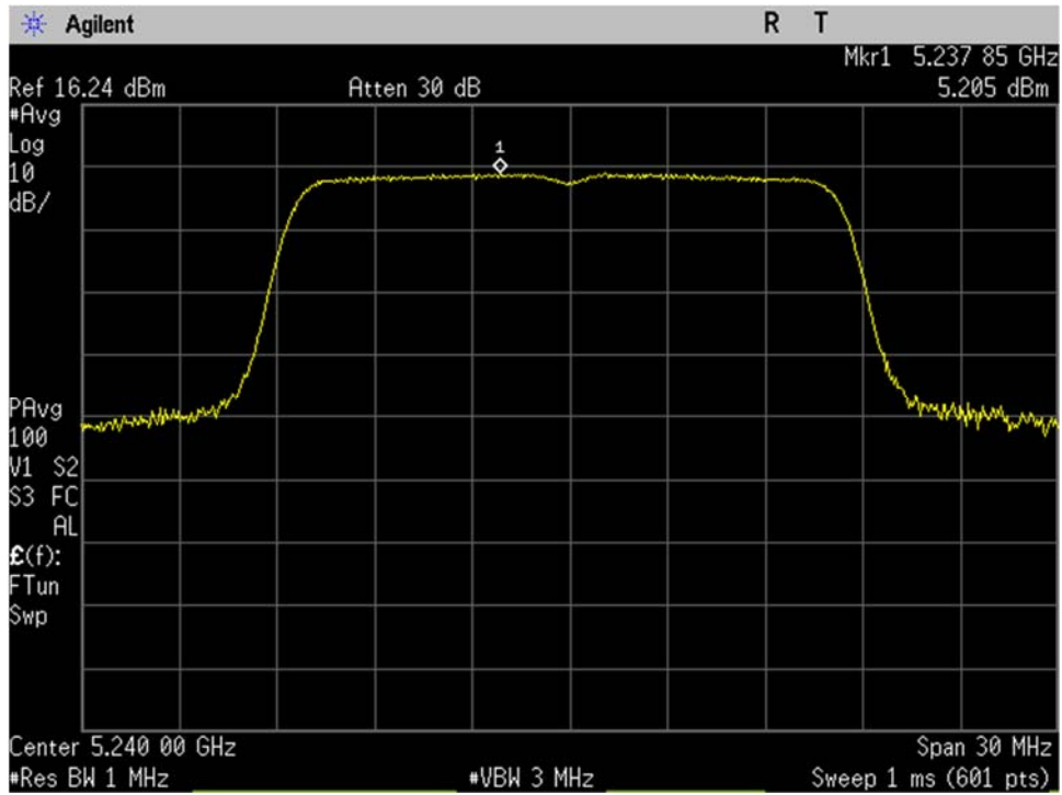
U-NII-1_5240MHz_high_mid Ch_48_20MHz BW_a-mode_Spectral Density_Port 2
