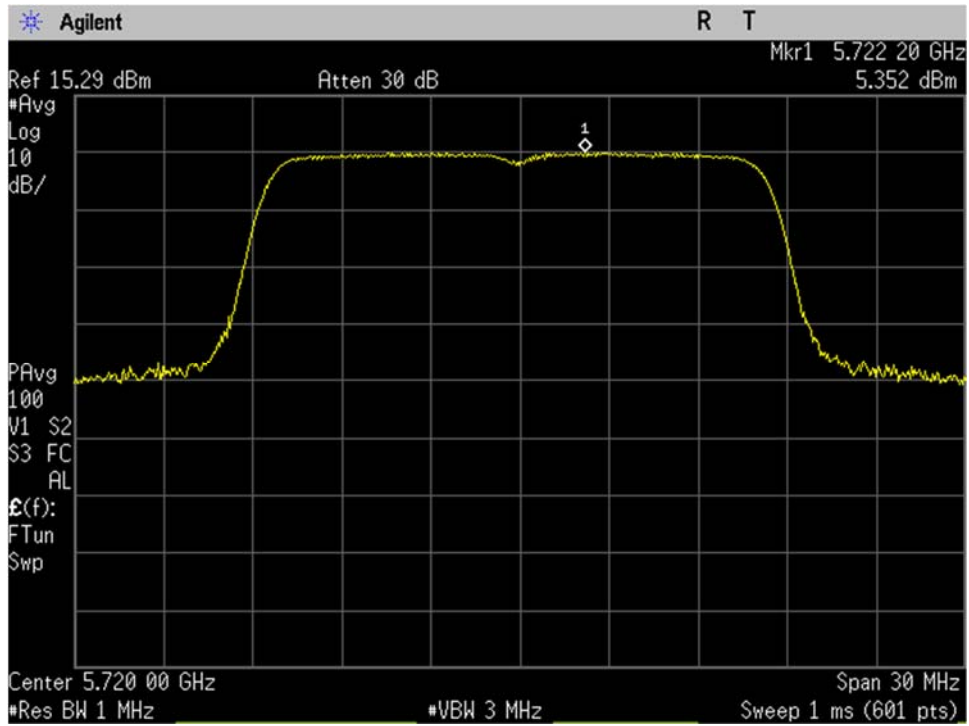
U-NII-2C_5720MHz_High Ch_144_20MHz BW_a-mode_Spectral Density_Port 1
