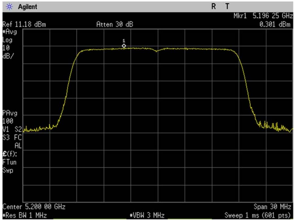
U-NII-1_5200MHz_low_Mid Ch_40_20MHz BW_n-mode_Spectral Density_Port 1
