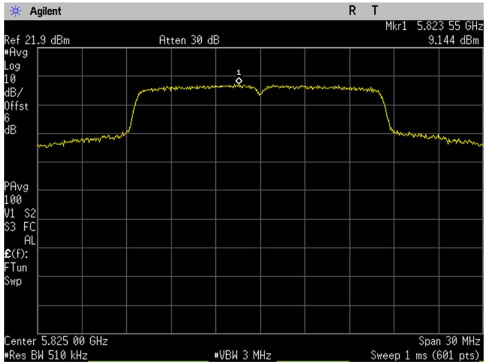
U-NII-3_5825MHz_High Ch_165_20MHz BW_a-mode_Spectral Density_Port 1
