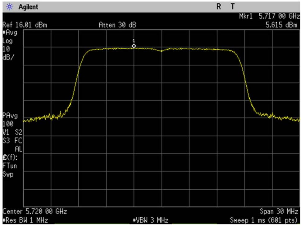
U-NII-2C_5720MHz_High Ch_144_20MHz BW_a-mode_Spectral Density_Port 2
