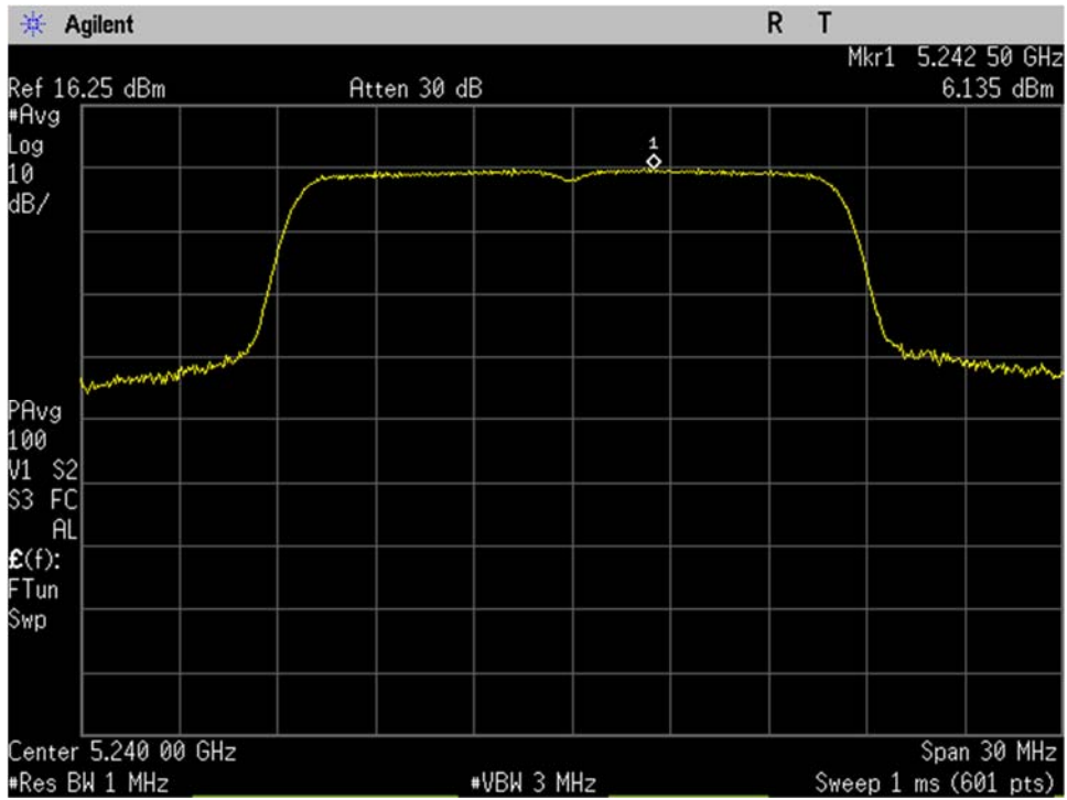
U-NII-1_5240MHz_high_mid Ch_48_20MHz BW_a-mode_Spectral Density_Port 1
