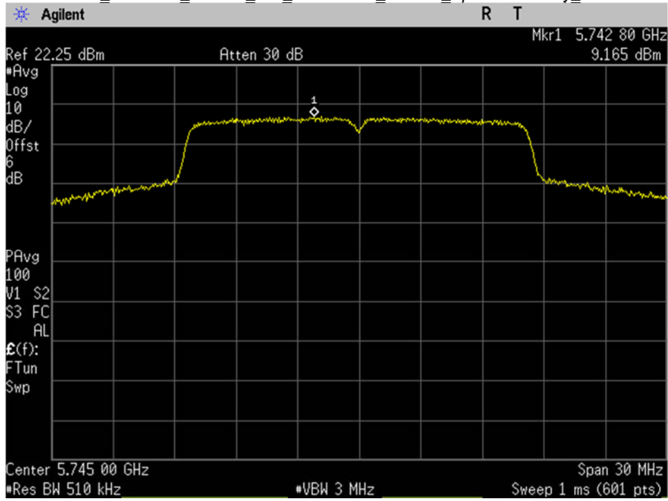
U-NII-3_5745MHz_Low Ch_149_20MHz BW_a-mode_Spectral Density_Port 1
