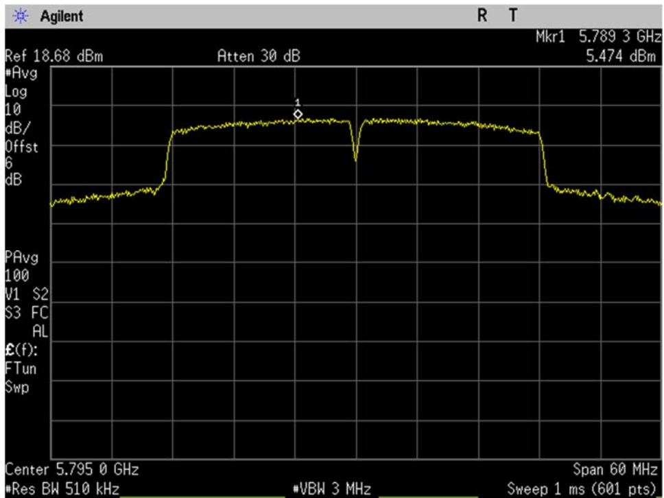
U-NII-3_5795MHz_High_Mid Ch_159_40MHz BW_n-mode_Spectral Density_Port 2
