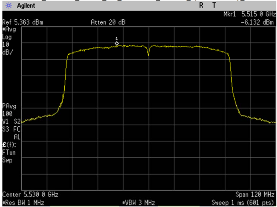
U-NII-2C_5530MHz_Low Ch_106_80MHz BW_ac-mode_Spectral Density_Port 1
