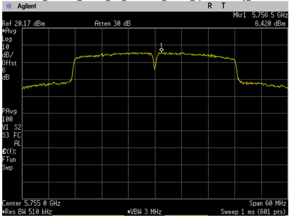
U-NII-3_5755MHz_Low Ch_151_40MHz BW_n-mode_Spectral Density_Port 2
