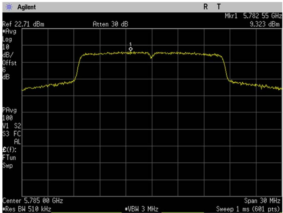
U-NII-3_5785MHz_Mid Ch_157_20MHz BW_a-mode_Spectral Density_Port 2
