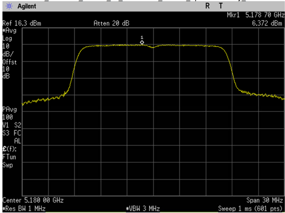
U-NII-1_5180MHz_Low Ch_36_20MHz BW_a-mode_Spectral Density_Port 1
