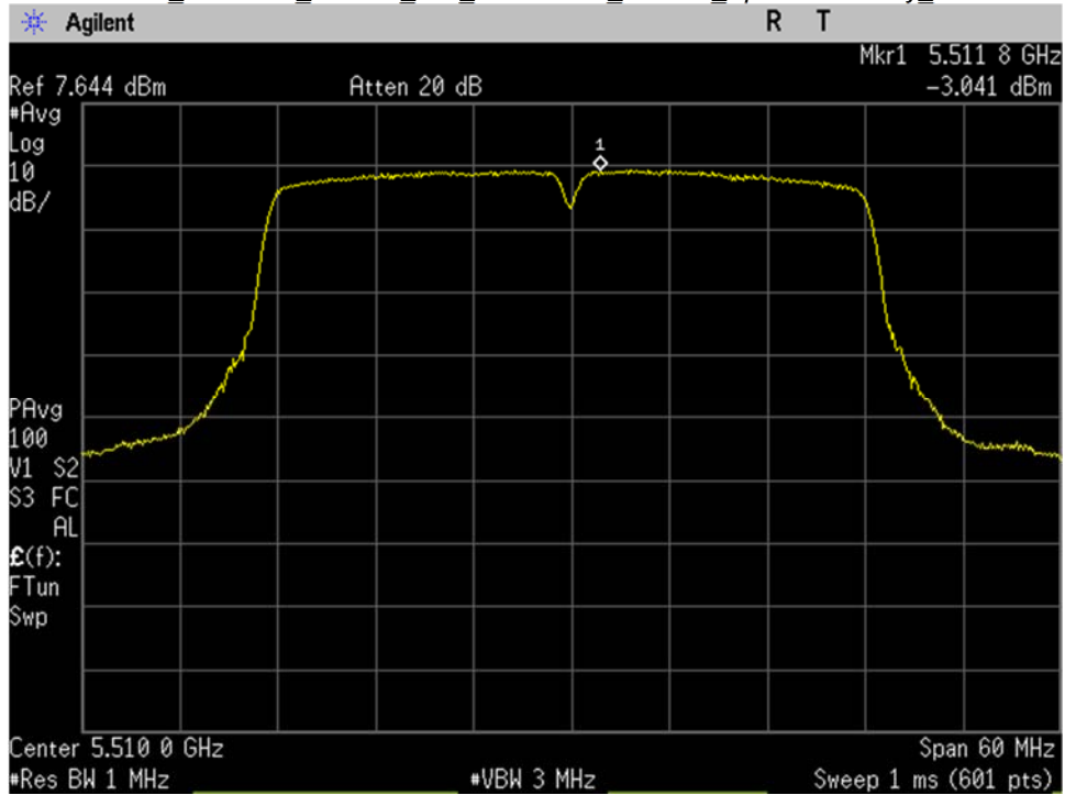
U-NII-2C_5510MHz_Low Ch_102_40MHz BW_n-mode_Spectral Density_Port 1
