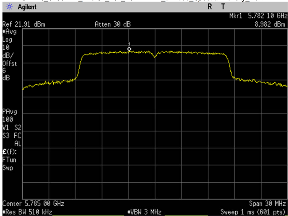
U-NII-3_5785MHz_Mid Ch_157_20MHz BW_a-mode_Spectral Density_Port 1
