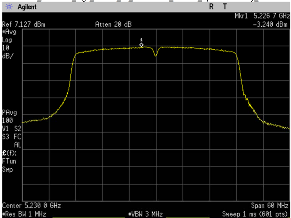
U-NII-1_5230MHz_high_Mid Ch_46_40MHz BW_n-mode_Spectral Density_Port 2
