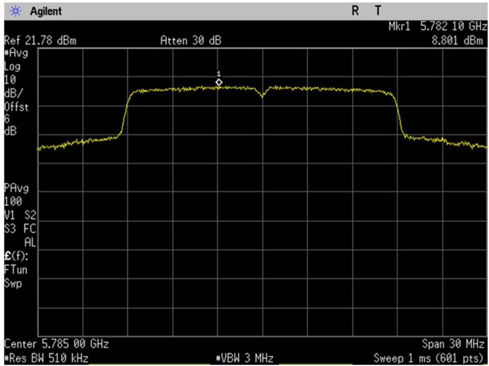
U-NII-3_5785MHz_Mid Ch_157_20MHz BW_n-mode_Spectral Density_Port 2
