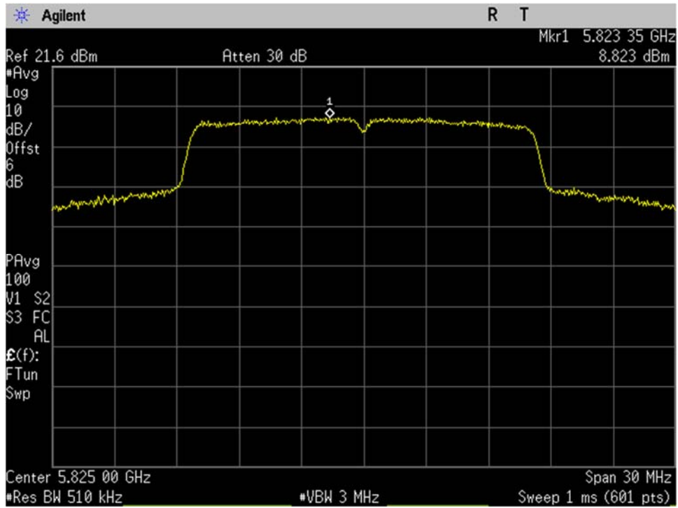
U-NII-3_5825MHz_High Ch_165_20MHz BW_a-mode_Spectral Density_Port 2
