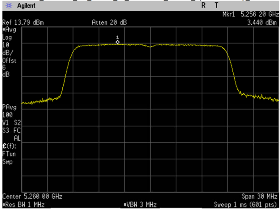
U-NII-2A_5260MHz_low_mid Ch_52_20MHz BW_n-mode_Spectral Density_Port 1
