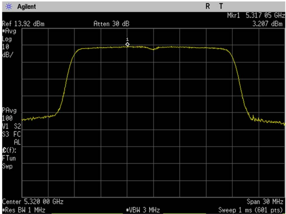
U-NII-2A_5320MHz_High_Ch_64_20MHz BW_n-mode_Spectral Density_Port 2
