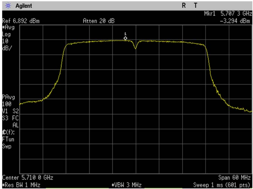
U-NII-2C_5710MHz_High Ch_142_40MHz BW_n-mode_Spectral Density_Port 1
