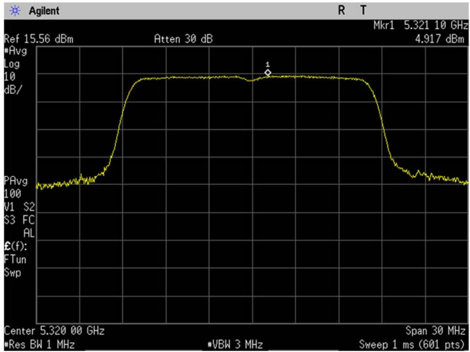
U-NII-2A_5320MHz_High Ch_64_20MHz BW_a-mode_Spectral Density_Port 1
