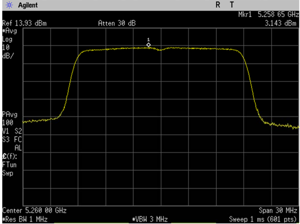
U-NII-2A_5260MHz_low_mid Ch_52_20MHz BW_n-mode_Spectral Density_Port 2
