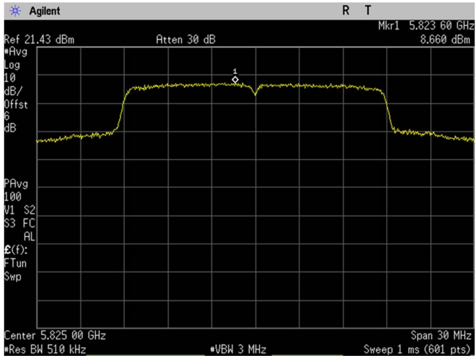
U-NII-3_5825MHz_High Ch_165_20MHz BW_n-mode_Spectral Density_Port 1
