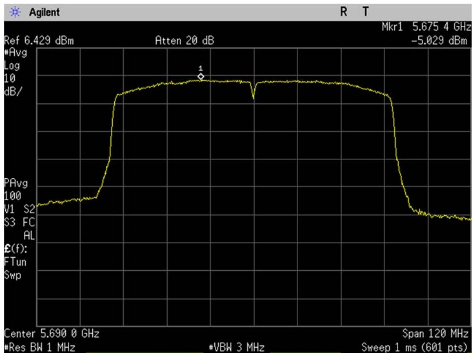
U-NII-2C_5690MHz_High Ch_138_80MHz BW_ac-mode_Spectral Density_Port 2
