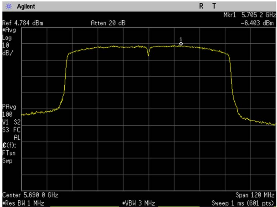
U-NII-2C_5690MHz_High Ch_138_80MHz BW_ac-mode_Spectral Density_Port 1
