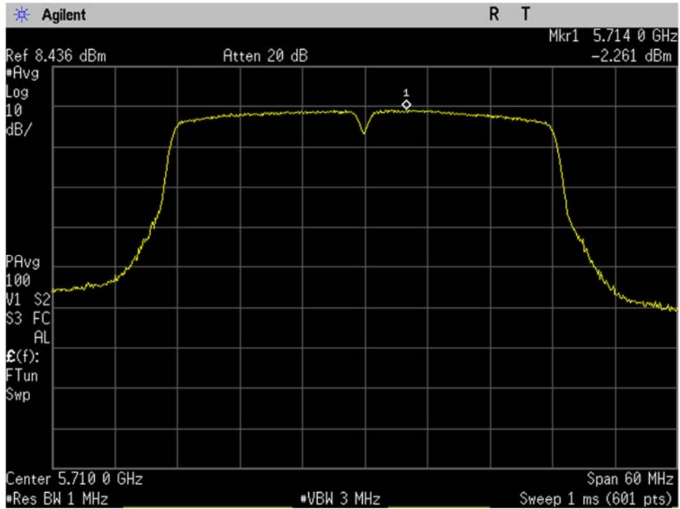
U-NII-2C_5710MHz_High Ch_142_40MHz BW_n-mode_Spectral Density_Port 2
