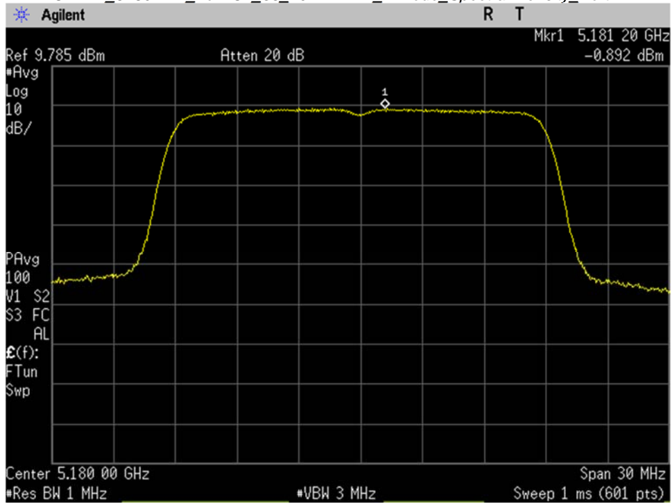
U-NII-1_5180MHz_Low Ch_36_20MHz BW_n-mode_Spectral Density_Port 2
