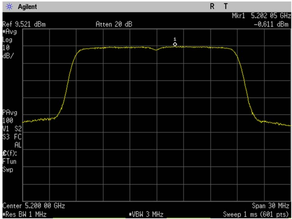
U-NII-1_5200MHz_low_Mid Ch_40_20MHz BW_n-mode_Spectral Density_Port 2
