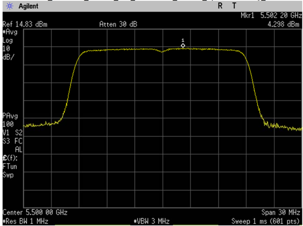
U-NII-2C_5500MHz_Low Ch_100_20MHz BW_n-mode_Spectral Density_Port 2
