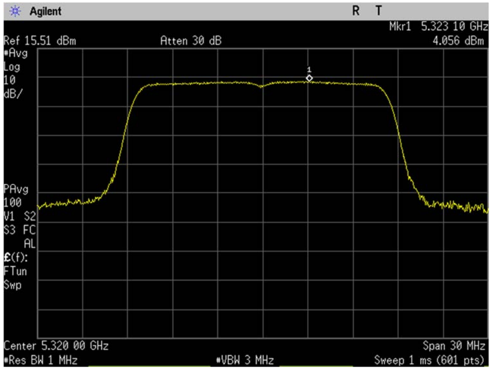
U-NII-2A_5320MHz_High Ch_64_20MHz BW_a-mode_Spectral Density_Port 2
