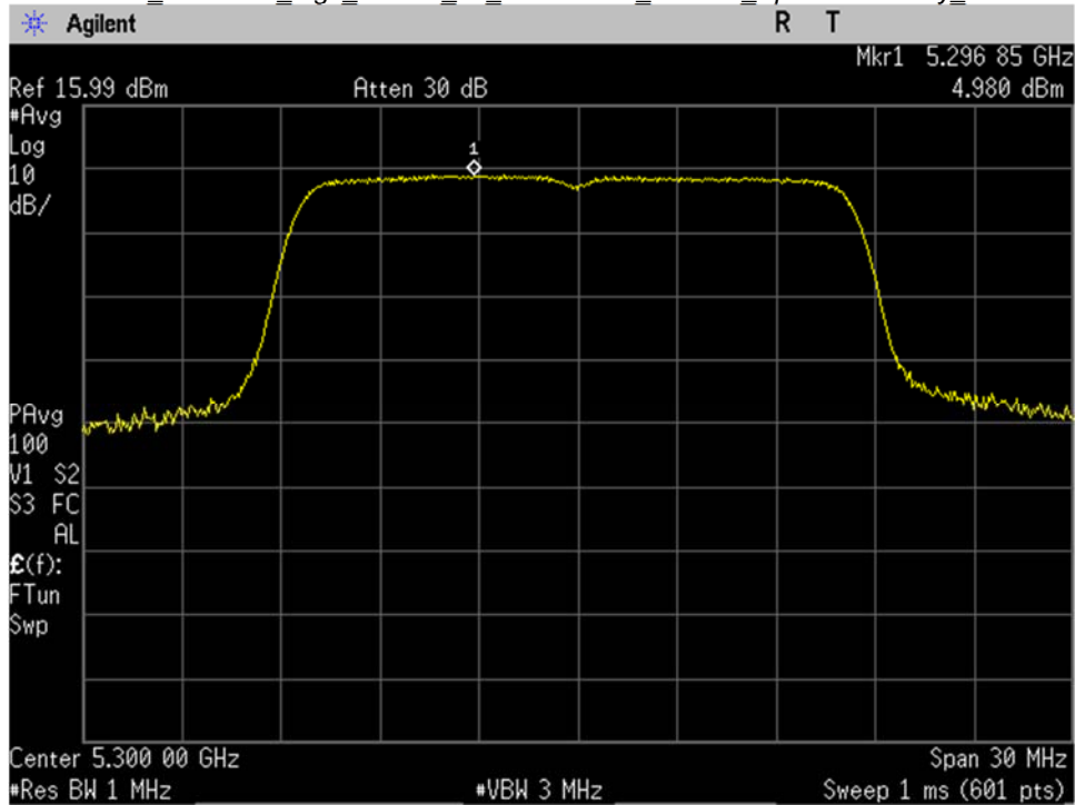
U-NII-2A_5300MHz_high_Mid Ch_60_20MHz BW_a-mode_Spectral Density_Port 1
