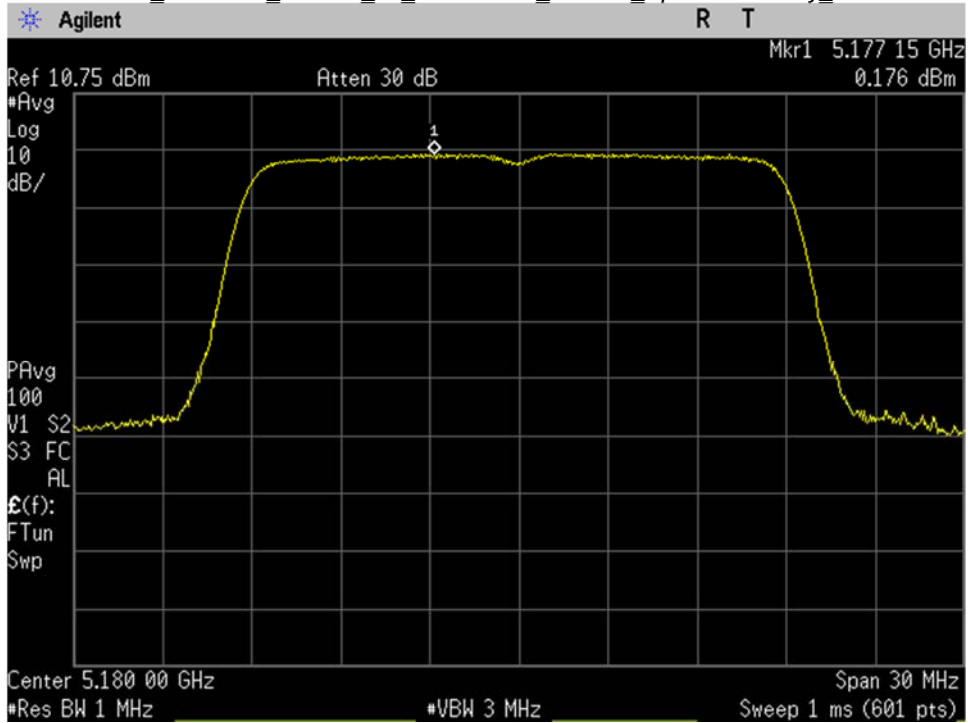
U-NII-1_5180MHz_Low Ch_36_20MHz BW_n-mode_Spectral Density_Port 1
