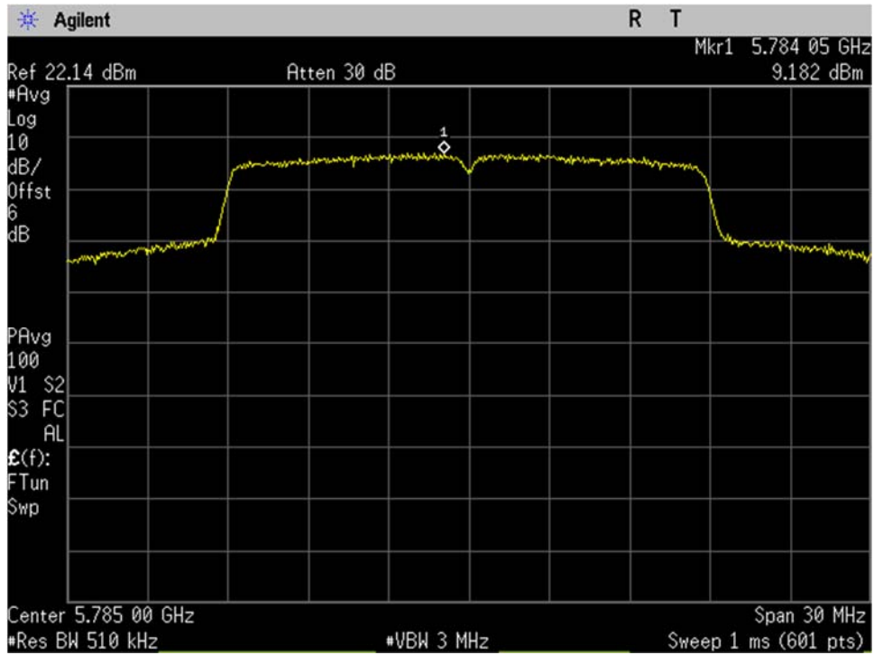
U-NII-3_5785MHz_Mid Ch_157_20MHz BW_n-mode_Spectral Density_Port 1
