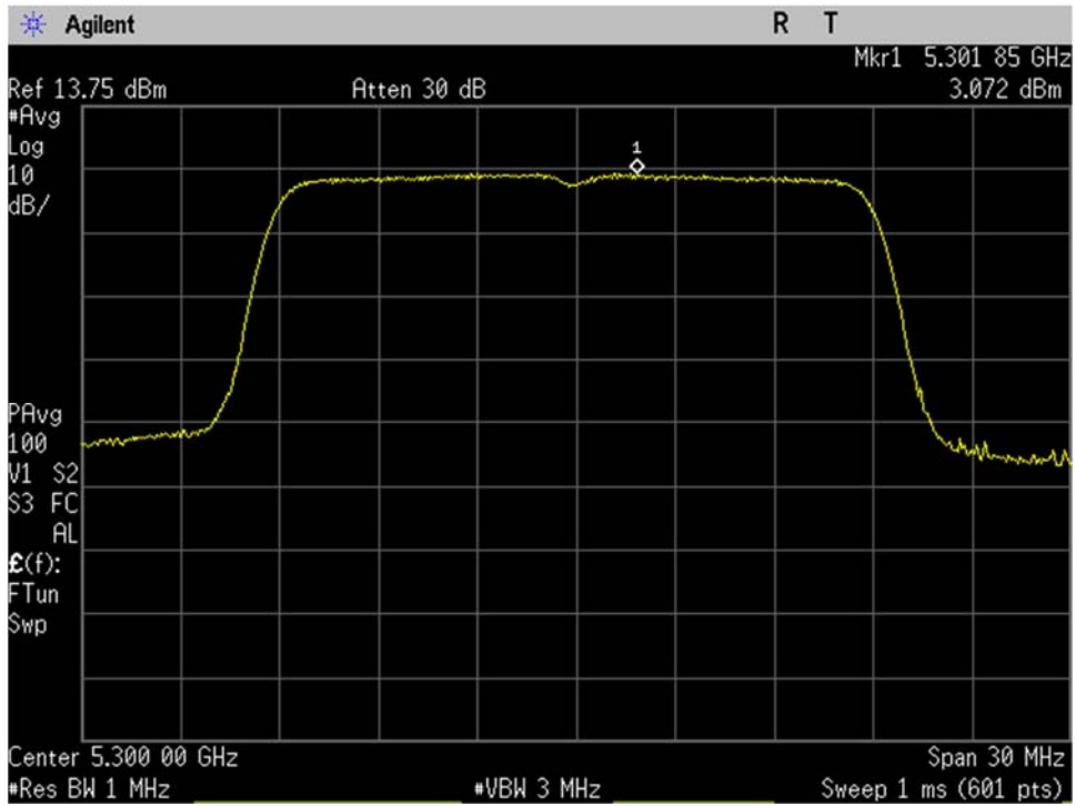
U-NII-2A_5300MHz_high_Mid_Ch_60_20MHz BW_n-mode_Spectral Density_Port 2
