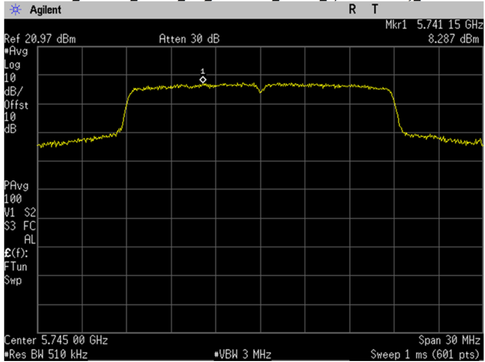
U-NII-3_5745MHz_Low Ch_149_20MHz BW_n-mode_Spectral Density_Port 2
