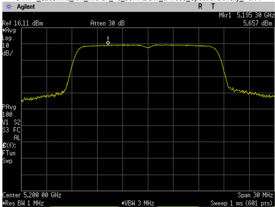
U-NII-1_5200MHz_low_Mid Ch_40_20MHz BW_a-mode_Spectral Density_Port 1
