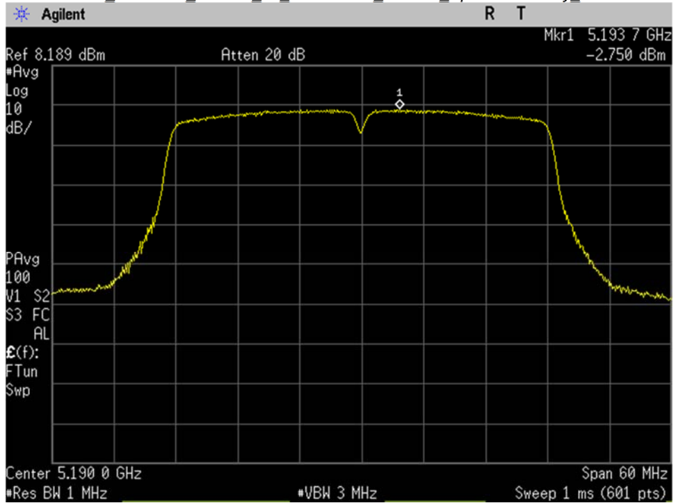
U-NII-1_5190MHz_Low Ch_38_40MHz BW_n-mode_Spectral Density_Port 1
