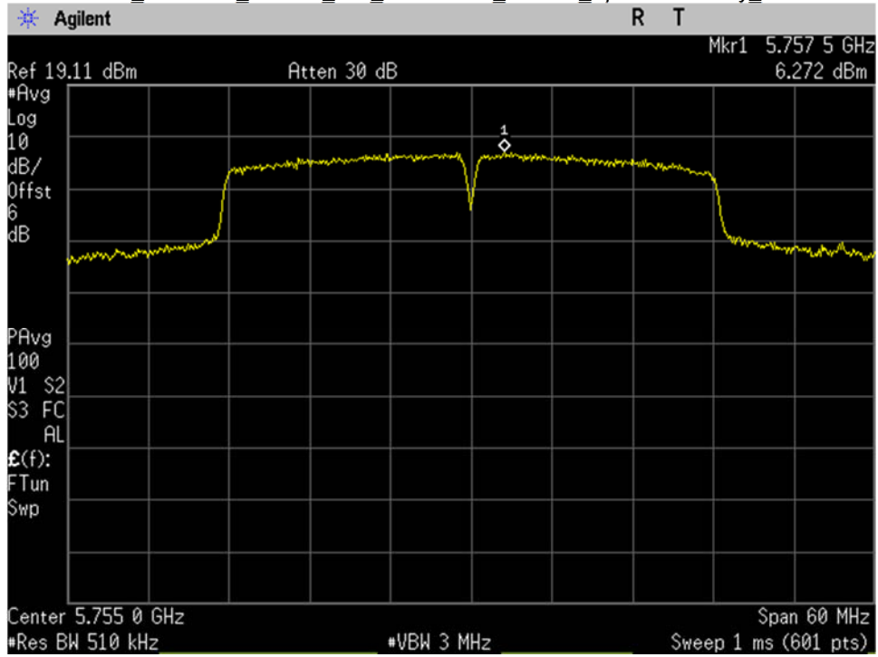
U-NII-3_5755MHz_Low Ch_151_40MHz BW_n-mode_Spectral Density_Port 1
