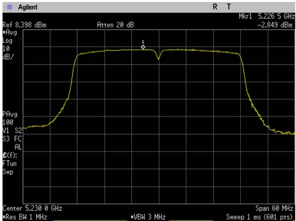
U-NII-1_5230MHz_high_Mid Ch_46_40MHz BW_n-mode_Spectral Density_Port 1
