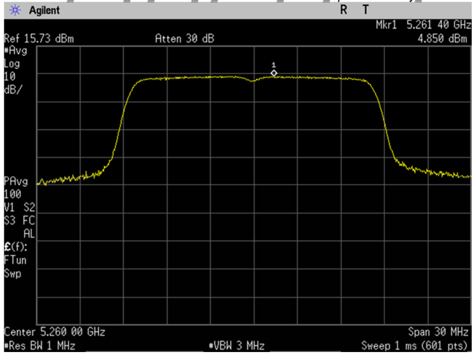
U-NII-2A_5260MHz_low_mid Ch_52_20MHz BW_a-mode_Spectral Density_Port 1
