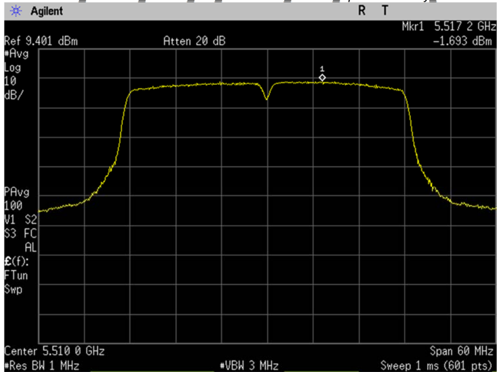
U-NII-2C_5510MHz_Low Ch_102_40MHz BW_n-mode_Spectral Density_Port 2
