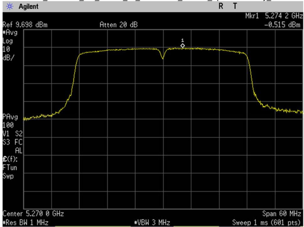
U-NII-2A_5270MHz_low_Mid Ch_54_40MHz BW_n-mode_Spectral Density_Port 1
