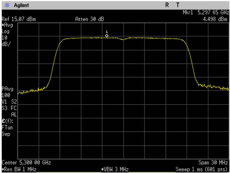
U-NII-2A_5300MHz_high_Mid_Ch_60_20MHz BW_n-mode_Spectral Density_Port 1
