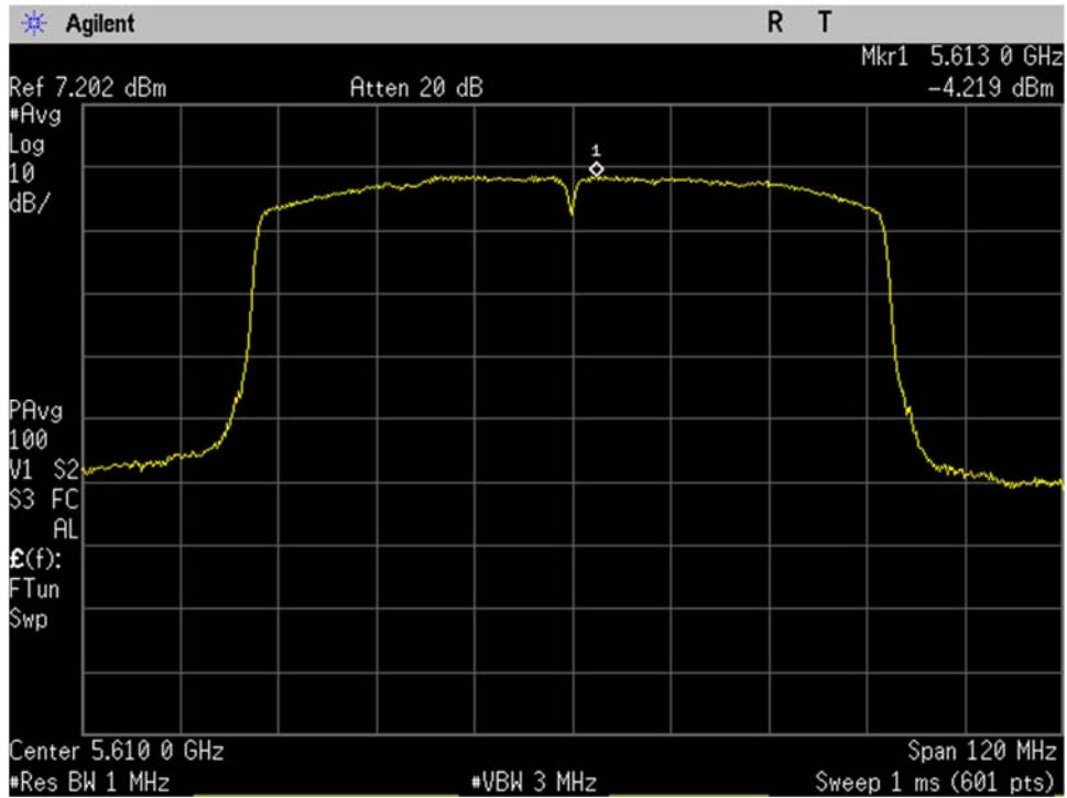
U-NII-2C_5610MHz_Mid Ch_122_80MHz BW_ac-mode_Spectral Density_Port 2
