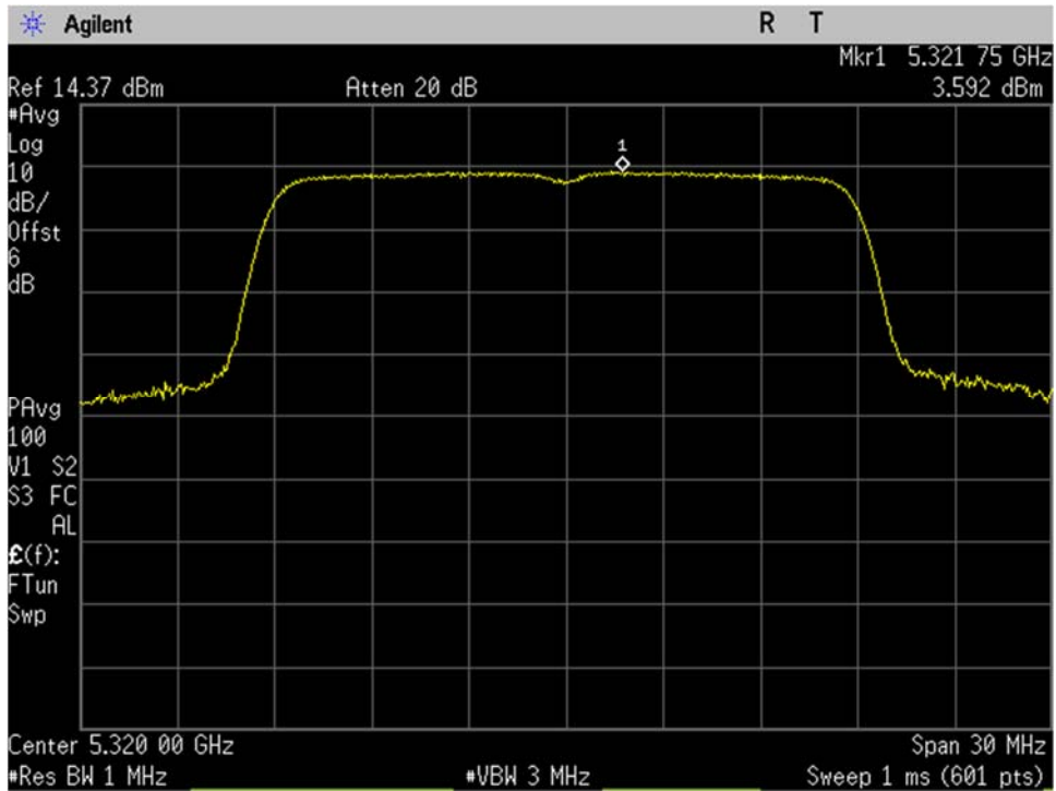
U-NII-2A_5320MHz_High_Ch_64_20MHz BW_n-mode_Spectral Density_Port 1
