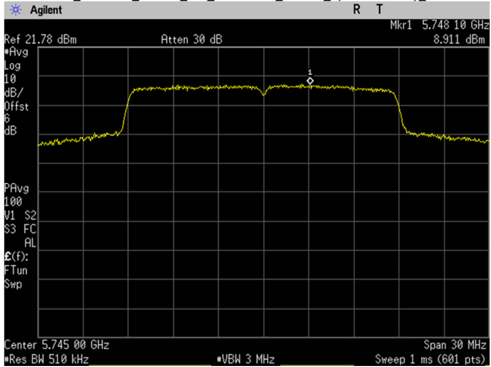
U-NII-3_5745MHz_Low Ch_149_20MHz BW_n-mode_Spectral Density_Port 1
