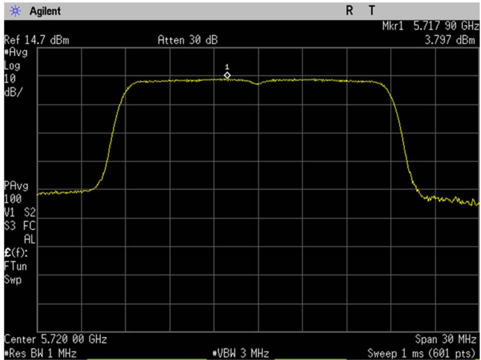
U-NII-2C_5720MHz_High Ch_144_20MHz BW_n-mode_Spectral Density_Port 1
