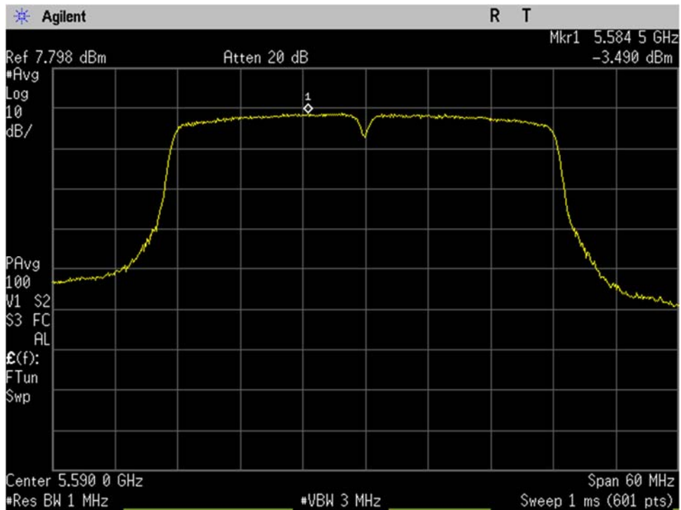
U-NII-2C_5590MHz_Mid Ch_118_40MHz BW_n-mode_Spectral Density_Port 1
