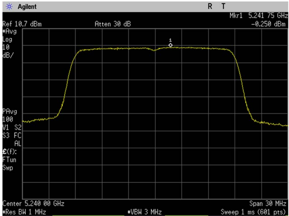
U-NII-1_5240MHz_high_mid Ch_48_20MHz BW_n-mode_Spectral Density_Port 2
