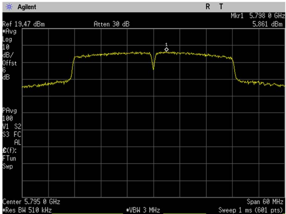
U-NII-3_5795MHz_High_Mid Ch_159_40MHz BW_n-mode_Spectral Density_Port 1
