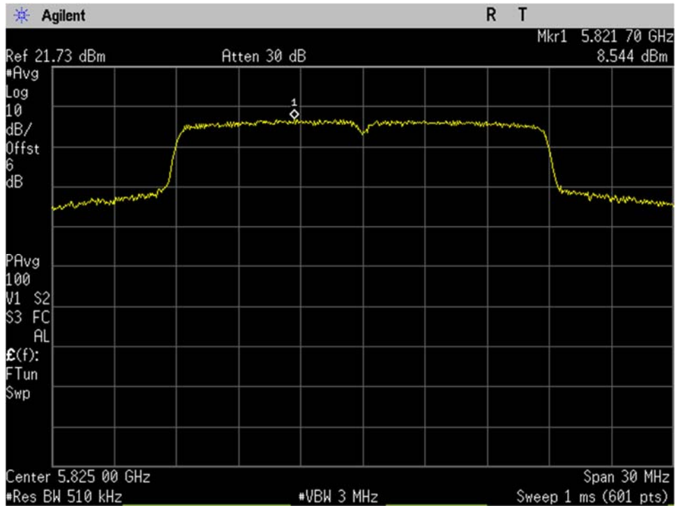
U-NII-3_5825MHz_High Ch_165_20MHz BW_n-mode_Spectral Density_Port 2
