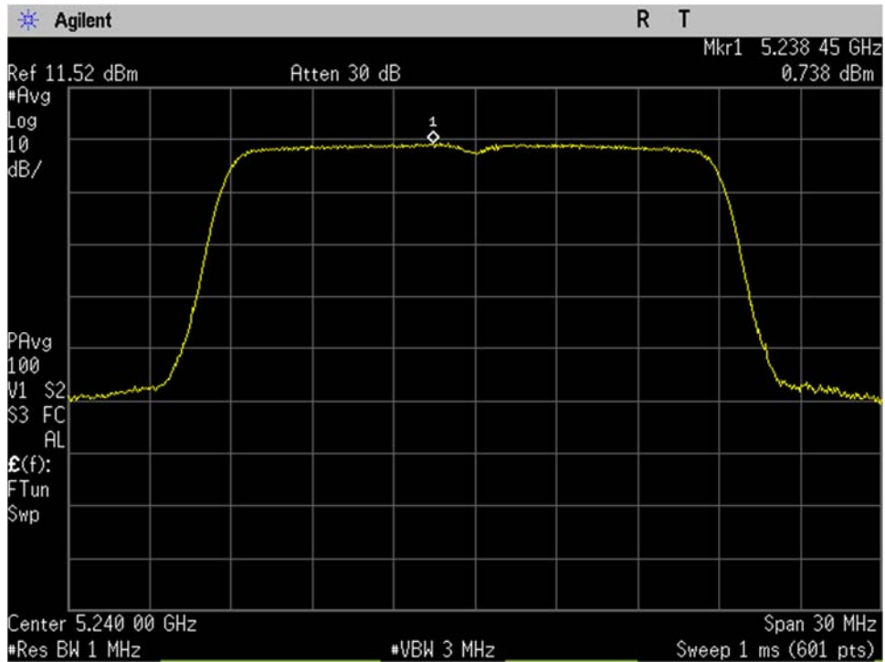
U-NII-1_5240MHz_high_mid Ch_48_20MHz BW_n-mode_Spectral Density_Port 1
