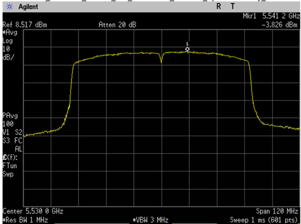
U-NII-2C_5530MHz_Low Ch_106_80MHz BW_ac-mode_Spectral Density_Port 2
