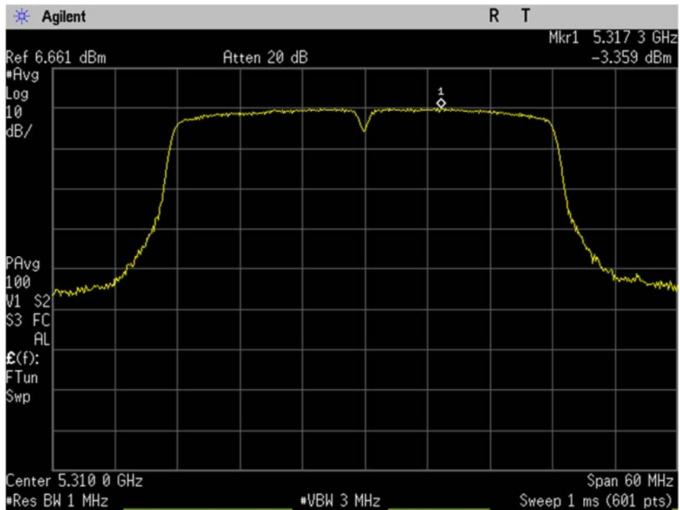
U-NII-2A_5310MHz_High Ch_62_40MHz BW_n-mode_Spectral Density_Port 1
