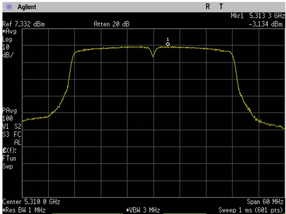
U-NII-2A_5310MHz_High Ch_62_40MHz BW_n-mode_Spectral Density_Port 2
