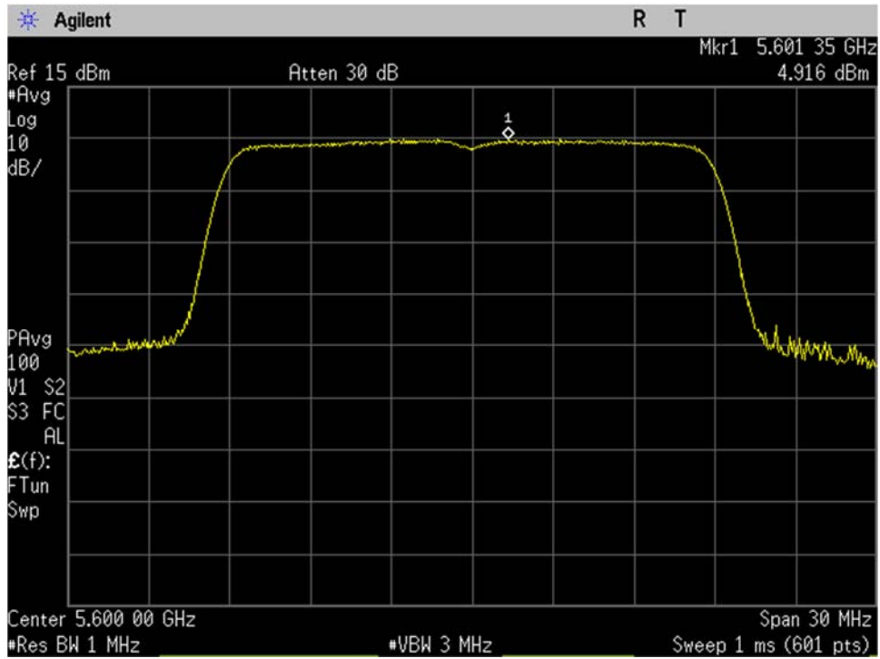
U-NII-2C_5600MHz_Mid Ch_120_20MHz BW_n-mode_Spectral Density_Port 1
