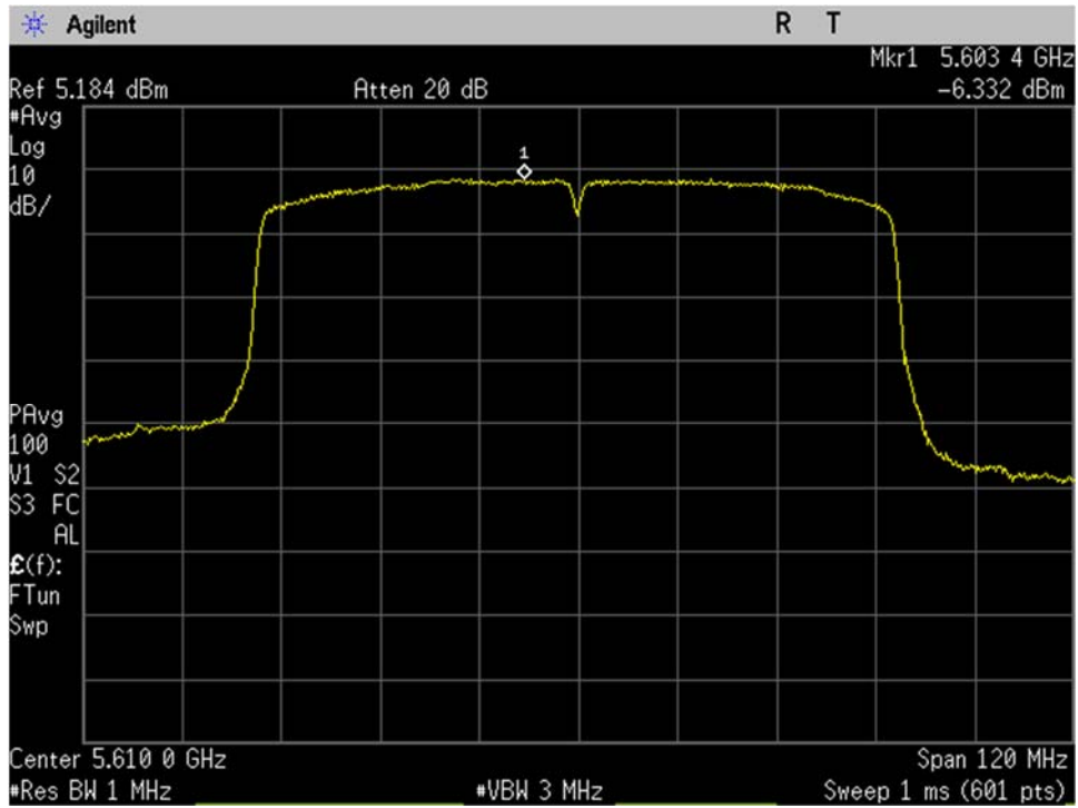
U-NII-2C_5610MHz_Mid Ch_122_80MHz BW_ac-mode_Spectral Density_Port 1
