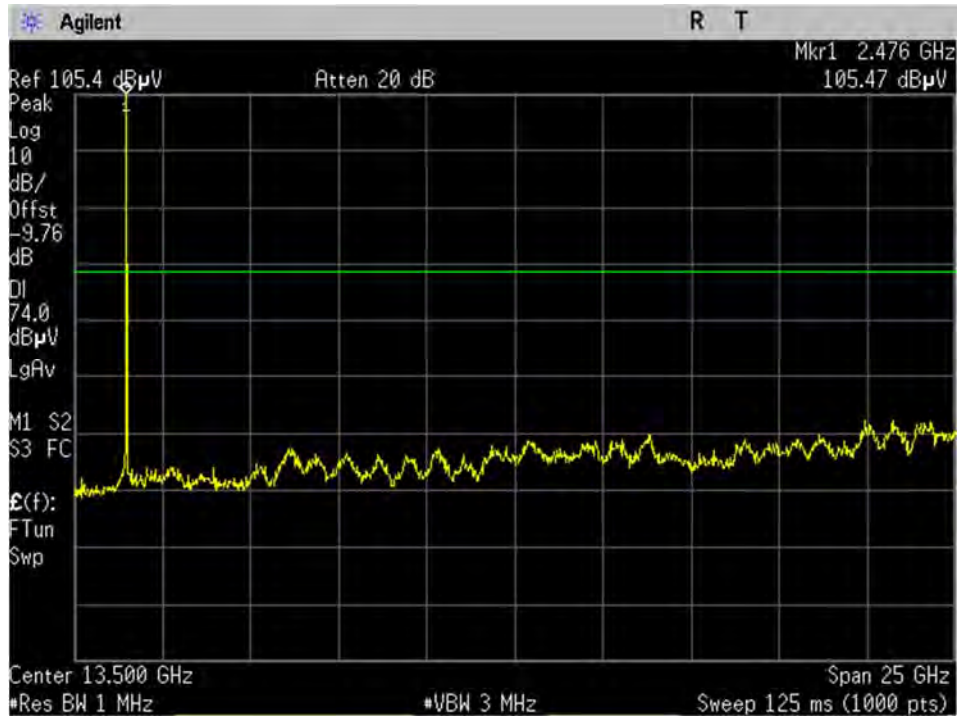
BLE_High Ch_2480MHz_1MBit_15.209_1-26GHz_Peak_Port 1
