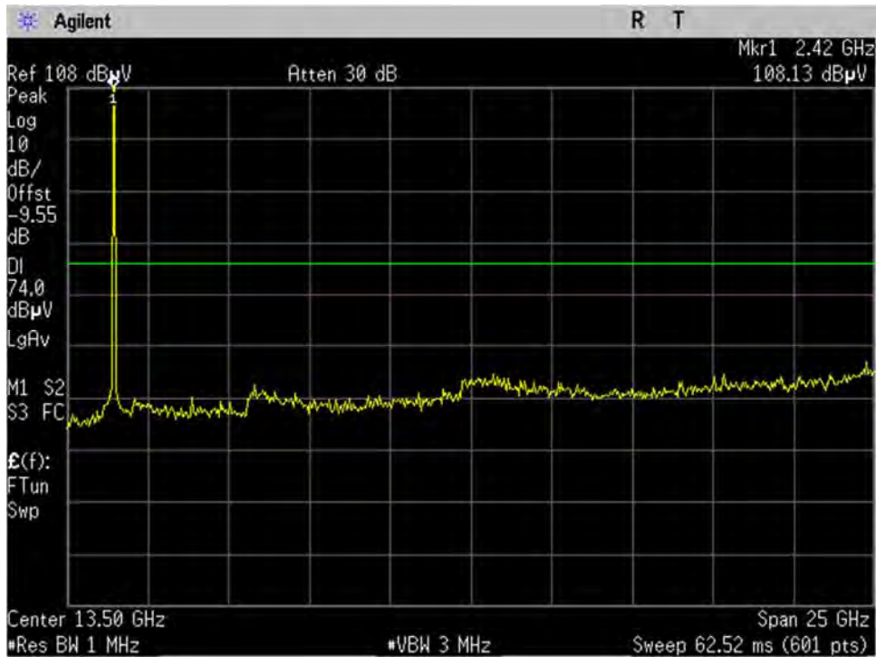
WIFI_Mid Ch_2437MHz_20MHz BW_b-mode_15.209_1-26GHz_Peak_Port 2
