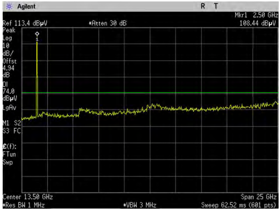
BLE_High Ch_2480MHz_2MBit_15.209_1-26GHz_Peak_Port 1
