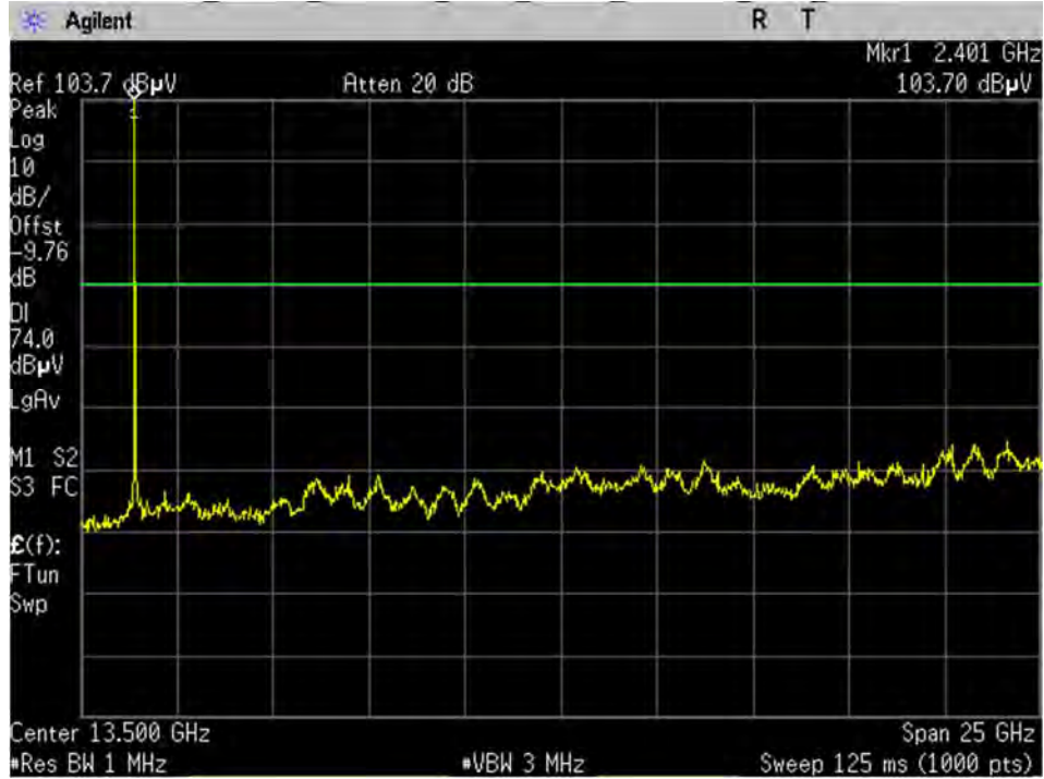
BLE_Low Ch_2402MHz_1MBit_15.209_1-26GHz_Peak_Port 1
