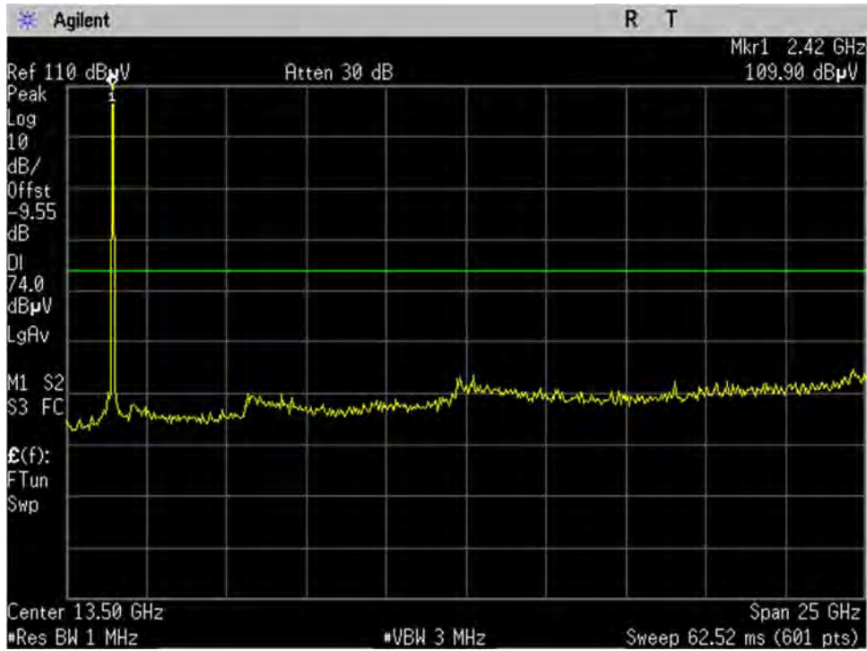
WIFI_Mid Ch_2437MHz_20MHz BW_b-mode_15.209_1-26GHz_Peak_Port 1
