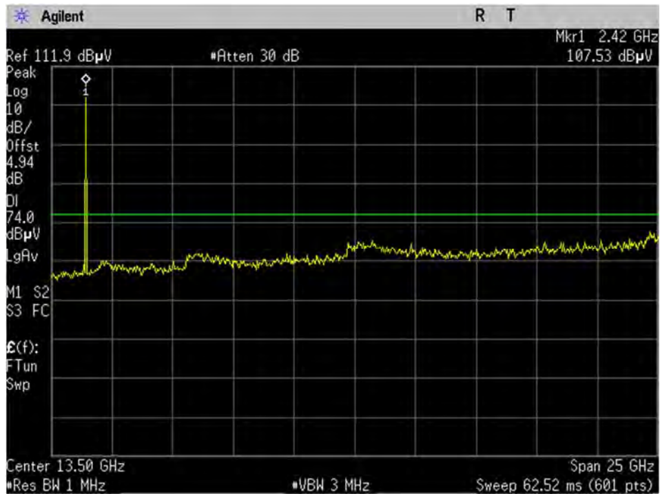
BLE_Low Ch_2402MHz_2MBit_15.209_1-26GHz_Peak_Port 1
