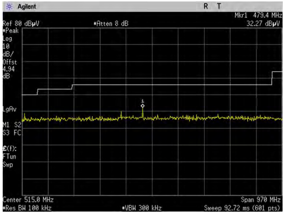
BLE_Mid Ch_2440MHz_2MBit_15.209_30-1000MHz_Peak_Port 1
