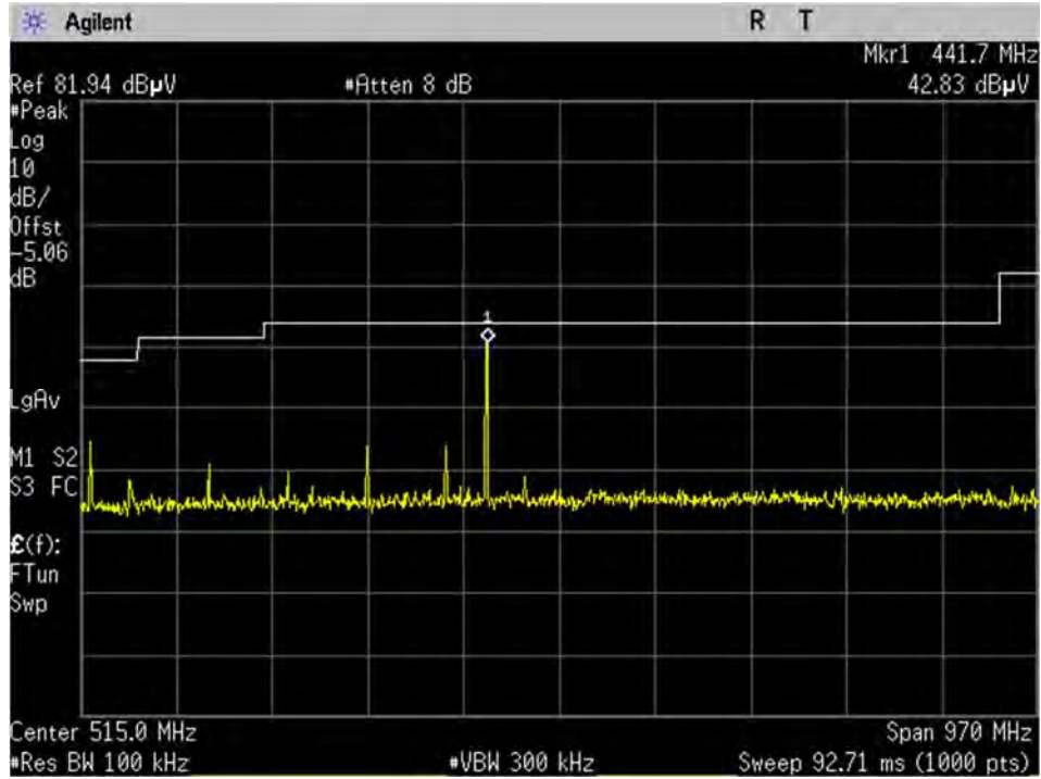
BLE_Low Ch_2402MHz_1MBit_15.209_30-1000MHz_Peak_Port 1
