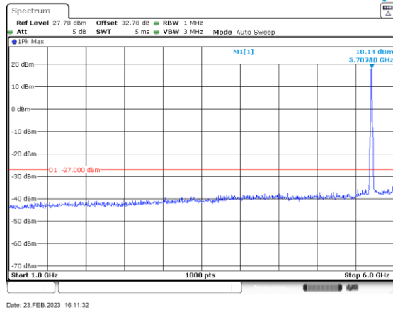
a_5700_1000-6000_Ant A
