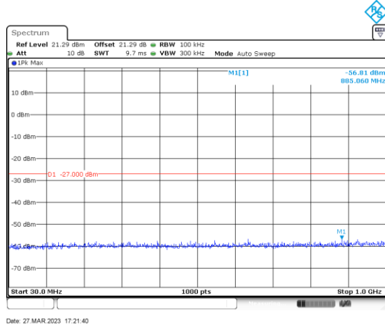
ac80_5610_30-1000_Ant B
