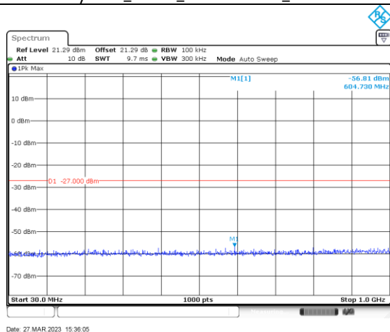
ac/n40_5310_30-1000_Ant B
