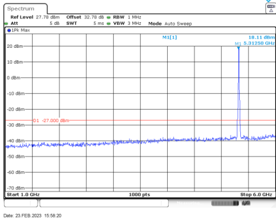
ac/n20_5320_1000-6000_Ant A
