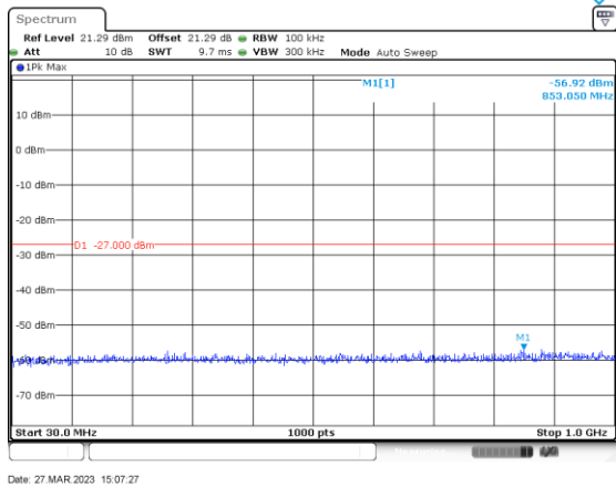
a_5260_30-1000_Ant B
