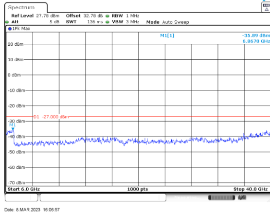
ac/n20_5260_6000-40000_Ant A
