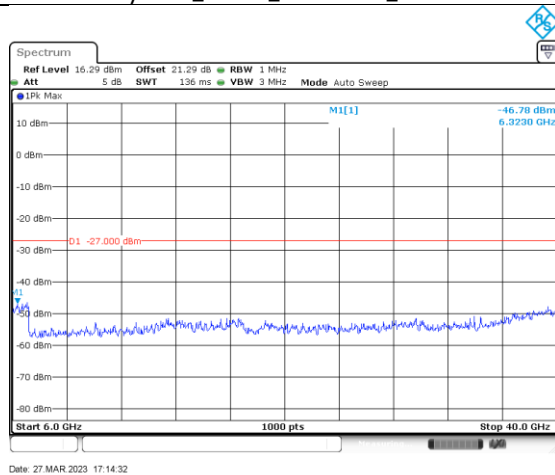
ac/n40_5590_6000-40000_Ant B
