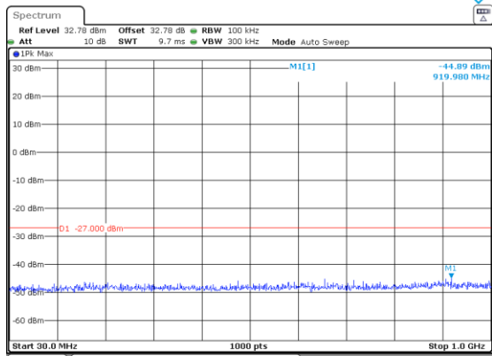
a_5500_30-1000_Ant A
