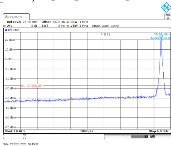
ac/n40_5710_1000-6000_Ant A
