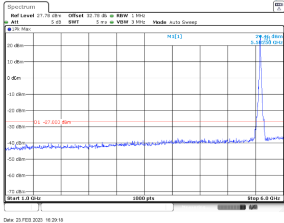
ac/n20_5580_1000-6000_Ant A
