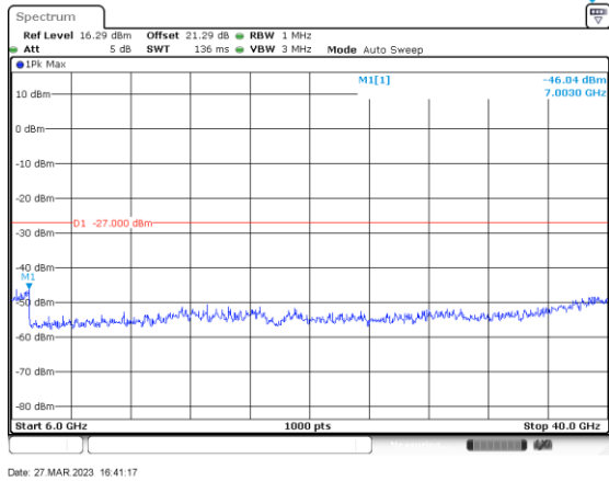
ac80_5290_6000-40000_Ant B
