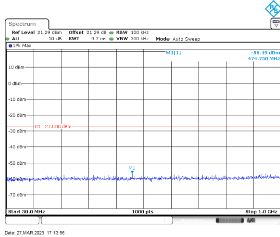
ac/n40_5590_30-1000_Ant B
