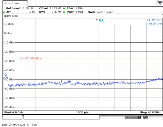
ac/n40_5670_6000-40000_Ant B
