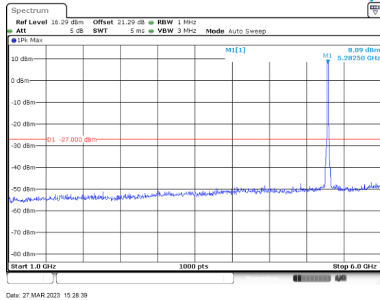
ac/n20_5280_1000-6000_Ant B
