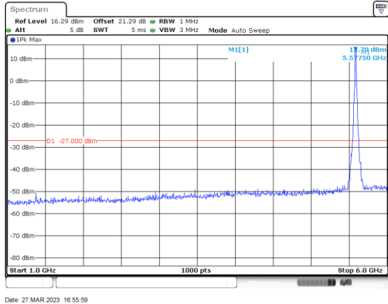
ac/n20_5580_1000-6000_Ant B
