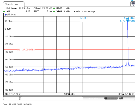
a_5700_1000-6000_Ant B
