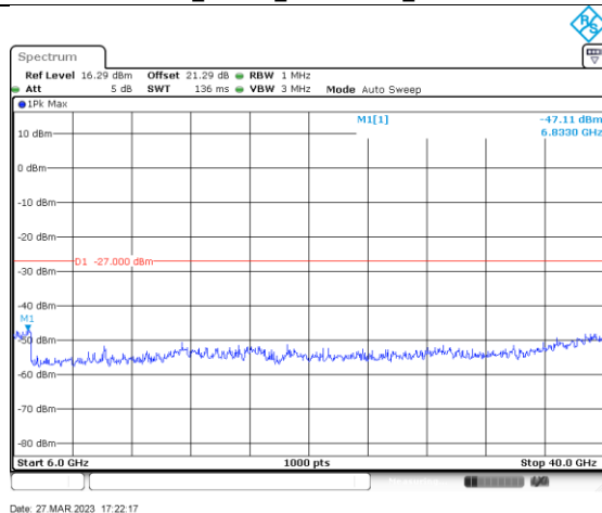
ac80_5610_6000-40000_Ant B
