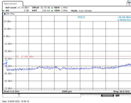
a_5280_6000-40000_Ant A
