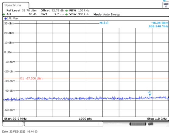
ac80_5530_30-1000_Ant A
