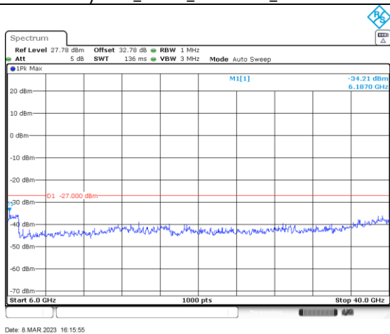
ac/n40_5510_6000-40000_Ant A
