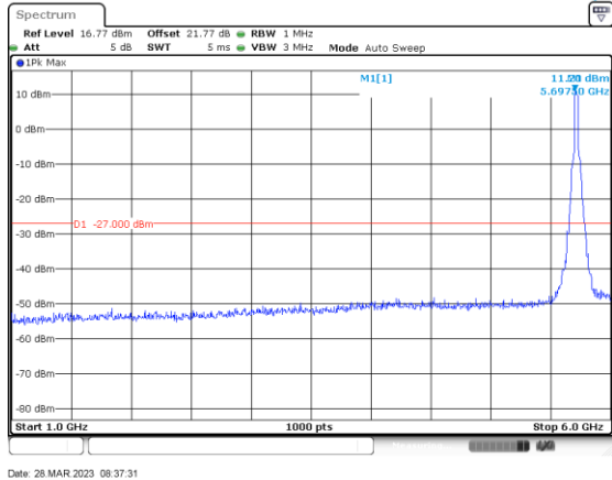
ac/n40_5710_1000-6000_Ant B
