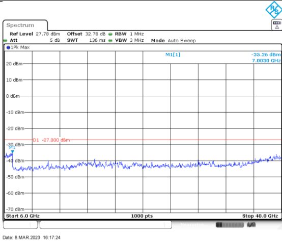
ac80_5690_6000-40000_Ant A
