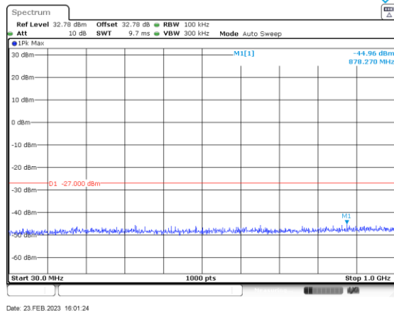
ac/n40_5310_30-1000_Ant A
