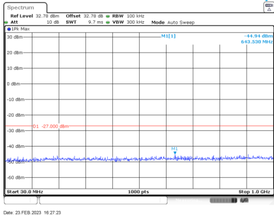
ac/n20_5500_30-1000_Ant A
