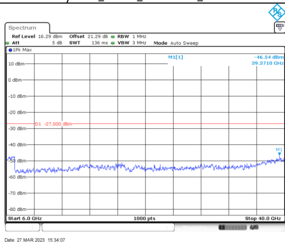
ac/n40_5270_6000-40000_Ant B
