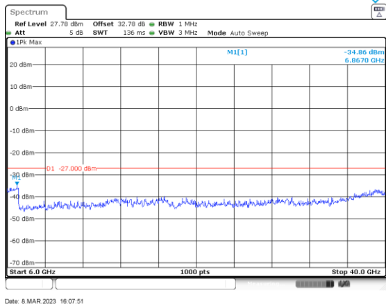
ac/n40_5270_6000-40000_Ant A
