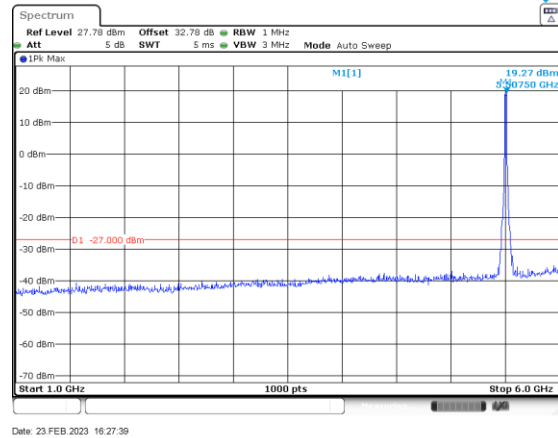
ac/n20_5500_1000-6000_Ant A
