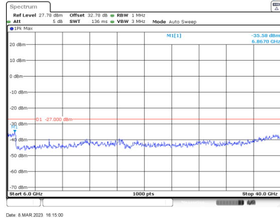
ac/n20_5580_6000-40000_Ant A
