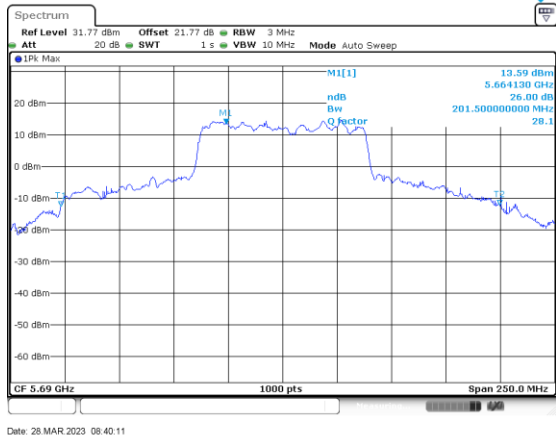
ac80_5690_Ant B
