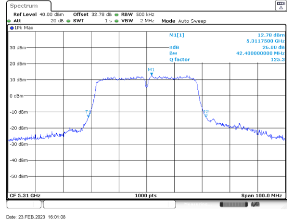
ac/n40_5310_Ant A
