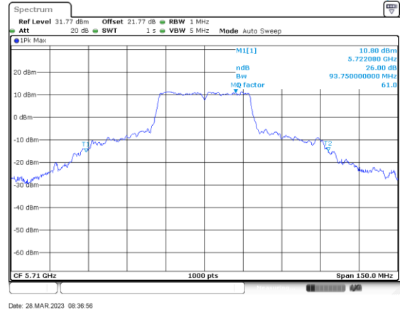
ac/n40_5710_Ant B
