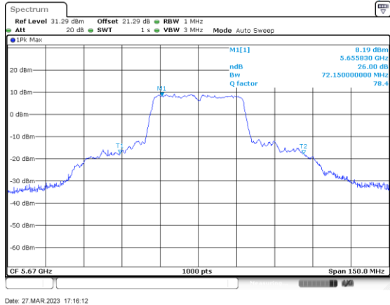
ac/n40_5670_Ant B
