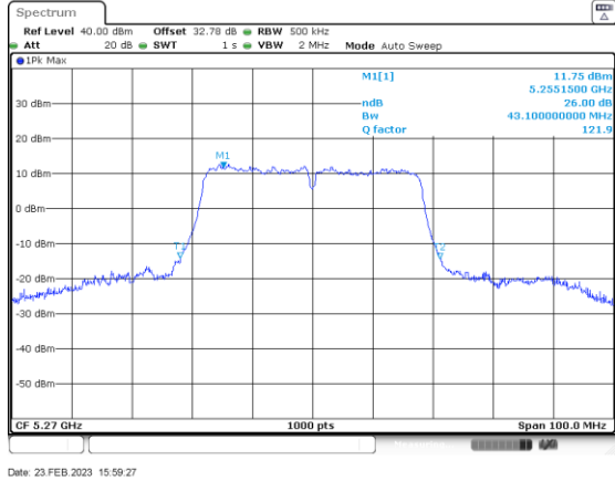
ac/n40_5270_Ant A
