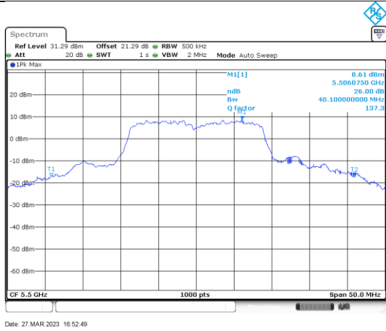
ac/n20_5500_Ant B
