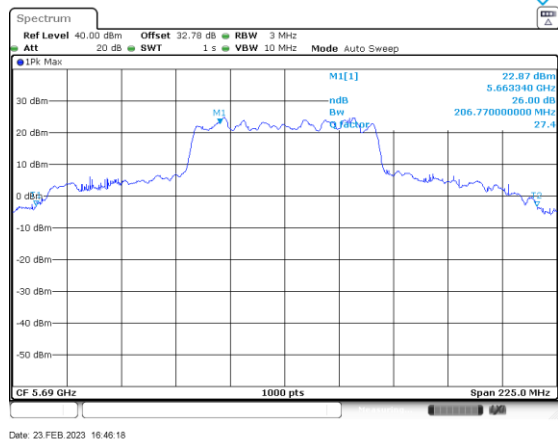
ac80_5690_Ant A
