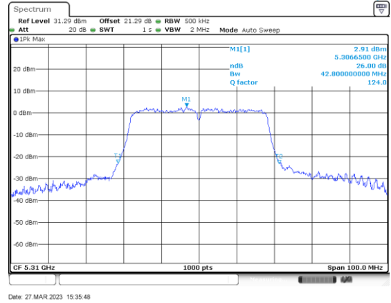
ac/n40_5310_Ant B
