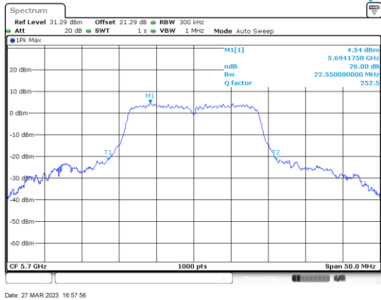
ac/n20_5700_Ant B
