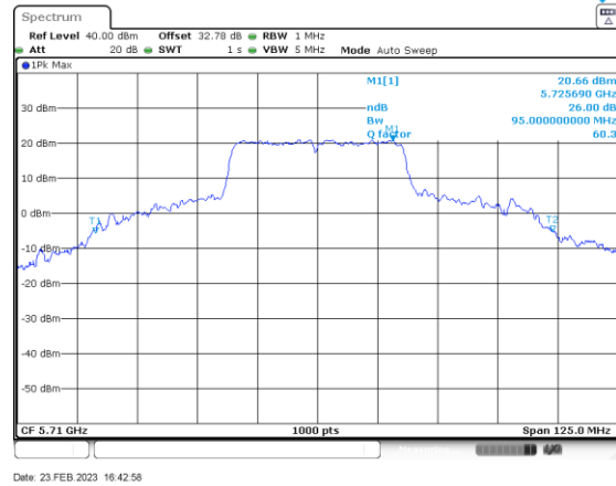
ac/n40_5710_Ant A
