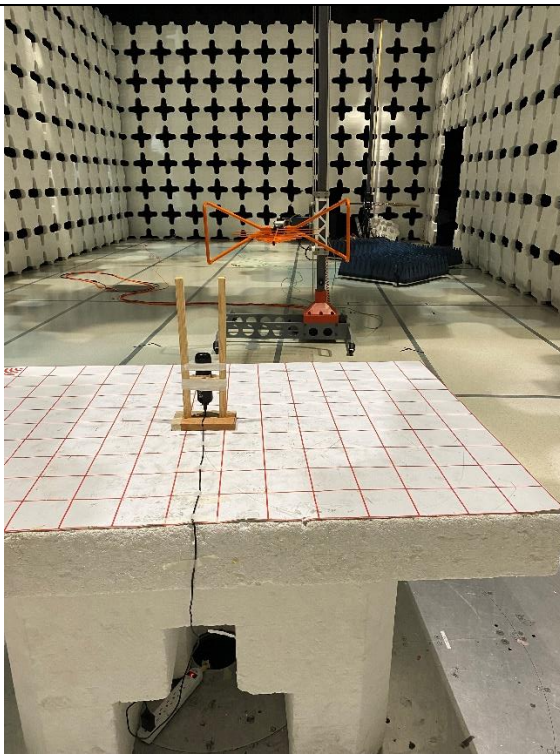
Radiated Emissions Test Below 1GHz Rear View
