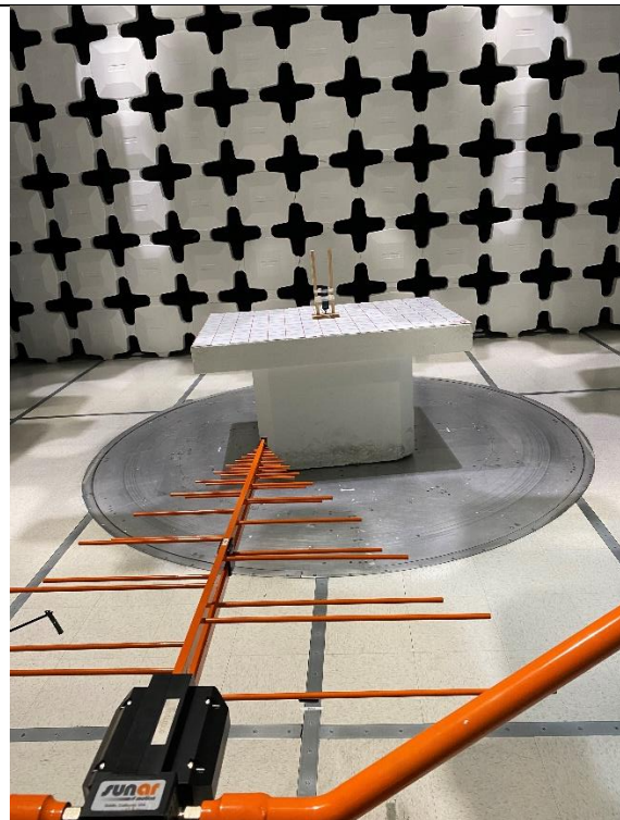
Radiated Emissions Test Below 1GHz Front View
