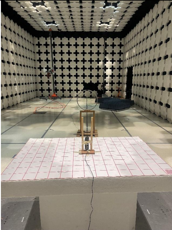
Radiated Emissions Test Below 30MHz Rear
