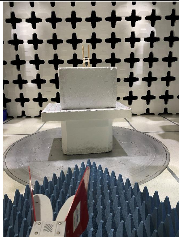
Radiated Emissions Test Above 1GHz Front View
