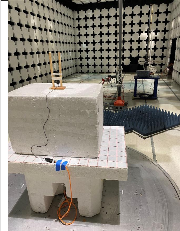
Radiated Emissions Test Above 1GHz Rear View
