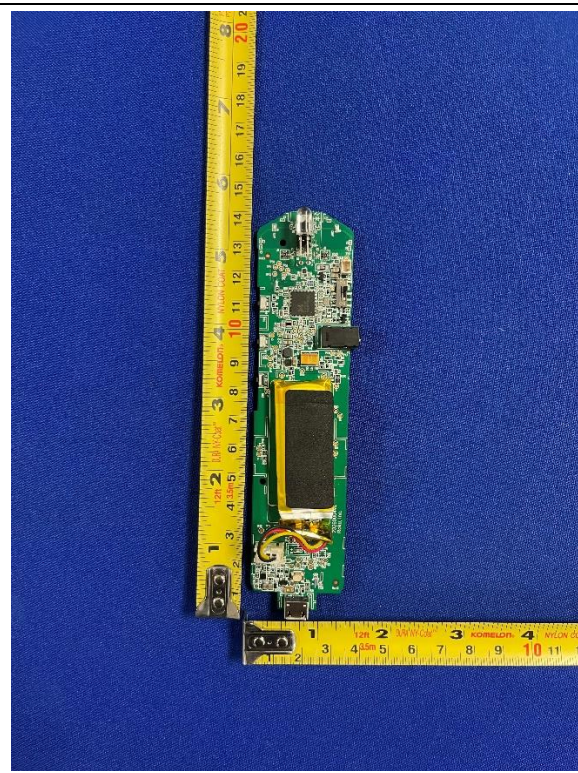
EUT – Main Board Rear
