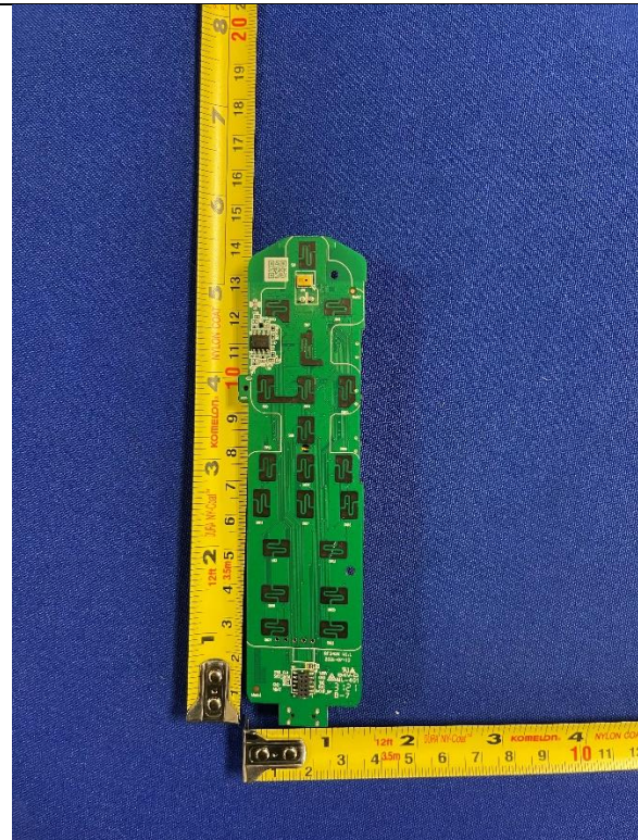
EUT – Main Board Front
