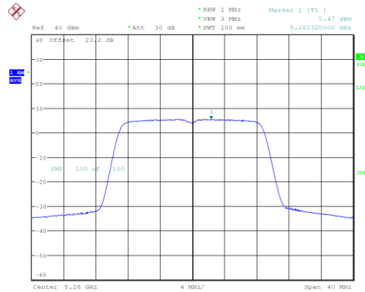
n/ac20_5260_Ant A
