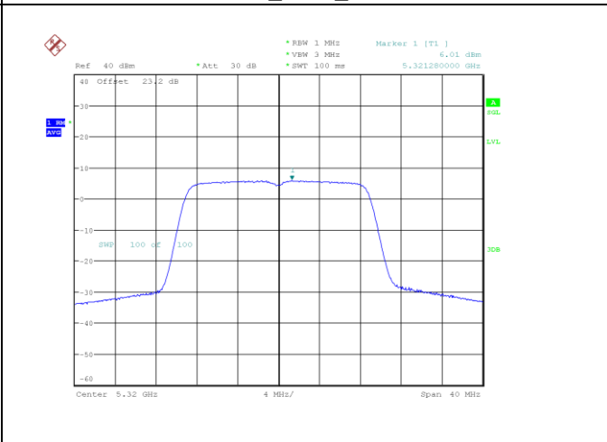
n/ac20_5320_Ant B
