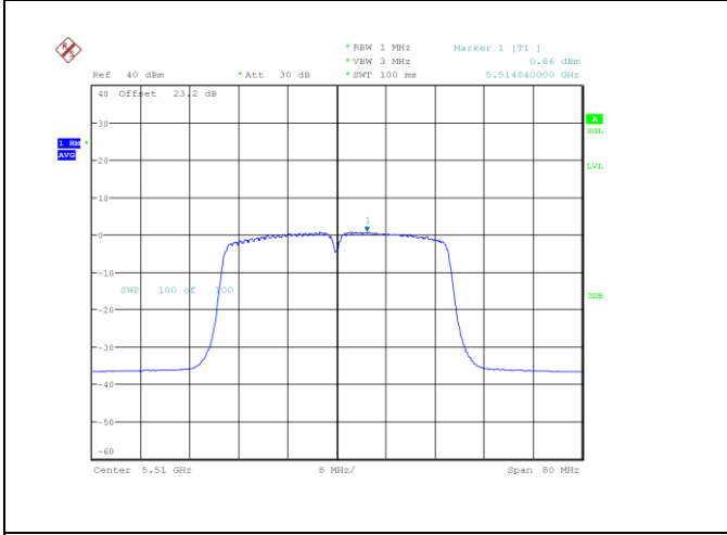
n/ac40_5510_Ant B
