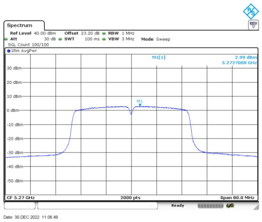
n/ac40_5270_Ant B
