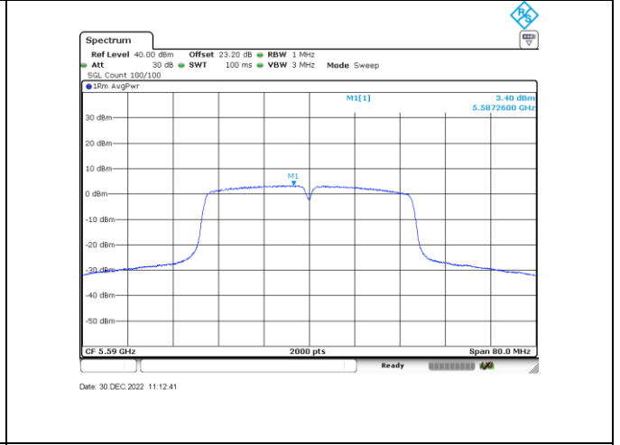
n/ac40_5590_Ant B
