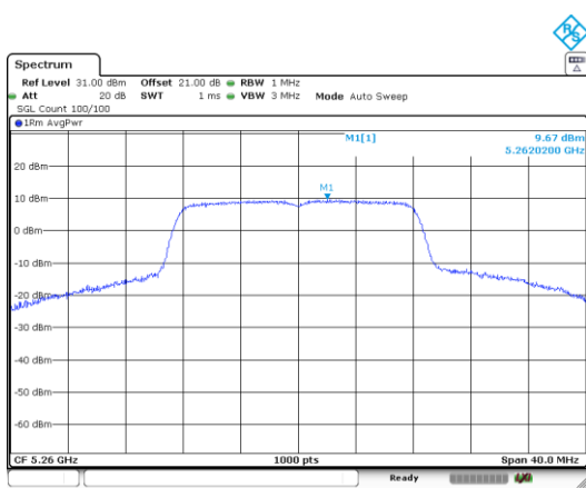
a_5260_Ant A
