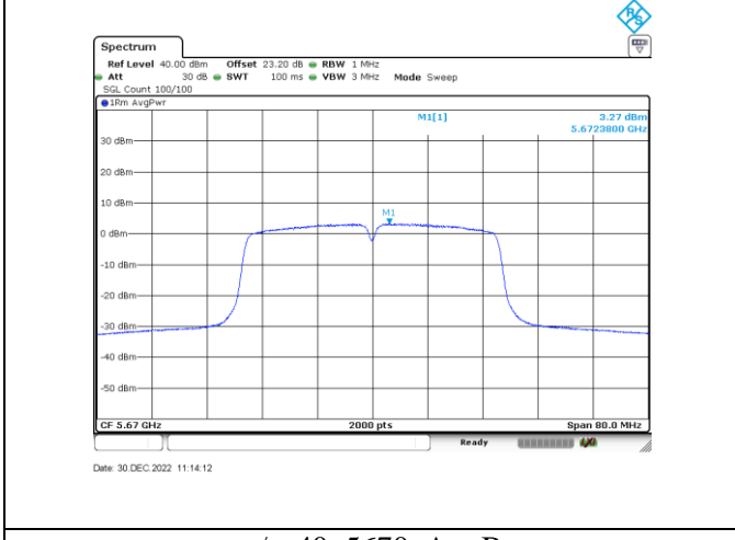
n/ac40_5670_Ant B
