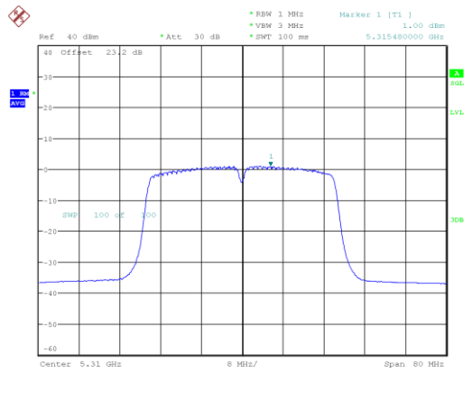
n/ac40_5310_Ant B
