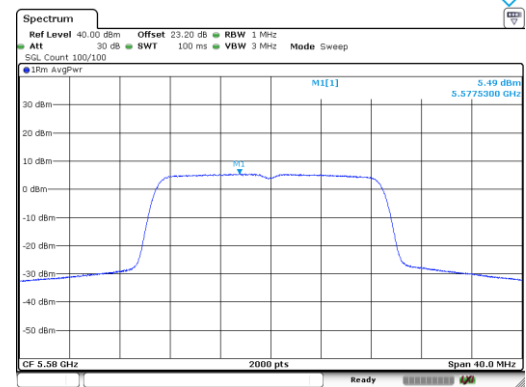
n/ac20_5580_Ant B
