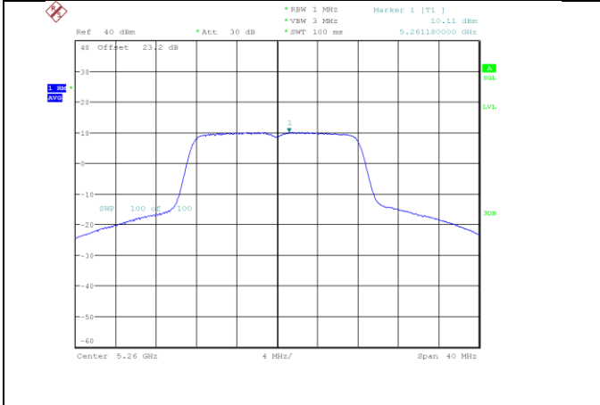
a_5260_Ant B
