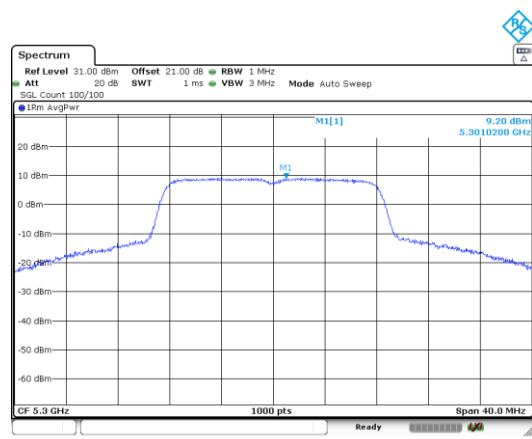
a_5300_Ant A
