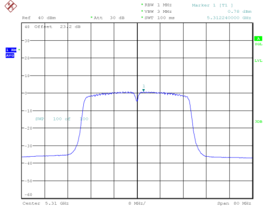
n/ac40_5310_Ant A
