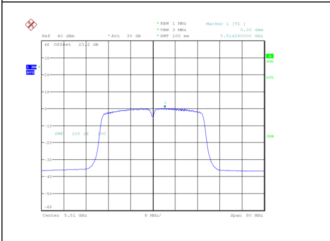
n/ac40_5510_Ant A
