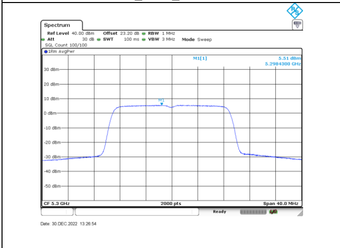
n/ac20_5300_Ant B
