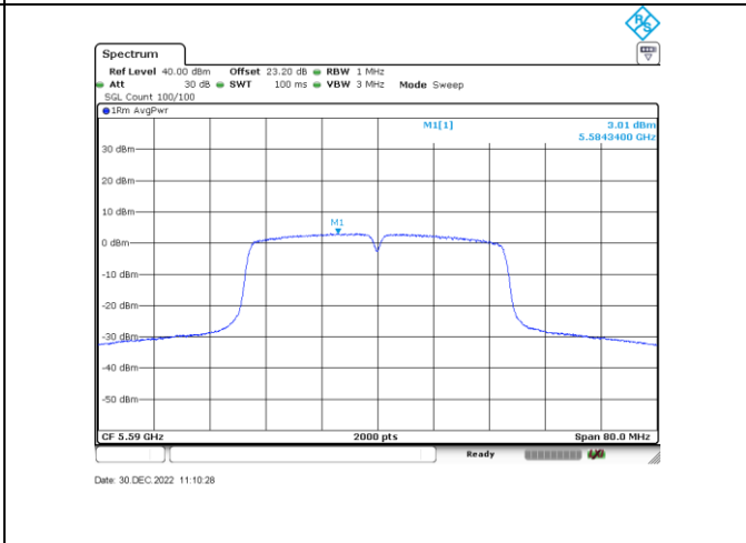
n/ac40_5590_Ant A
