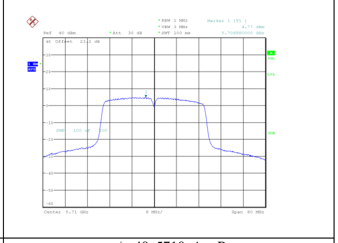
n/ac40_5710_Ant B
