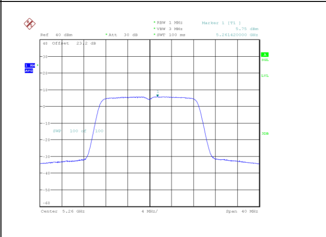
n/ac20_5260_Ant B
