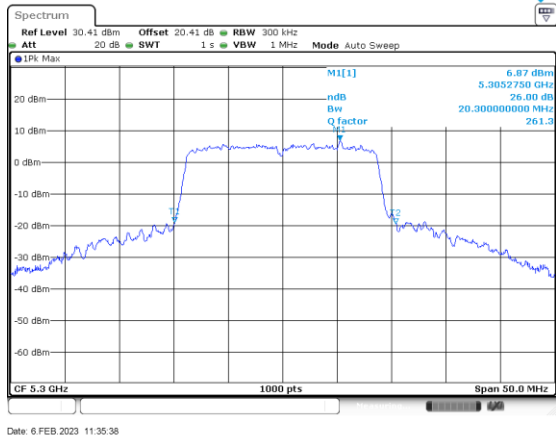
n/ac20_5300_Ant A
