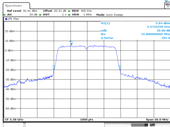
n2/ac20_5580_Ant A
