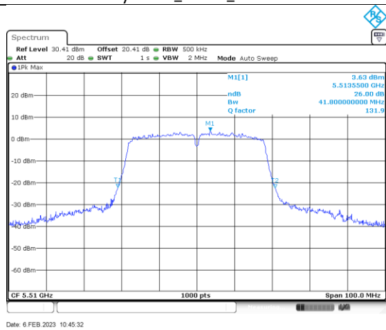
n/ac40_5510_Ant A
