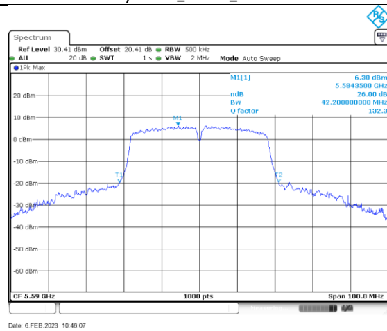
n/ac40_5590_Ant A
