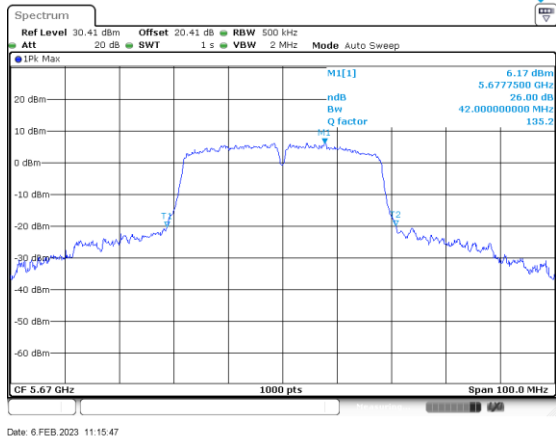
n/ac40_5670_Ant B
