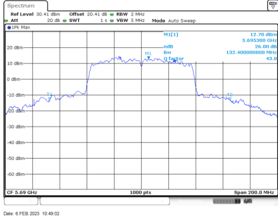
ac80_5690_Ant A
