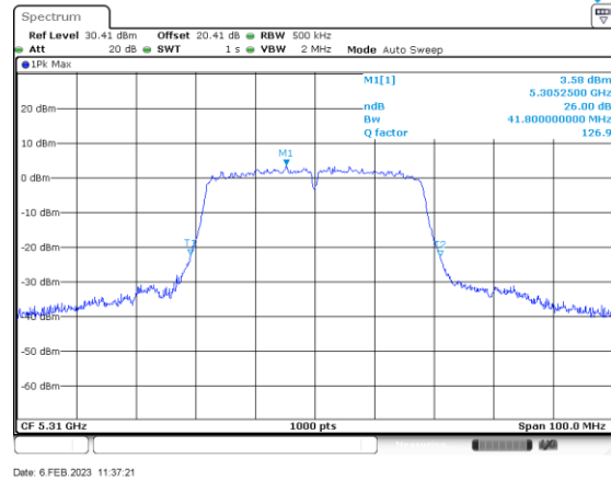
n/ac40_5310_Ant A
