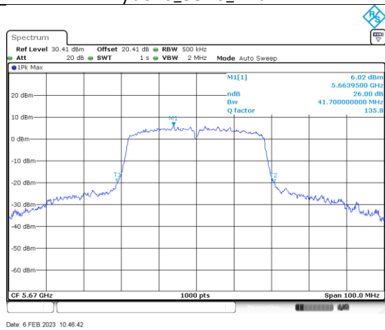
n/ac40_5670_Ant A
