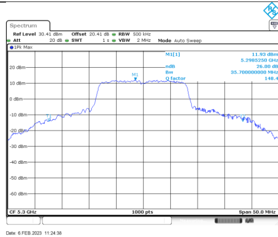
a_5300_Ant B
