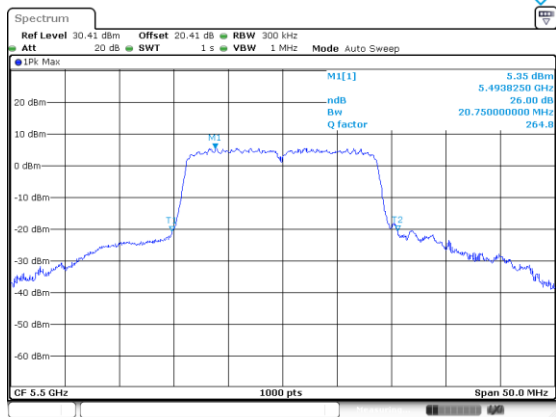
n/ac20_5500_Ant A
