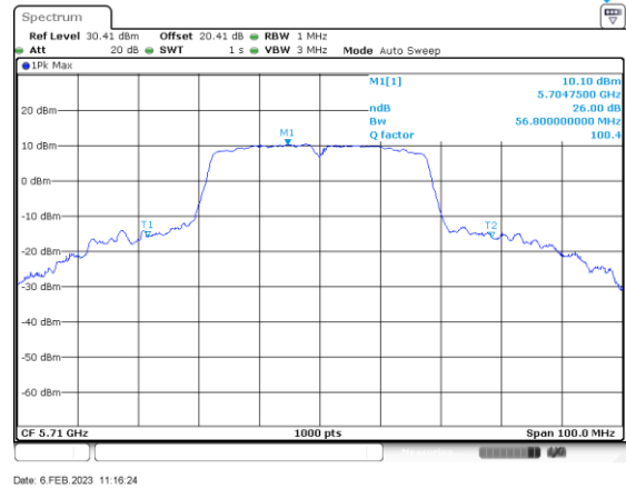
n/ac40_5710_Ant B
