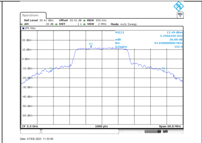
a_5300_Ant A
