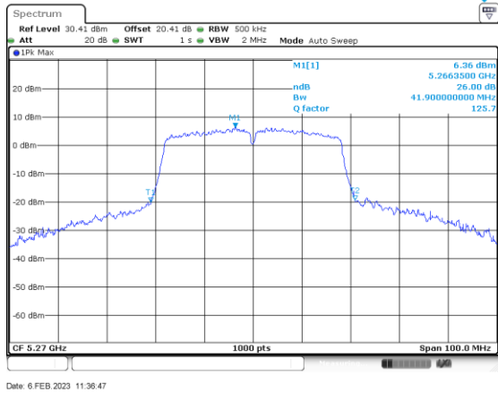
n/ac40_5270_Ant A
