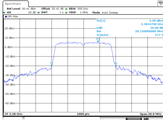
n/ac20_5580_Ant B
