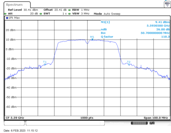
n/ac40_5590_Ant B
