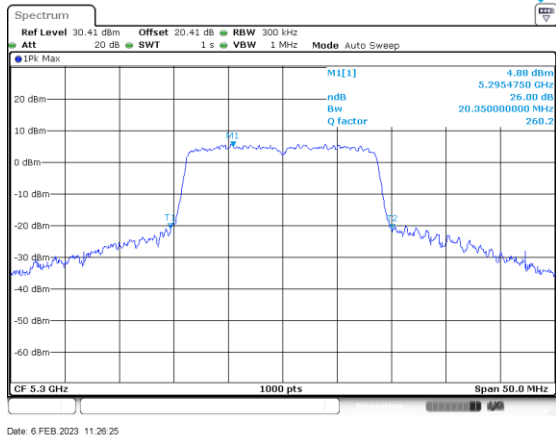
n/ac20_5300_Ant B
