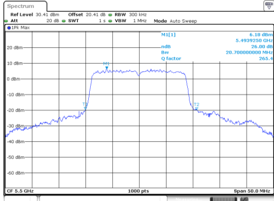
n/ac20_5500_Ant B
