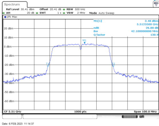
n/ac40_5510_Ant B
