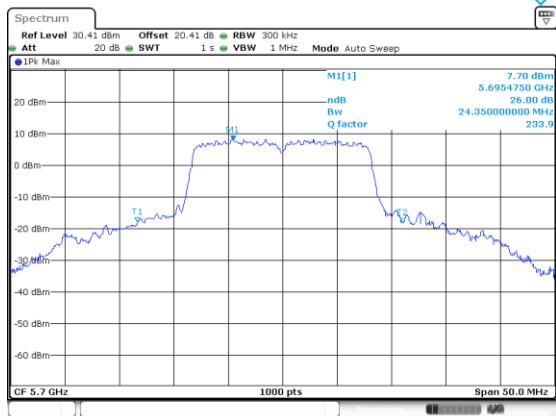
a_5700_Ant A
