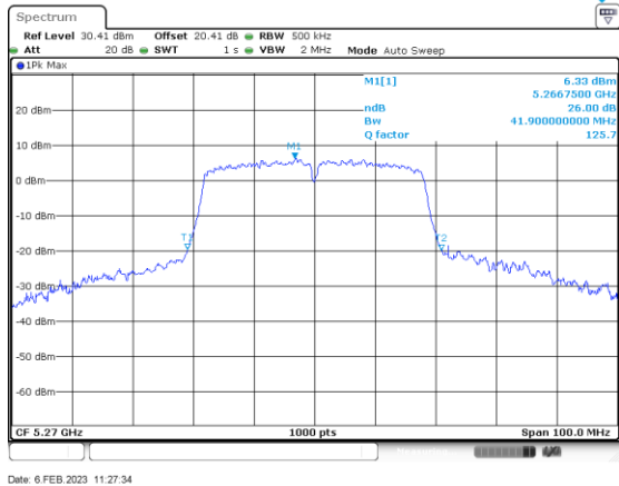
n/ac40_5270_Ant B
