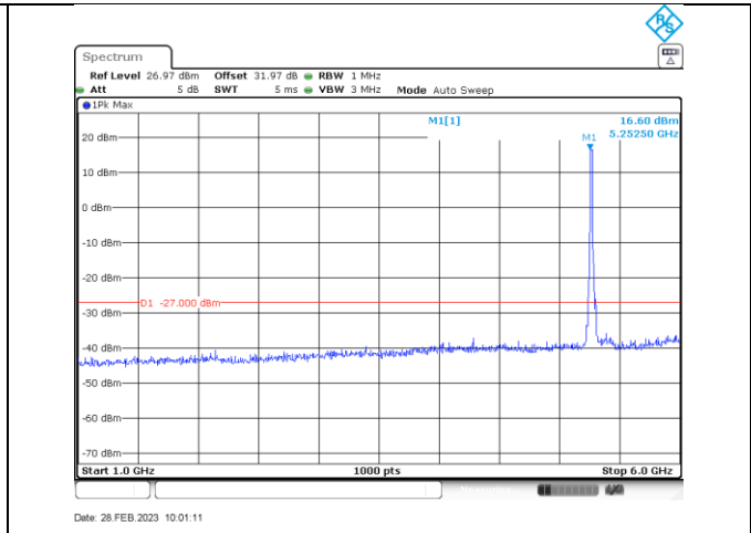
a_5260_1000-6000
