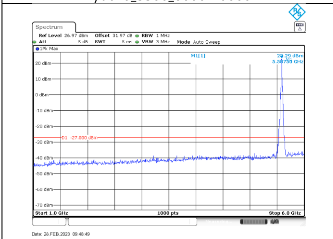
n/ac20_5580_1000-6000
