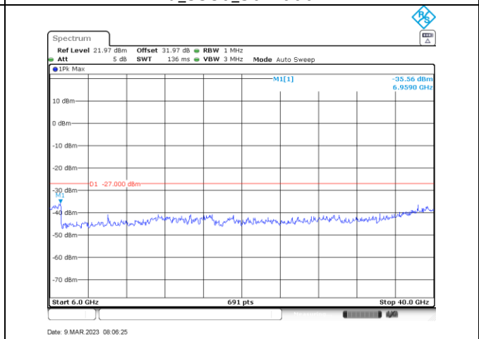
a_5580_6000-40000
