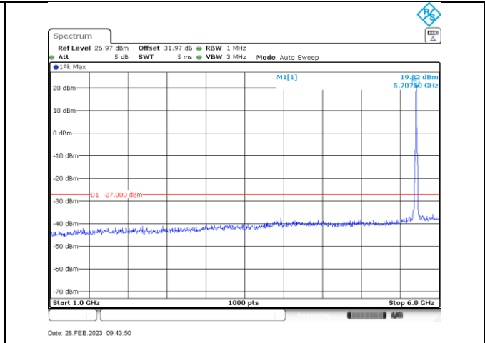
a_5700_1000-6000
