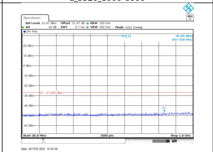
n/ac20_5260_30-1000
