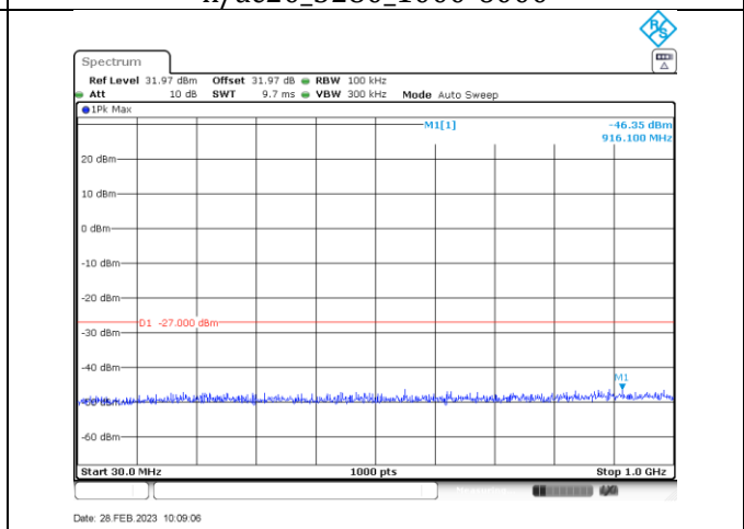
n/ac20_5320_30-1000
