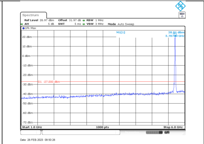
n/ac20_5700_1000-6000
