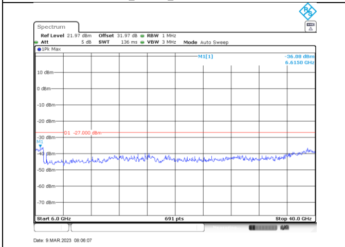
a_5500_6000-40000
