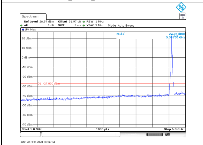
a_5580_1000-6000
