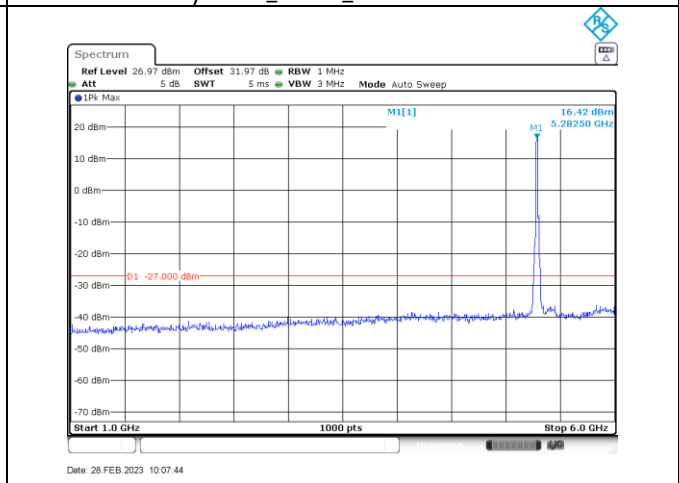
n/ac20_5280_1000-6000
