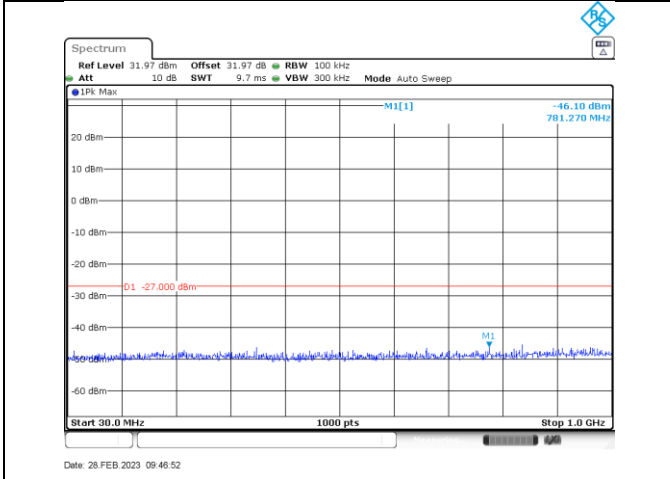
n/ac20_5500_30-1000
