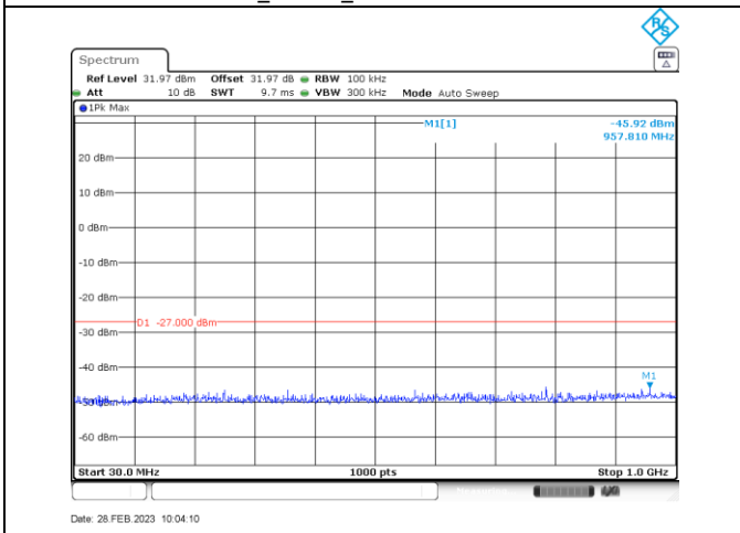
a_5320_30-1000
