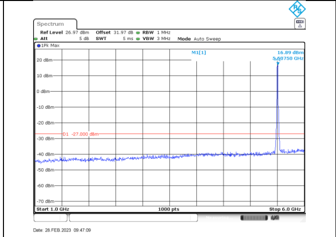
n/ac20_5500_1000-6000
