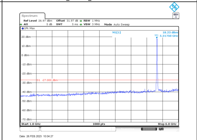
a_5320_1000-6000
