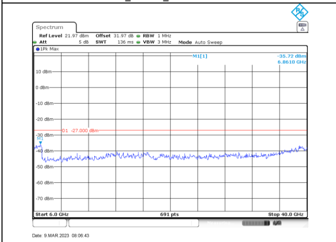
a_5700_6000-40000
