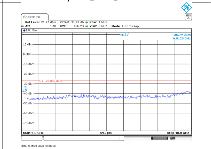
n/ac20_5580_6000-40000
