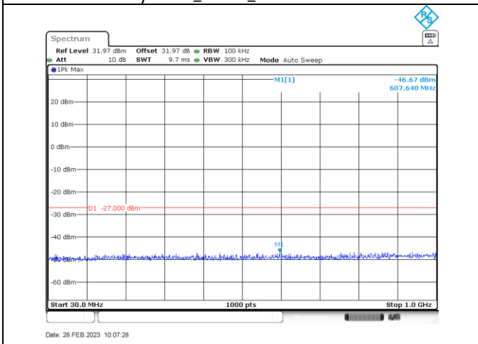
n/ac20_5280_30-1000
