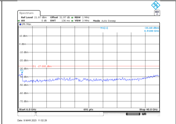
n/ac20_5260_6000-40000
