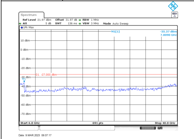
n/ac20_5500_6000-40000
