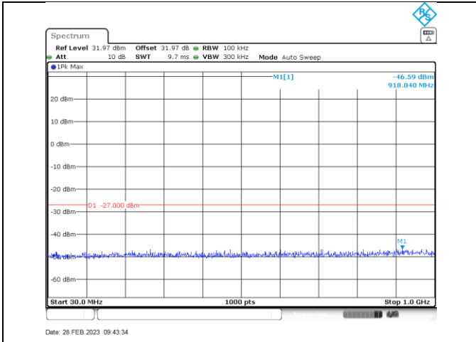
a_5700_30-1000
