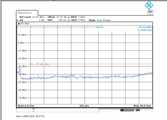
n/ac20_5700_6000-40000
