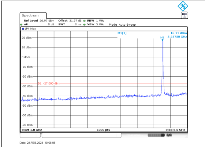
n/ac20_5260_1000-6000
