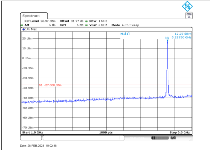
a_5280_1000-6000
