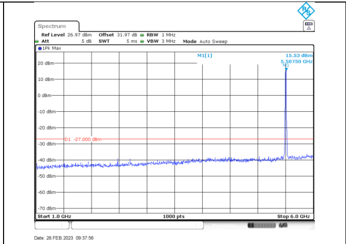
a_5500_1000-6000
