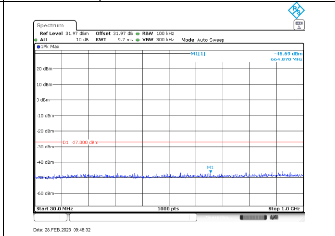
n/ac20_5580_30-1000
