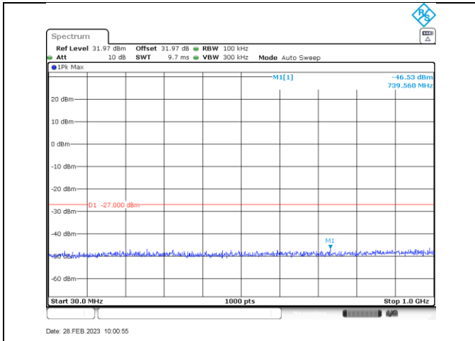
a_5260_30-1000
