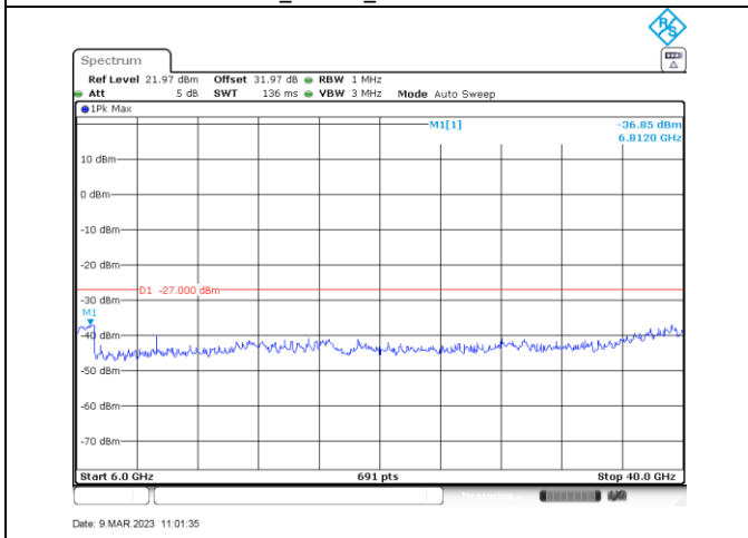
a_5260_6000-40000
