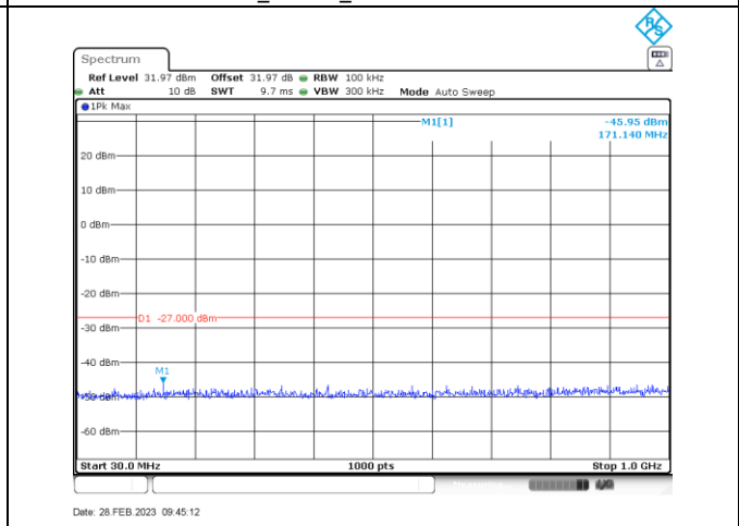
a_5720_30-1000
